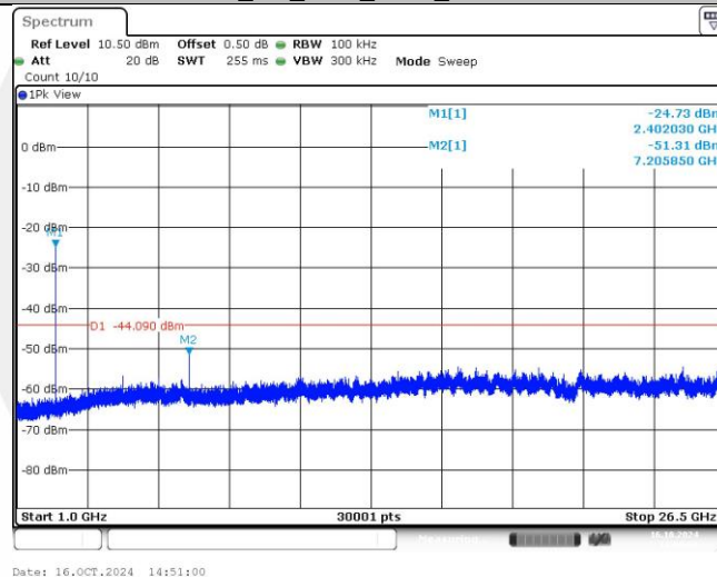
BLE_1M_Ant1_2402_1000~26500
