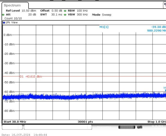
BLE_1M_Ant1_2440_30~1000
