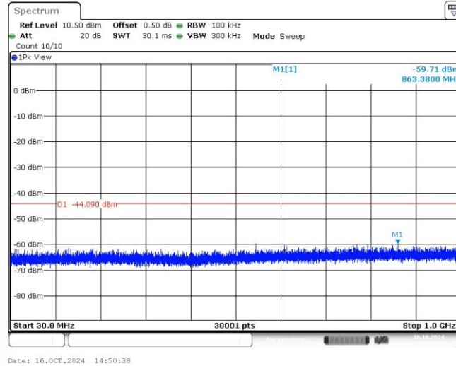
BLE_1M_Ant1_2402_30~1000
