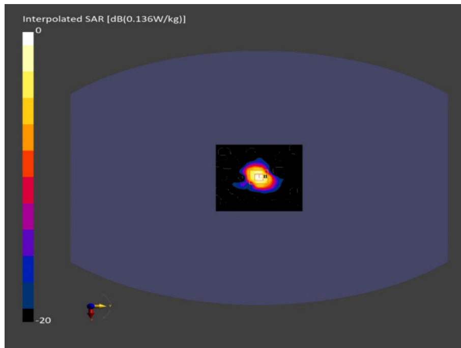
Figure C.1: Testing results for the Nuki Smart Lock at Channel 1 (2412 MHz, 1Mbps)
