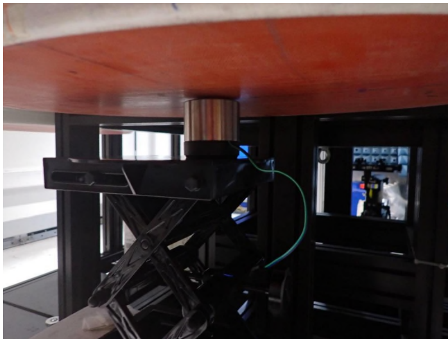
Figure D.2: EUT setup in 0mm front position.
