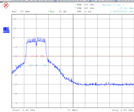
Out Of Band Emission IEEE 802.11n_Channel 11_20MHz_Antenna 0
