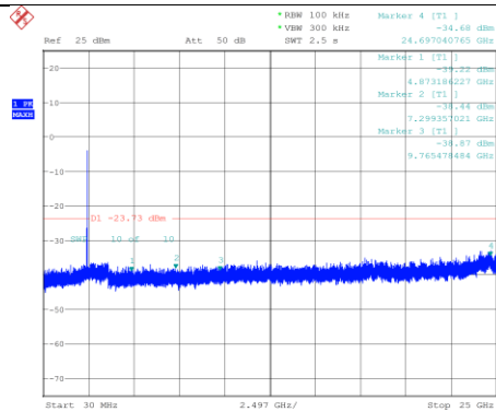
30.0 MHz - 25000.0 MHz IEEE 802.11n_Channel 6_20MHz_Antenna 0
