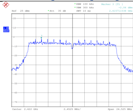
In-Band Reference Level IEEE 802.11n_Channel 3_40MHz_Antenna 0
