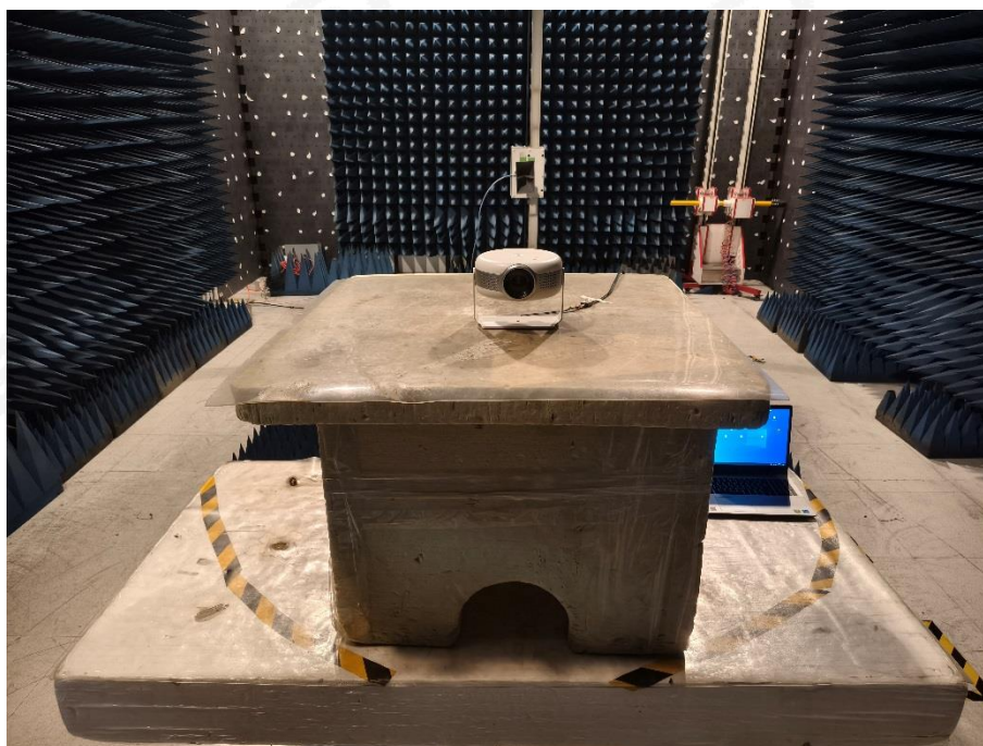
DSS_DTS_ U-NII radiation H
