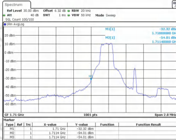
Band4 QAM16 BW=1.4MHz Channel=19957 RB Size=1 Position=#0 NVNT
