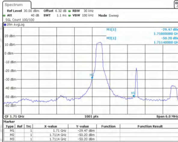
Band4 QAM16 BW=3MHz Channel=19965 RB Size=1 Position=#0 NVNT
