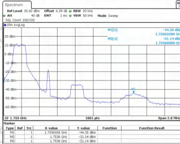
Band4 QAM16 BW=1.4MHz Channel=20393 RB Size=1 Position=#0 NVNT
