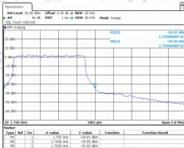
Band4 QAM16 BW=1.4MHz Channel=20393 RB Size=6 Position=#0 NVNT
