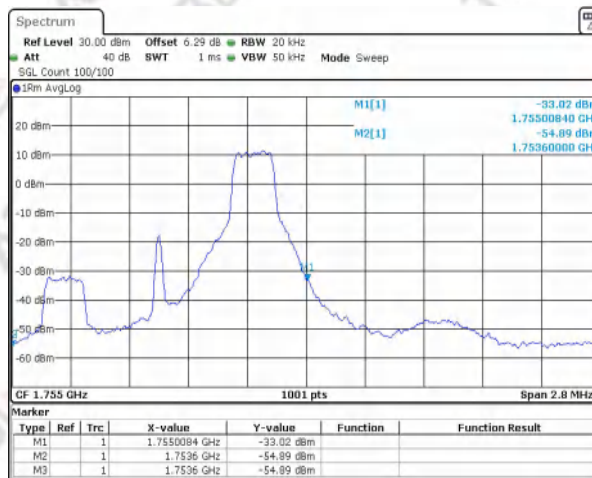
Band4 QAM16 BW=1.4MHz Channel=20393 RB Size=1 Position=#Max NVNT
