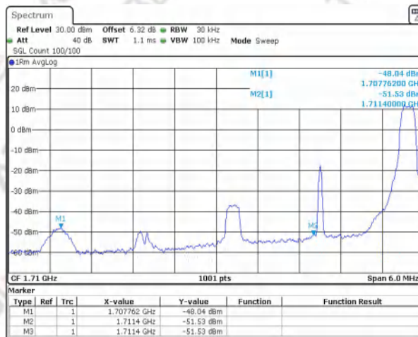
Band4 QAM16 BW=3MHz Channel=19965 RB Size=1 Position=#Max NVNT
