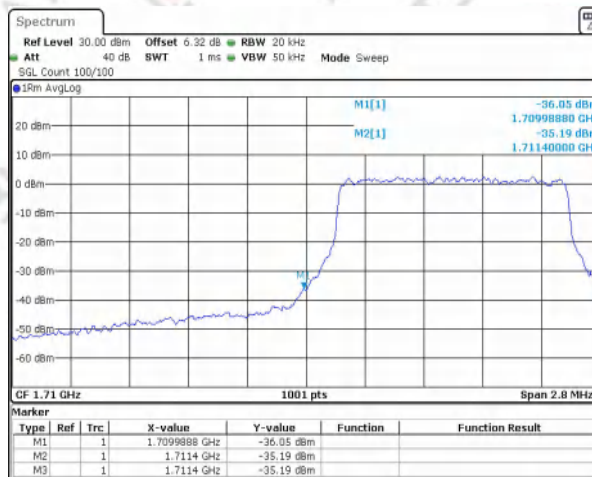
Band4 QAM16 BW=1.4MHz Channel=19957 RB Size=6 Position=#0 NVNT
