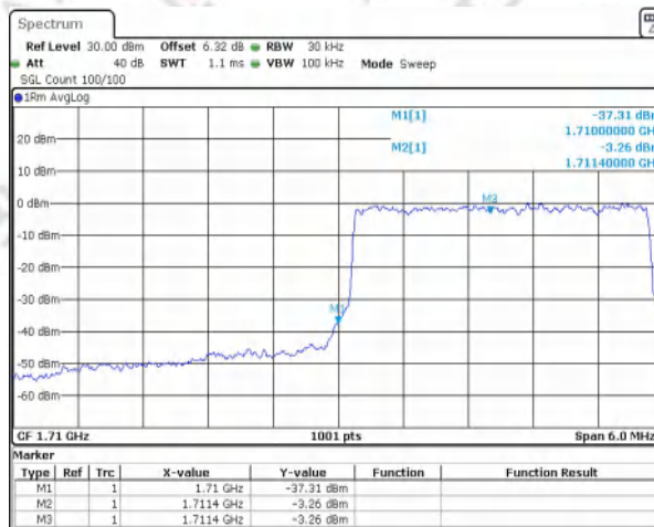
Band4 QAM16 BW=3MHz Channel=19965 RB Size=15 Position=#0 NVNT
