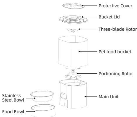
Pet feeder
