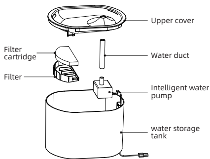
Water Fountain
