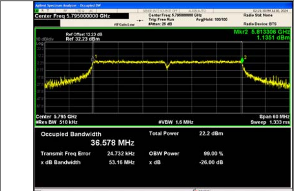
IEEE 802.11n_Channel 159_40MHz_Antenna 0
