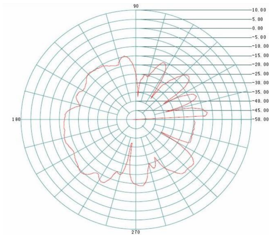
Vertical 2402M
