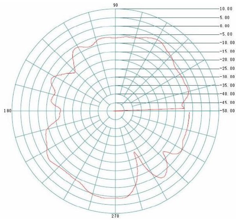
Vertical 2440M
