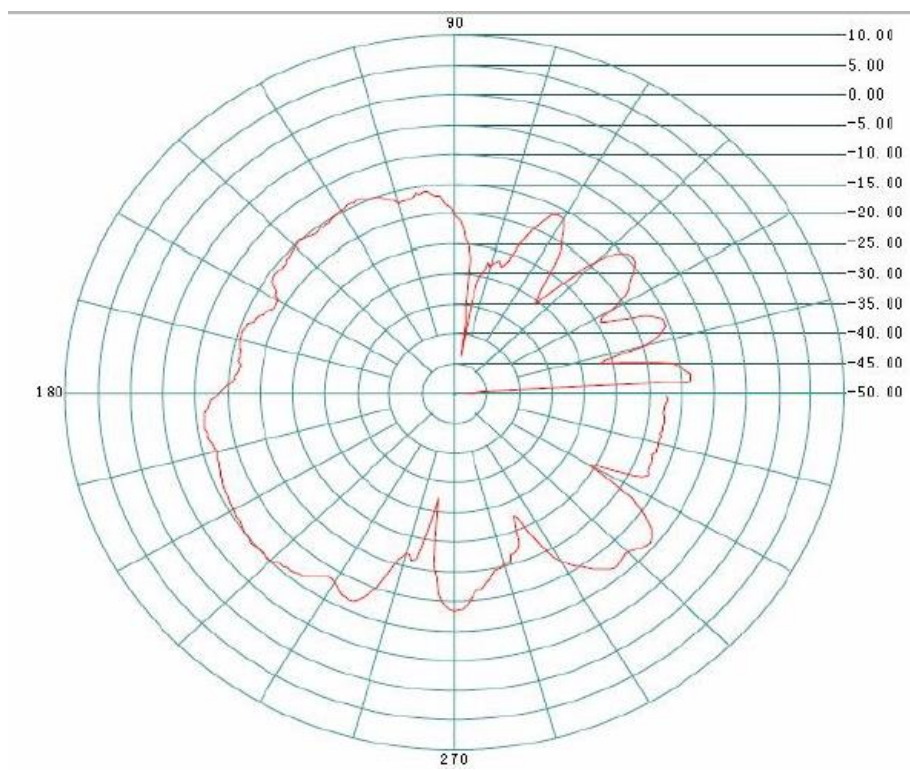
Horizontal 2440M
