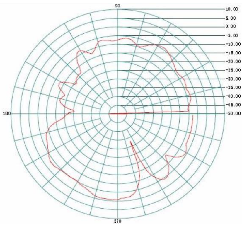
Horizontal 2480M
