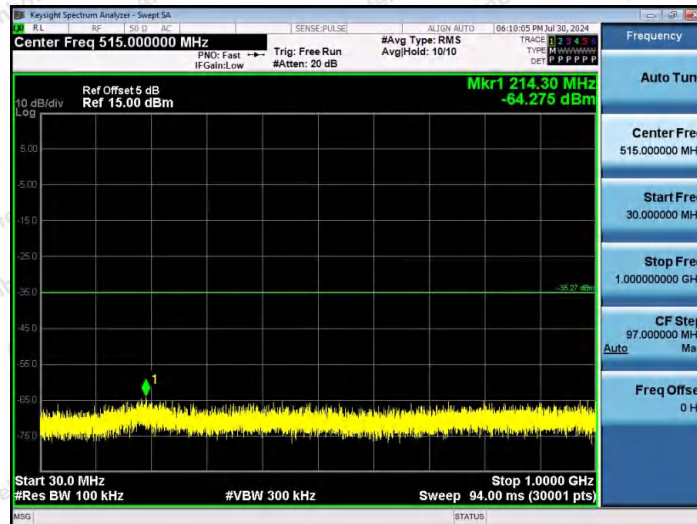
11N40MIMO-Ant2-2437-30~1000-PASS
