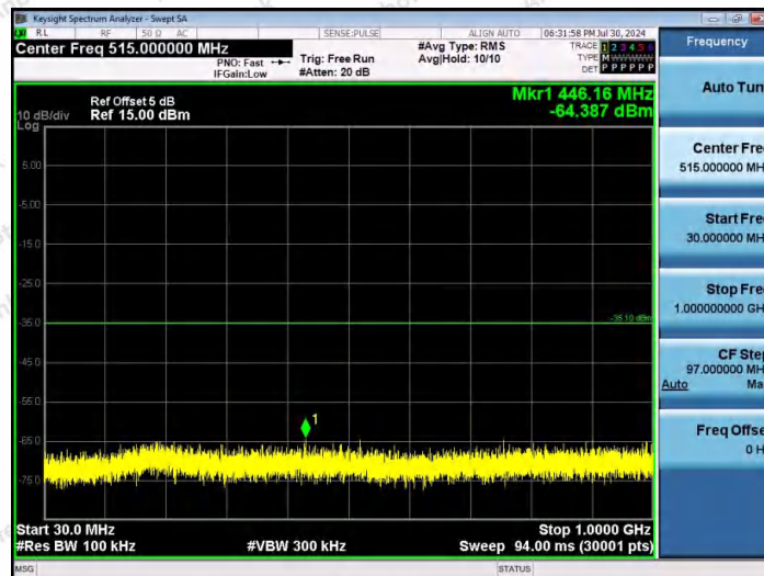
11AX40MIMO-Ant1-2437-30~1000-PASS
