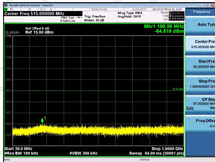
11AX40MIMO-Ant2-2452-30~1000-PASS
