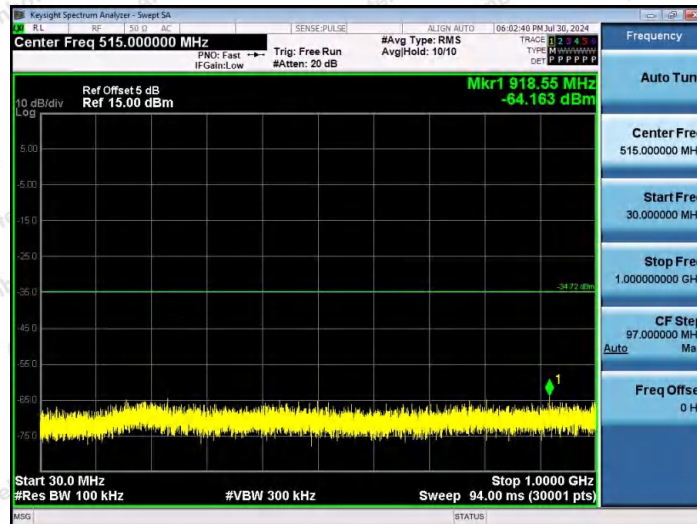
11N20MIMO-Ant2-2462-30~1000-PASS
