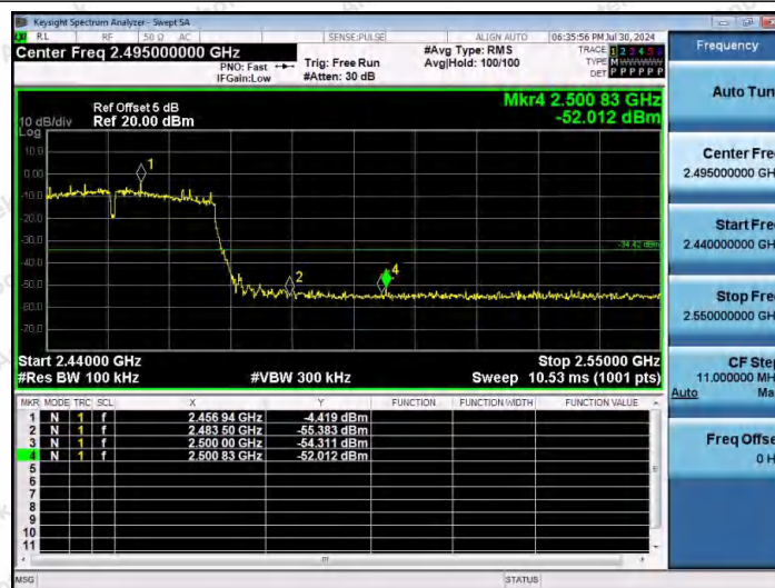
11AX40MIMO-Ant1-2452-PASS
