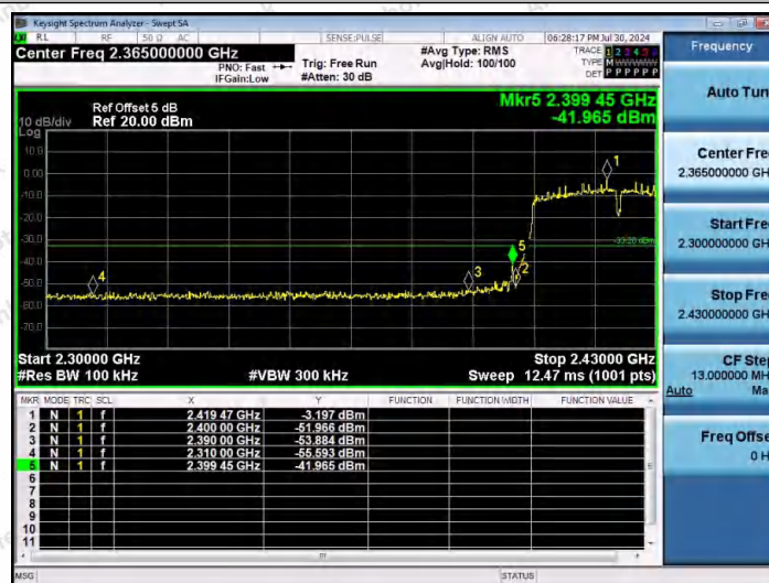
11AX40MIMO-Ant1-2422-PASS
