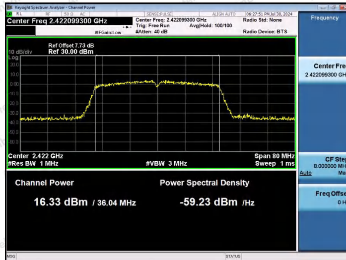
11AX40MIMO-Ant1-2422-PASS
