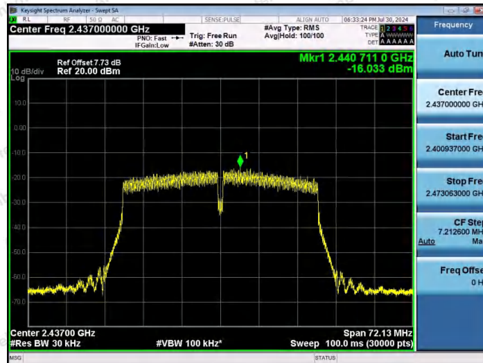
11AX40MIMO-Ant2-2437-PASS
