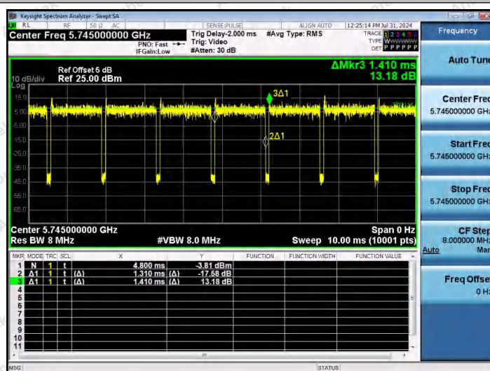
NTNV-11N20MIMO-Ant2-5745
