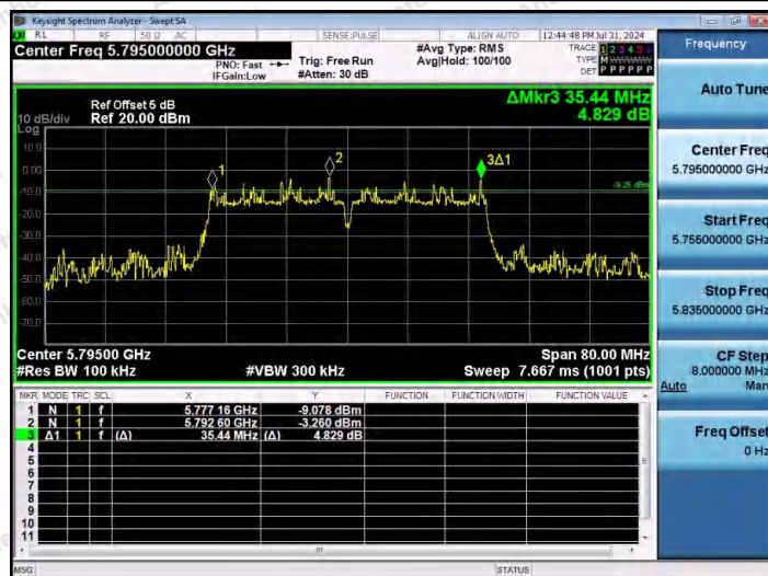
11N40MIMO-Ant2-5795-PASS
