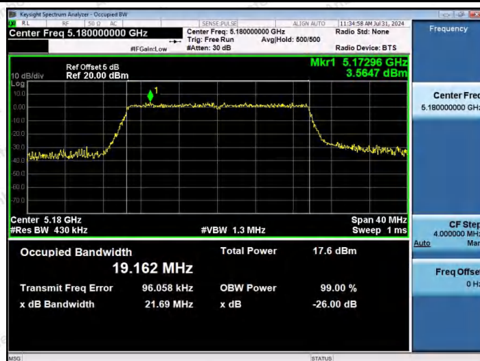
11AX20MIMO-Ant2-5180
