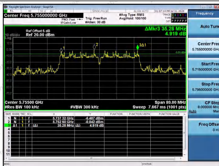
11AC40MIMO-Ant2-5755-PASS
