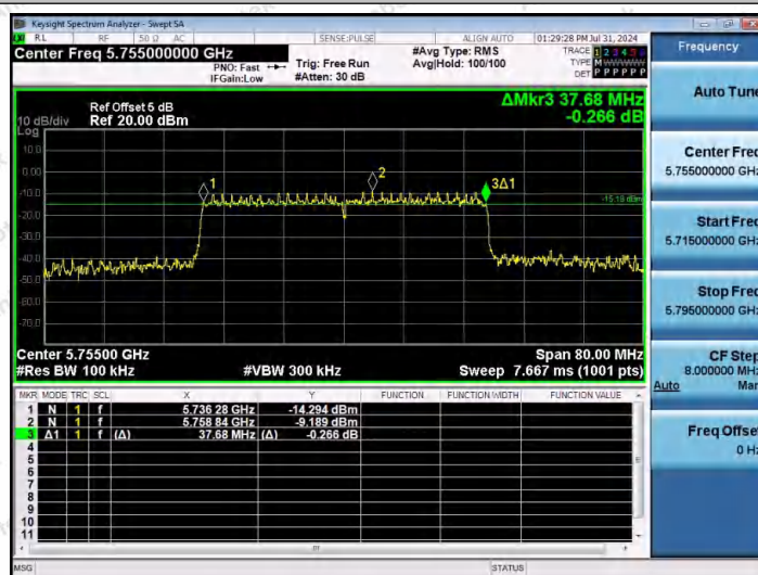
11AX40MIMO-Ant2-5755-PASS
