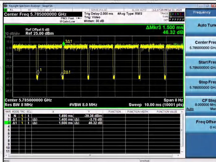
NTNV-11A-Ant2-5785
