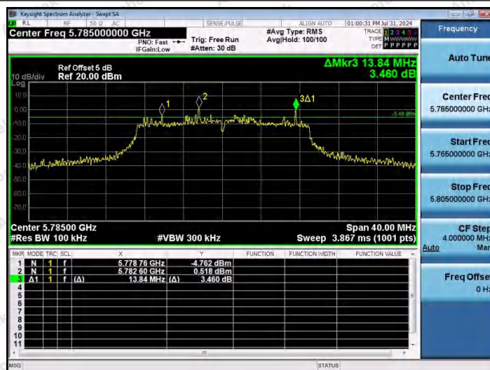
11AC20MIMO-Ant2-5785-PASS
