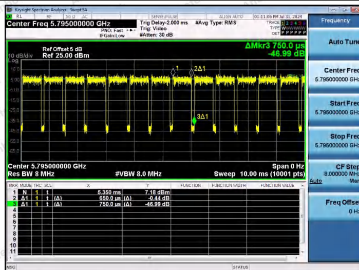
NTNV-11AC40MIMO-Ant2-5795
