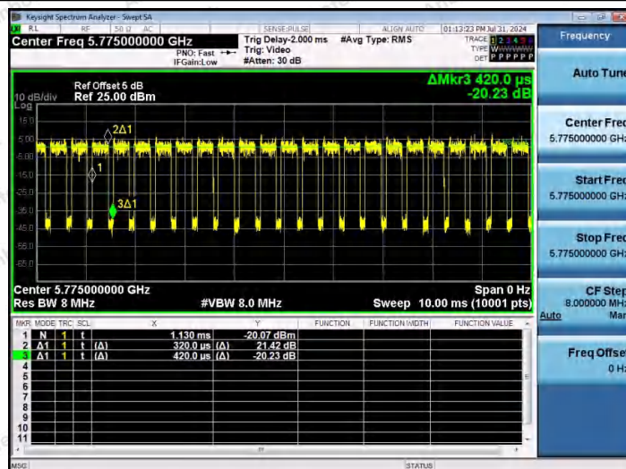
NTNV-11AC80MIMO-Ant1-5775
