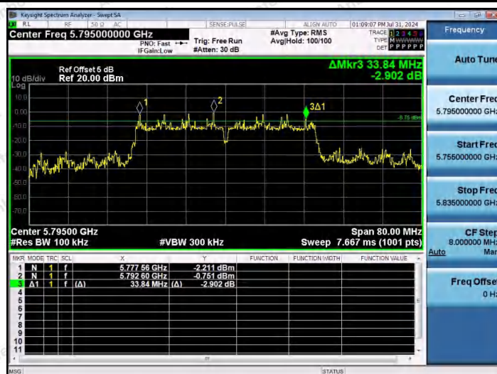
11AC40MIMO-Ant1-5795-PASS
