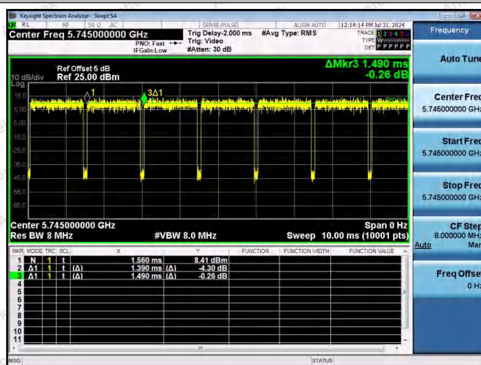
NTNV-11A-Ant2-5745
