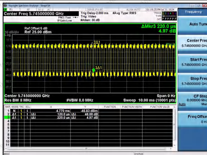
NTNV-11AX20MIMO-Ant2-5745
