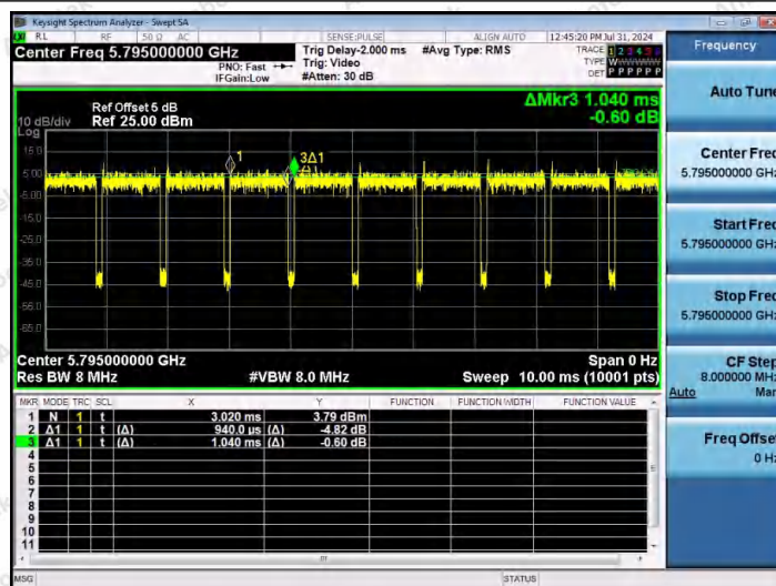
NTNV-11N40MIMO-Ant2-5795
