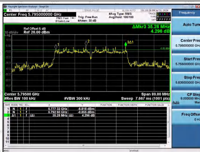
11AC40MIMO-Ant2-5795-PASS
