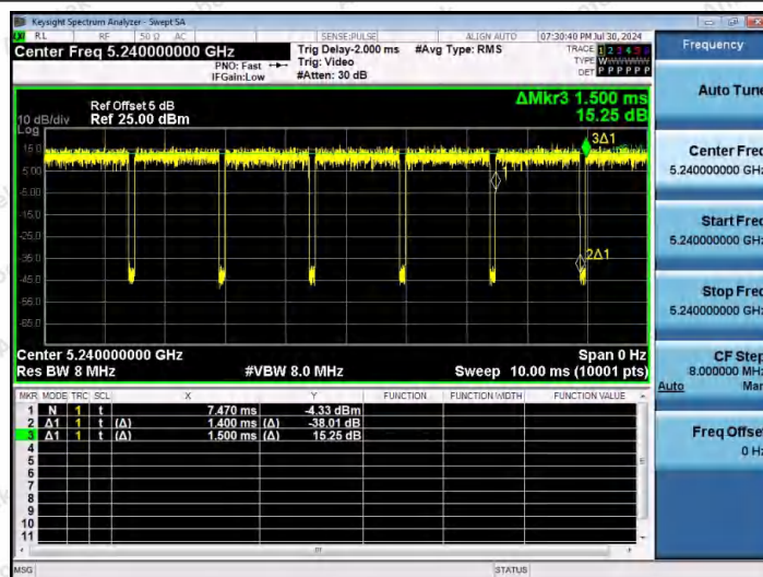
NTNV-11A-Ant1-5240
