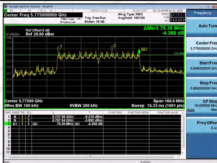
11AC80MIMO-Ant2-5775-PASS
