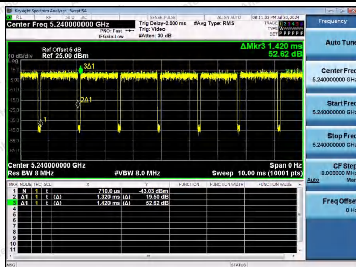
NTNV-11AC20MIMO-Ant1-5240
