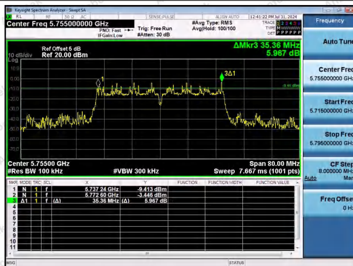
11N40MIMO-Ant2-5755-PASS
