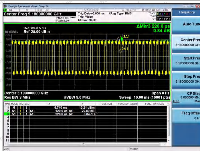
NTNV-11AX20MIMO-Ant1-5180
