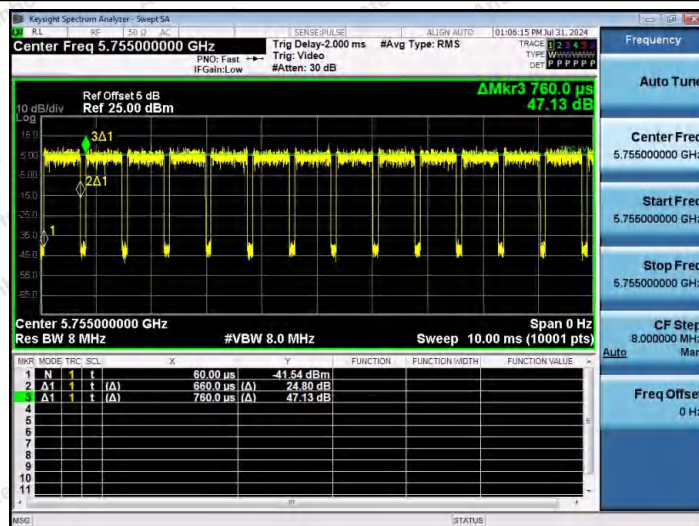
NTNV-11AC40MIMO-Ant1-5755
