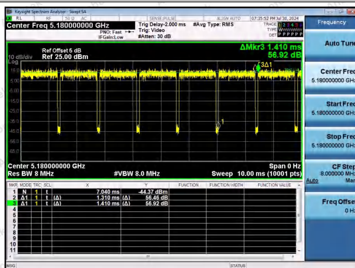
NTNV-11N20MIMO-Ant2-5180
