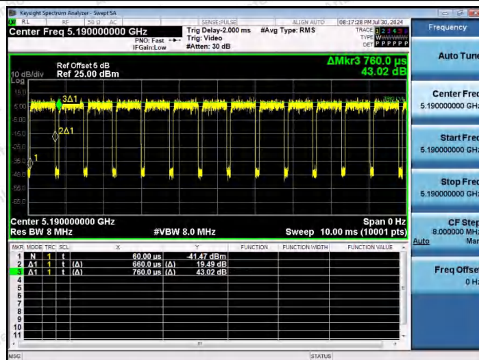
NTNV-11AC40MIMO-Ant2-5190
