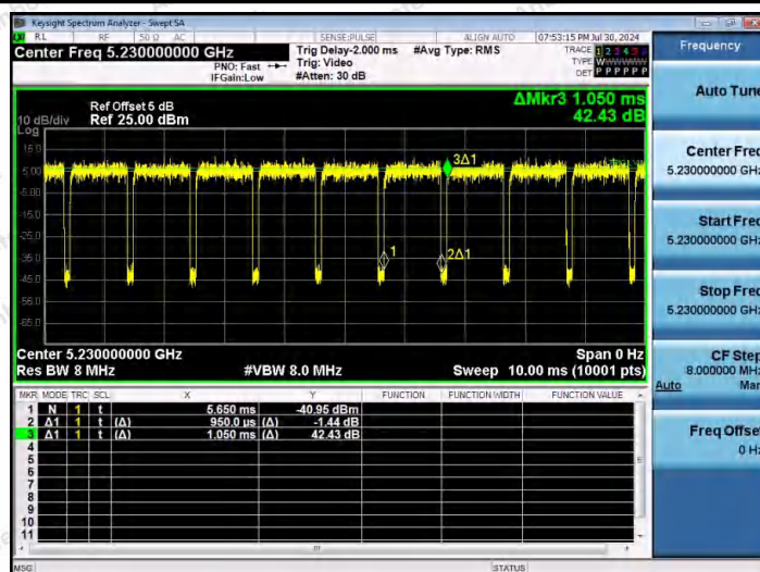
NTNV-11N40MIMO-Ant2-5230
