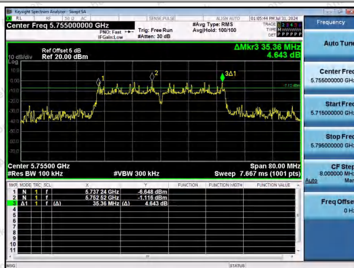
11AC40MIMO-Ant1-5755-PASS
