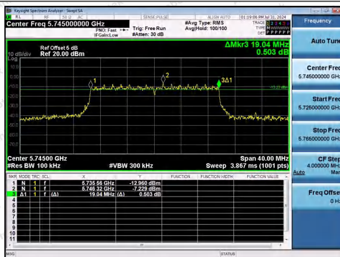
11AX20MIMO-Ant2-5745-PASS
