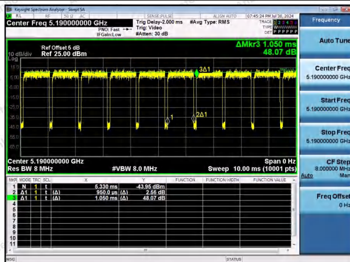
NTVN-11N40MIMO-Ant1-5190
