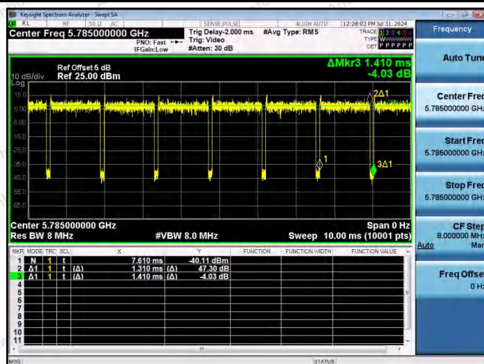
NTNV-11N20MIMO-Ant2-5785
