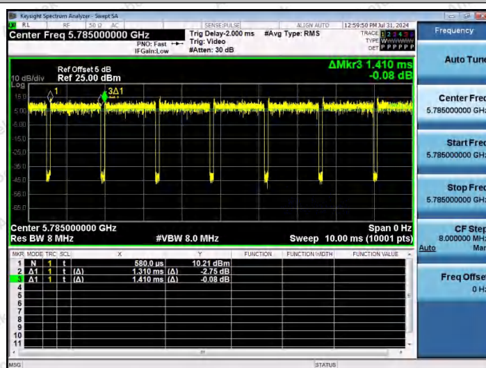
NTNV-11AC20MIMO-Ant1-5785
