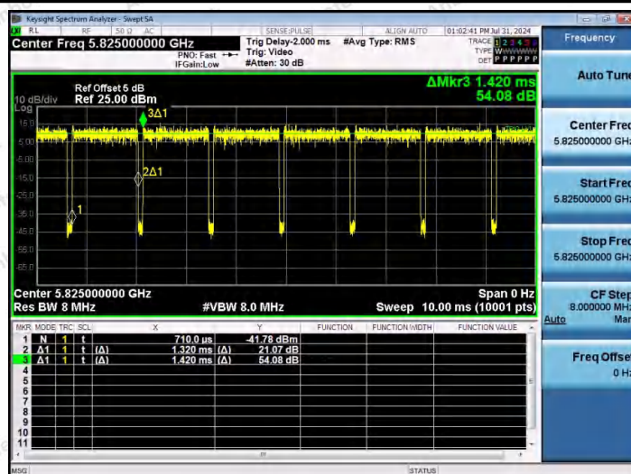
NTNV-11AC20MIMO-Ant1-5825
