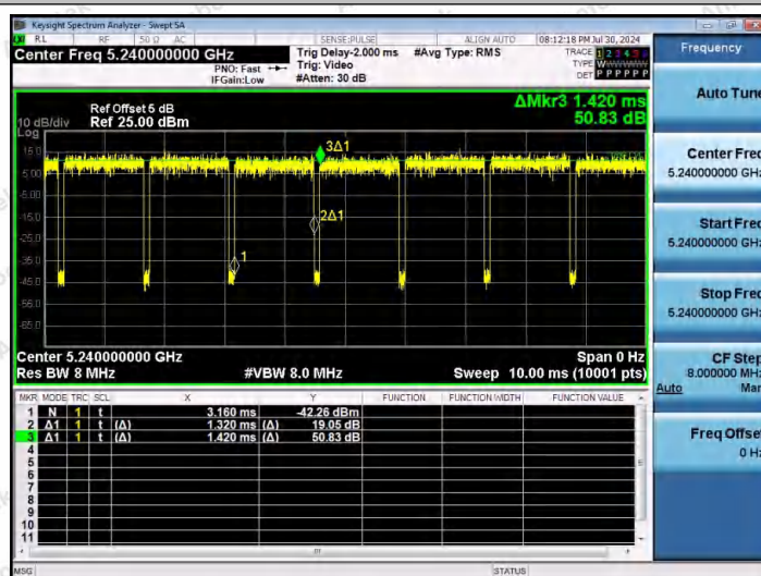
NTNV-11AC20MIMO-Ant2-5240
