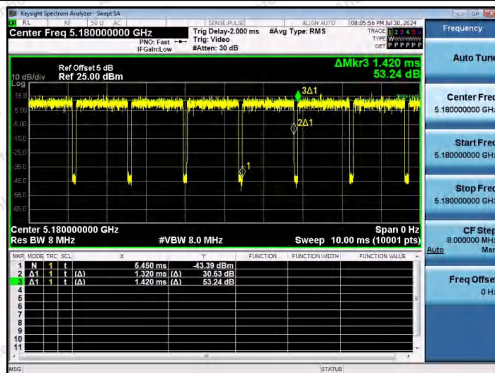
NTNV-11AC20MIMO-Ant2-5180
