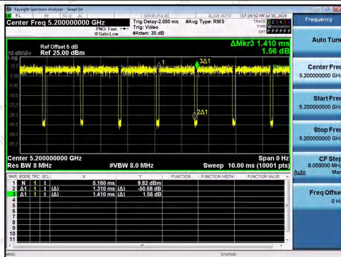
NTVN-11N20MIMO-Ant2-5200
