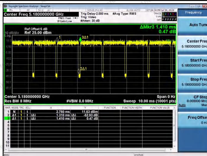
NTNV-11N20MIMO-Ant1-5180
