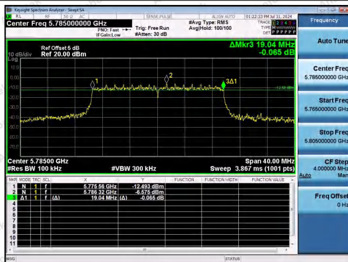
11AX20MIMO-Ant2-5785-PASS
