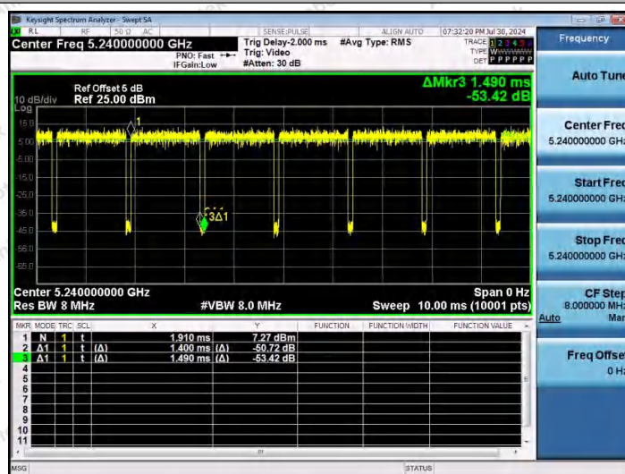
NTNV-11A-Ant2-5240
