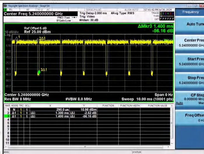
NTVN-11N20MIMO-Ant1-5240
