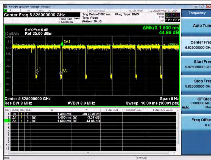
NTNV-11A-Ant2-5825
