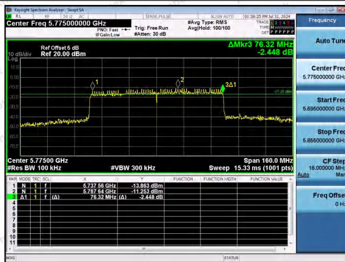
11AX80MIMO-Ant1-5775-PASS
