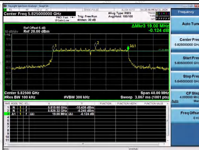
11AX20MIMO-Ant2-5825-PASS
