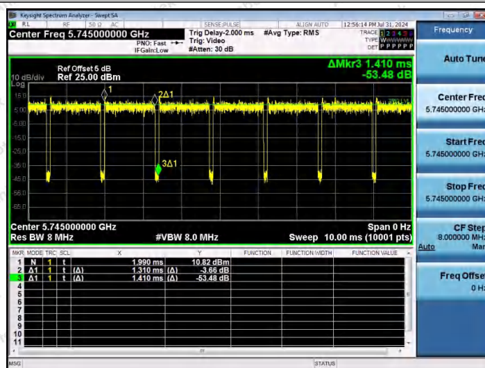
NTNV-11AC20MIMO-Ant1-5745
