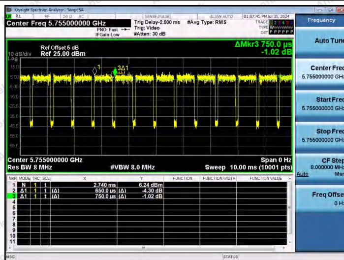
NTNV-11AC40MIMO-Ant2-5755
