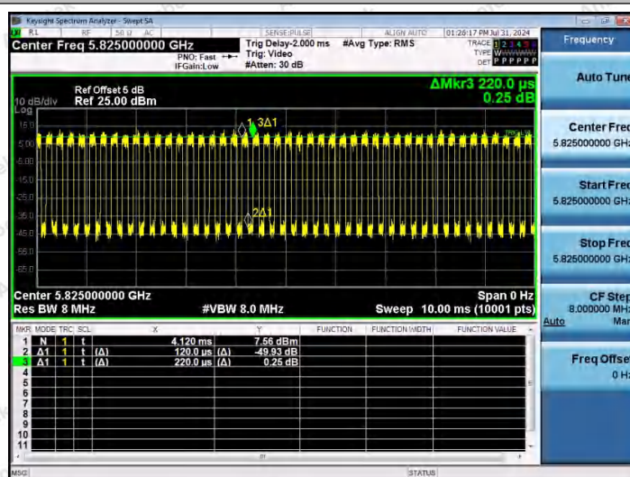
NTNV-11AX20MIMO-Ant2-5825
