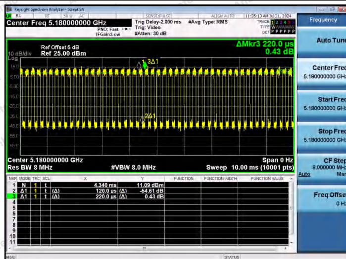
NTNV-11AX20MIMO-Ant2-5180
