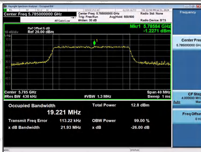
11AX20MIMO-Ant2-5785
