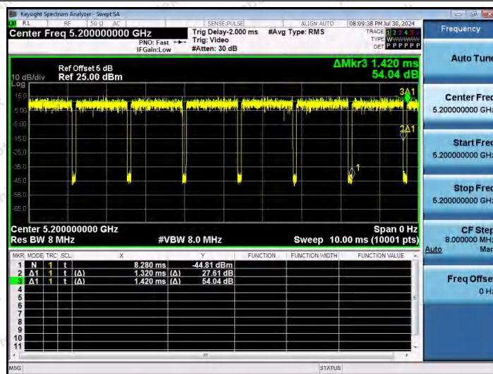
NTNV-11AC20MIMO-Ant2-5200
