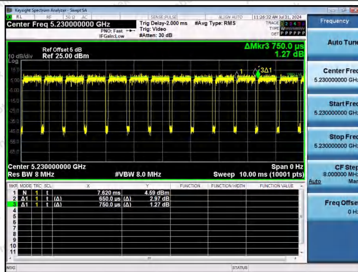
NTNV-11AC40MIMO-Ant2-5230
