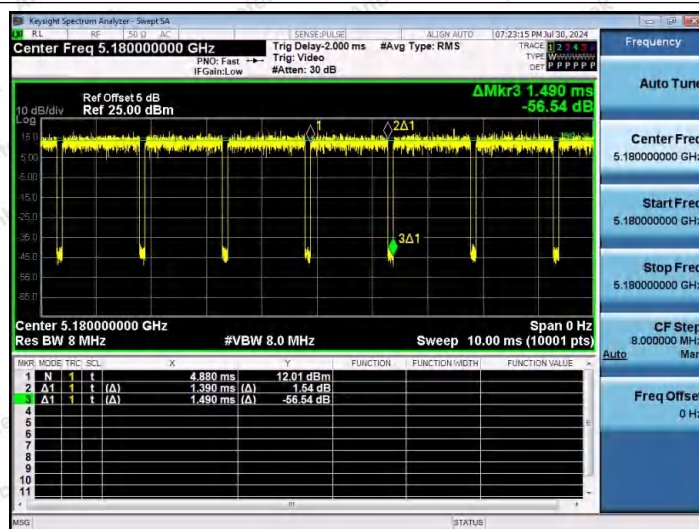
NTNV-11A-Ant1-5180
