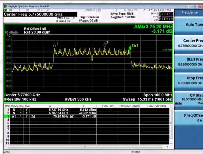
11AC80MIMO-Ant1-5775-PASS
