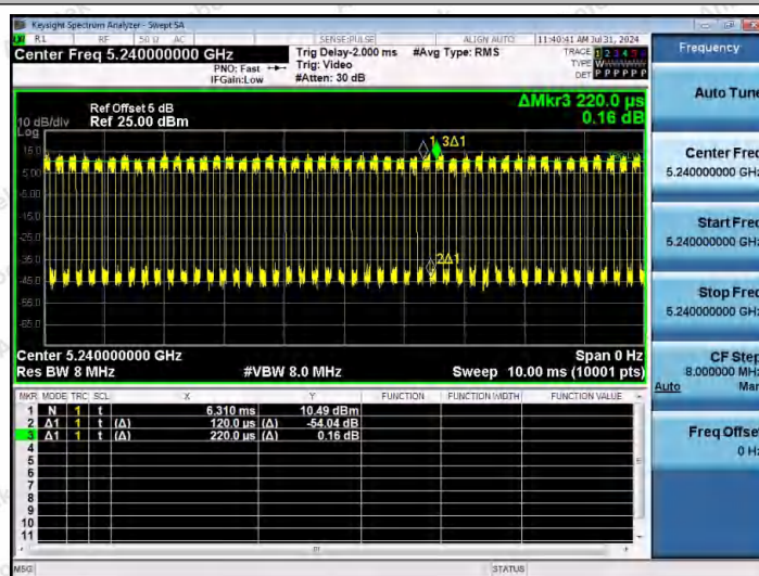
NTNV-11AX20MIMO-Ant2-5240
