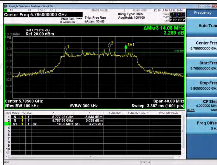
11N20MIMO-Ant1-5785-PASS
