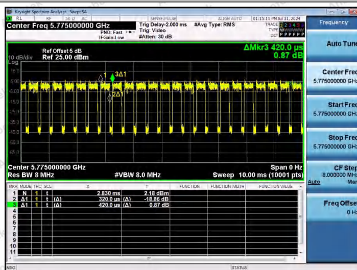
NTNV-11AC80MIMO-Ant2-5775
