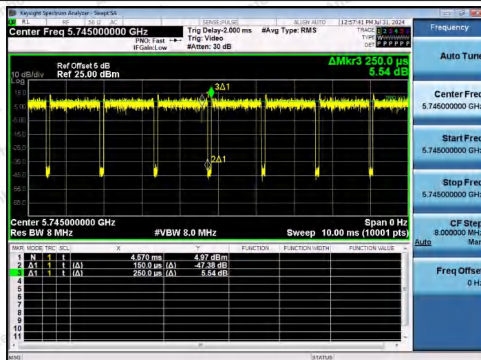
NTNV-11AC20MIMO-Ant2-5745
