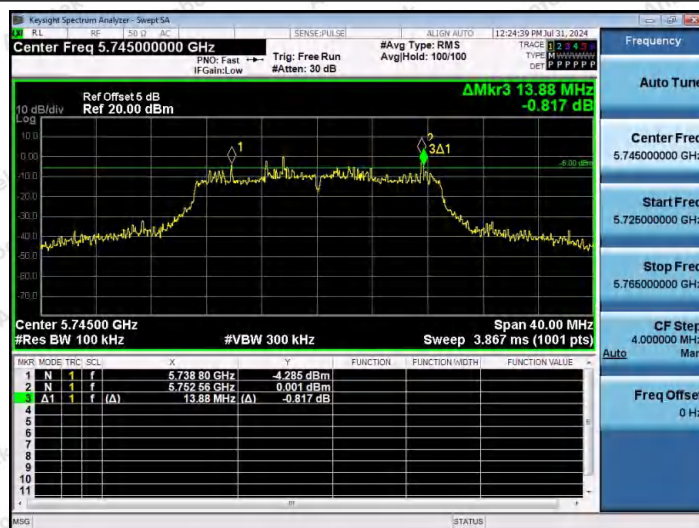
11N20MIMO-Ant2-5745-PASS
