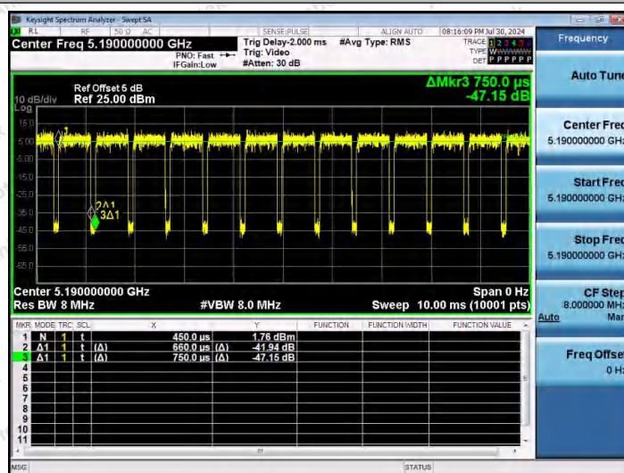
NTNV-11AC40MIMO-Ant1-5190
