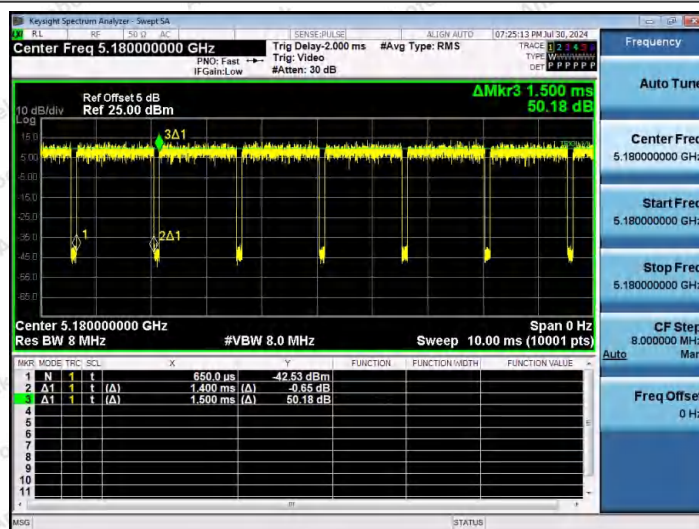
NTNV-11A-Ant2-5180
