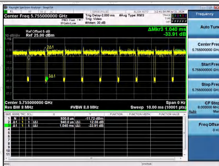
NTNV-11N40MIMO-Ant2-5755
