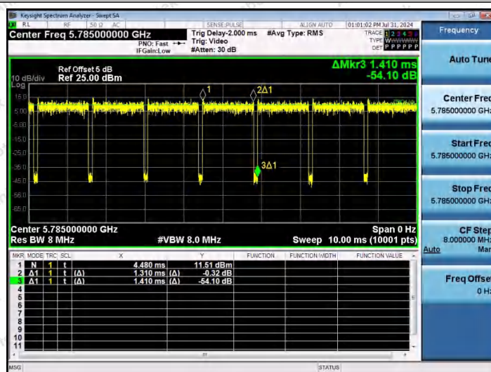
NTNV-11AC20MIMO-Ant2-5785
