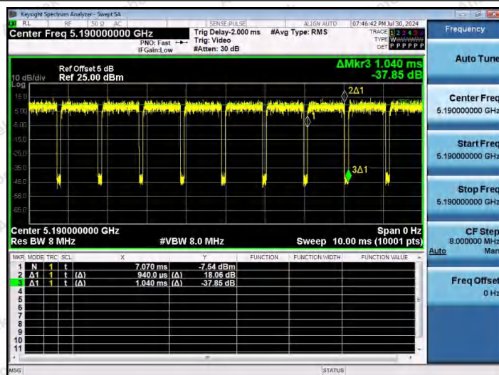
NTVN-11N40MIMO-Ant2-5190
