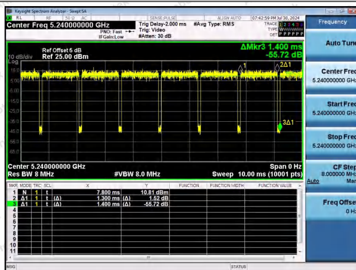
NTVN-11N20MIMO-Ant2-5240
