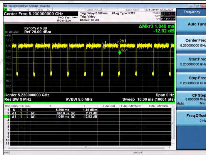
NTVN-11N40MIMO-Ant1-5230
