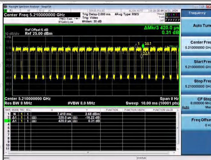
NTNV-11AC80MIMO-Ant2-5210
