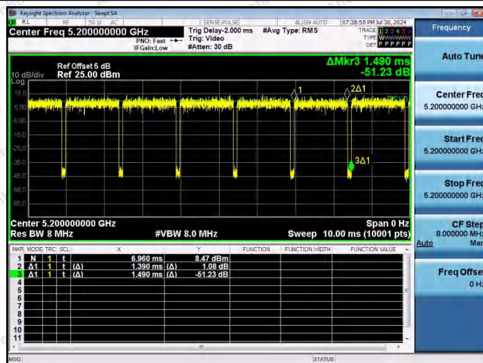
NTNV-11A-Ant2-5200
