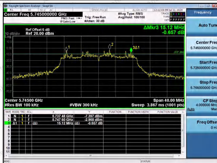
11N20MIMO-Ant1-5745-PASS
