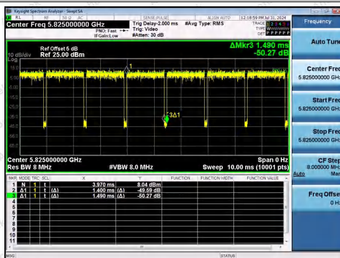
NTNV-11A-Ant1-5825
