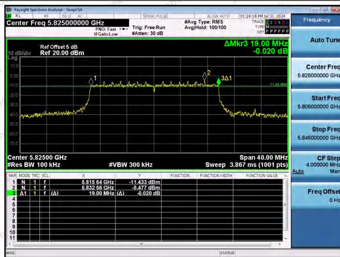
11AX20MIMO-Ant1-5825-PASS
