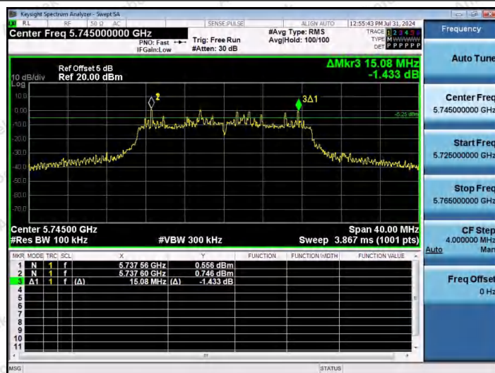
11AC20MIMO-Ant1-5745-PASS
