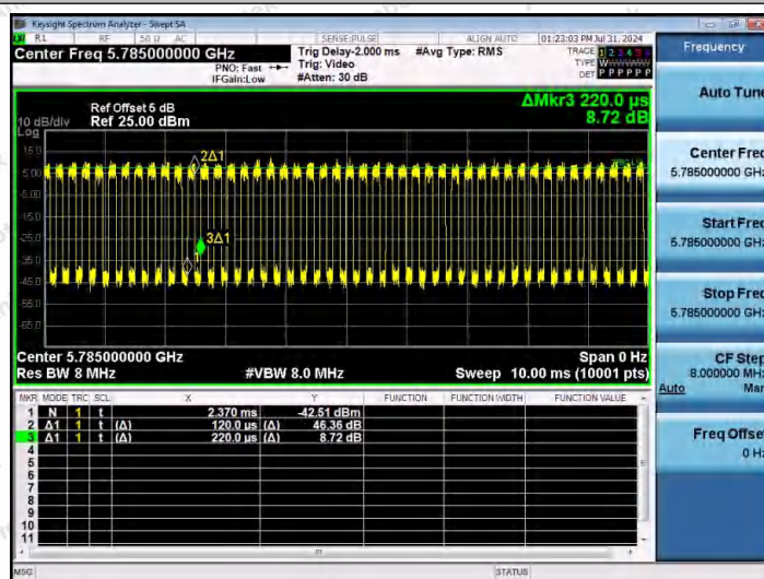
NTNV-11AX20MIMO-Ant2-5785
