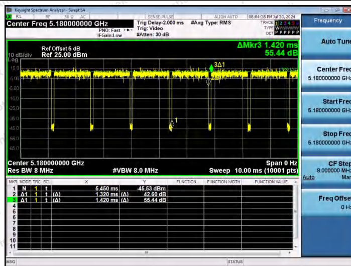
NTNV-11AC20MIMO-Ant1-5180
