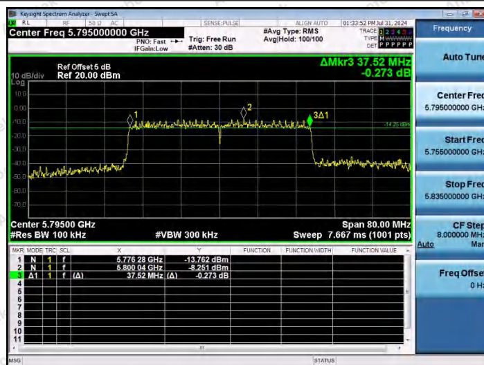
11AX40MIMO-Ant2-5795-PASS
