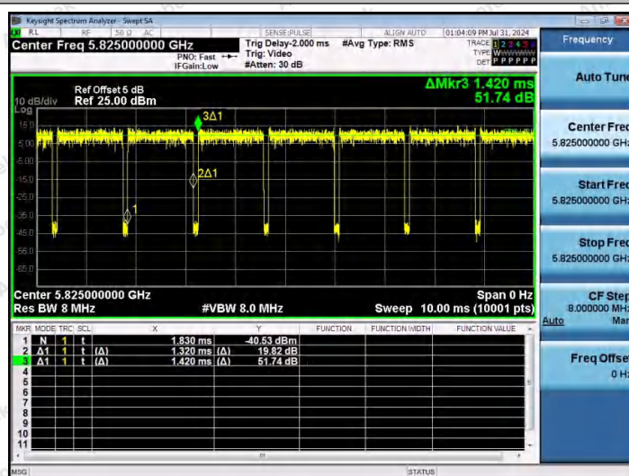
NTNV-11AC20MIMO-Ant2-5825
