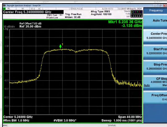
11AX20MIMO-Ant2-5240-PASS
