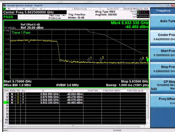
11AX80MIMO-Ant2-5775-PASS
