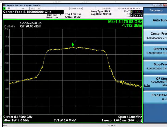
11AC20MIMO-Ant1-5180-PASS
