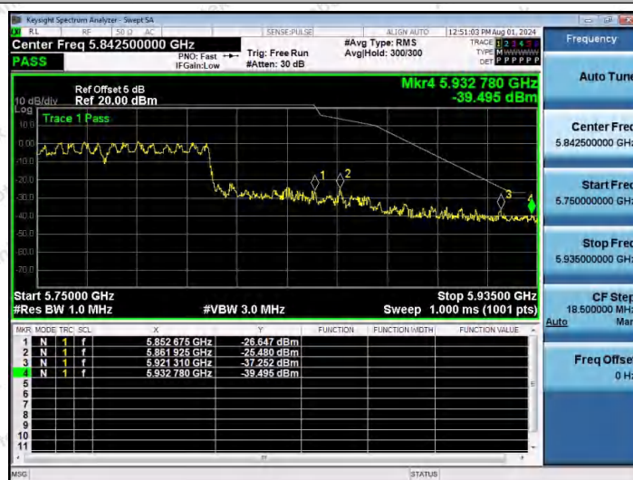
11AC80MIMO-Ant2-5775-PASS
