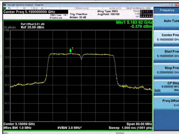
11AC40MIMO-Ant2-5190-PASS
