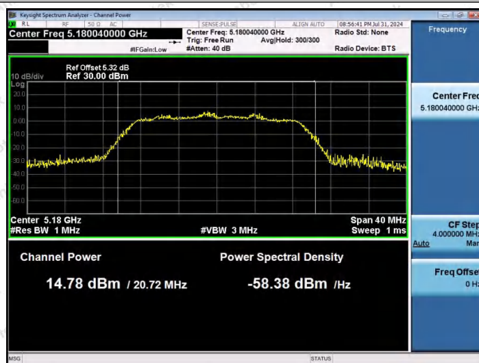
11A20MIMO-Ant1-5180-PASS
