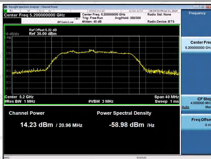
11AC20MIMO-Ant1-5200-PASS
