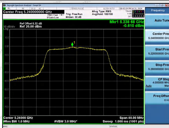
11N20MIMO-Ant2-5240-PASS
