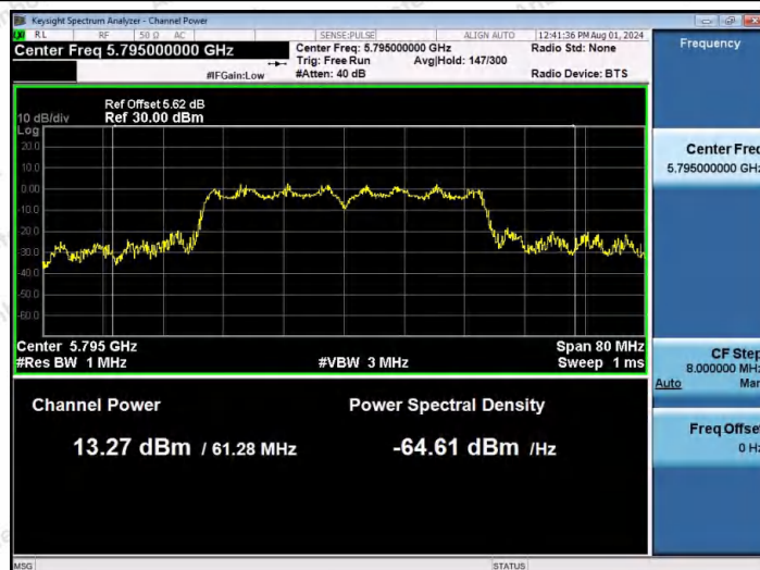
11AC40MIMO-Ant2-5795-PASS
