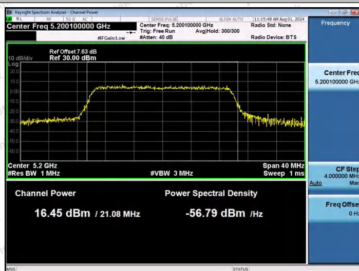
11AX20MIMO-Ant2-5200-PASS
