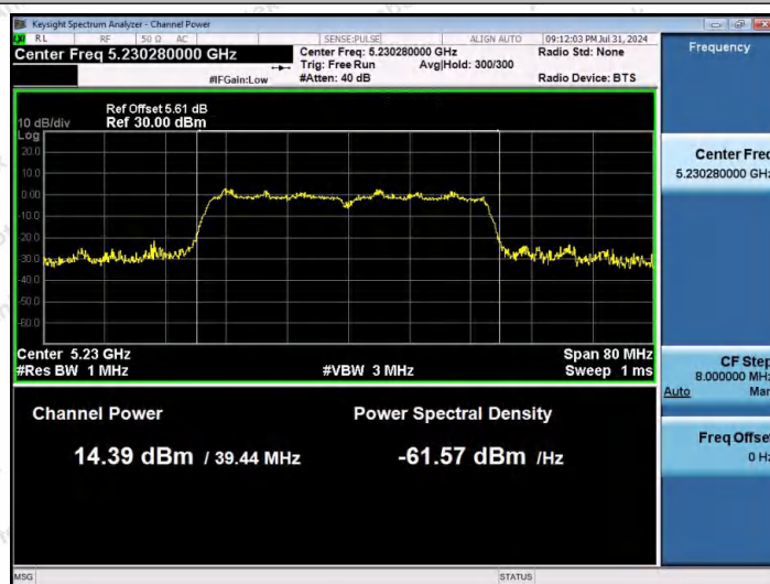
11AC40MIMO-Ant2-5230-PASS
