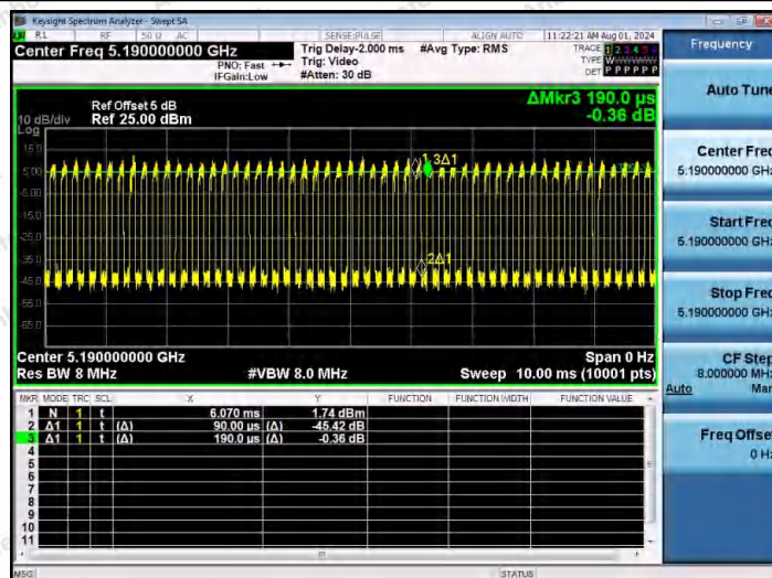
NTNV-11AX40MIMO-Ant2-5190
