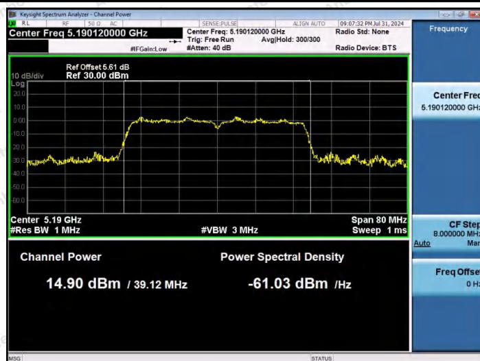
11AC40MIMO-Ant2-5190-PASS
