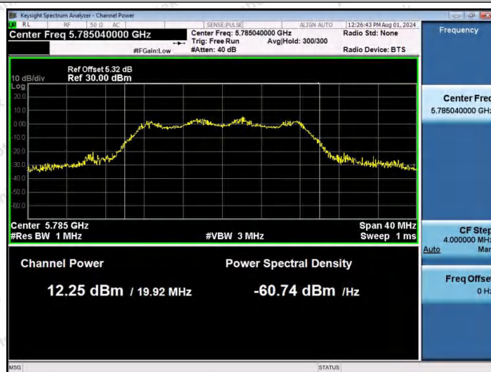
11AC20MIMO-Ant2-5785-PASS
