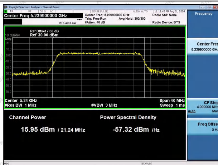
11AX20MIMO-Ant2-5240-PASS
