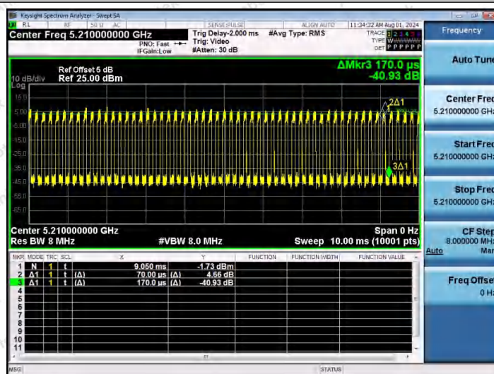
NTNV-11AX80MIMO-Ant2-5210
