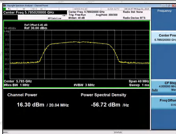
11AX20MIMO-Ant2-5785-PASS
