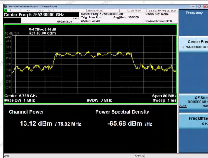
11N40MIMO-Ant2-5755-PASS
