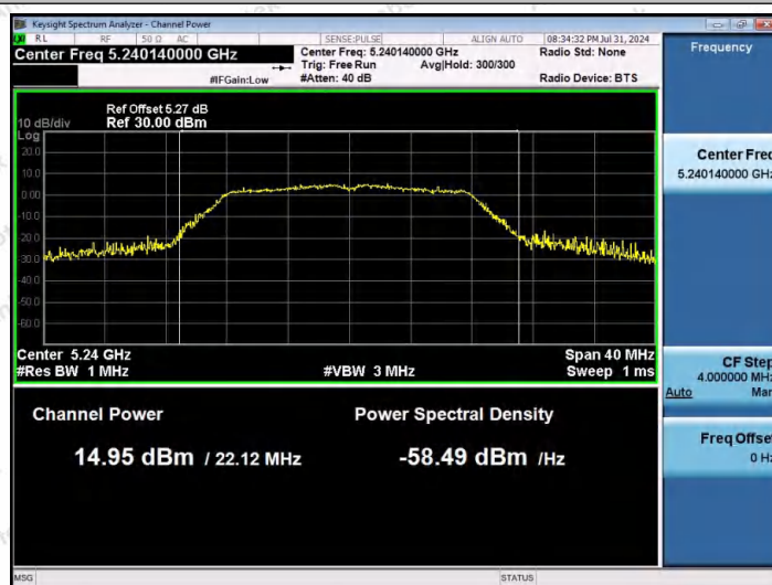
11A-Ant2-5240-PASS
