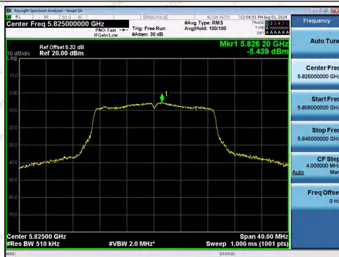
11N20MIMO-Ant2-5825-PASS
