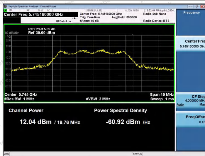
11AC20MIMO-Ant1-5745-PASS
