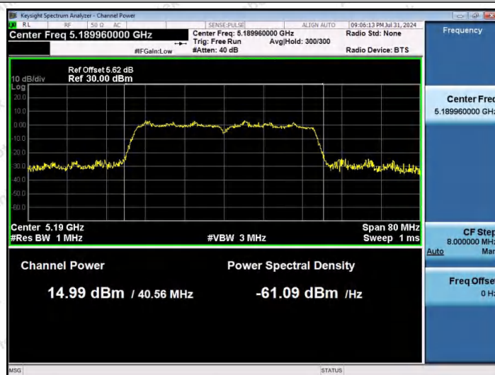
11AC40MIMO-Ant1-5190-PASS
