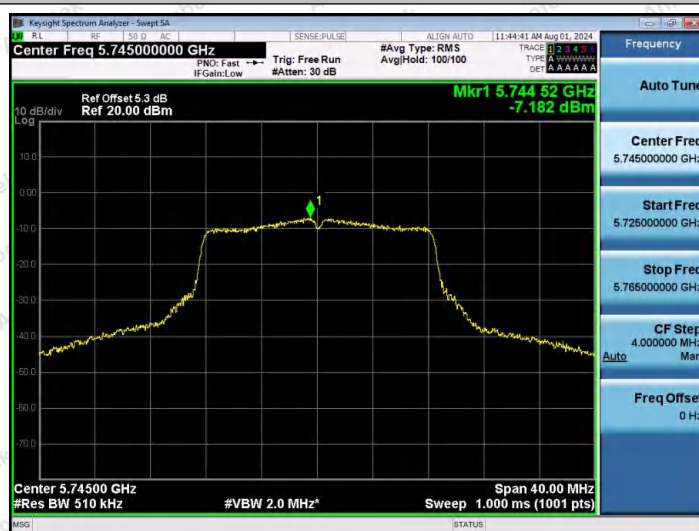
11A-Ant2-5745-PASS
