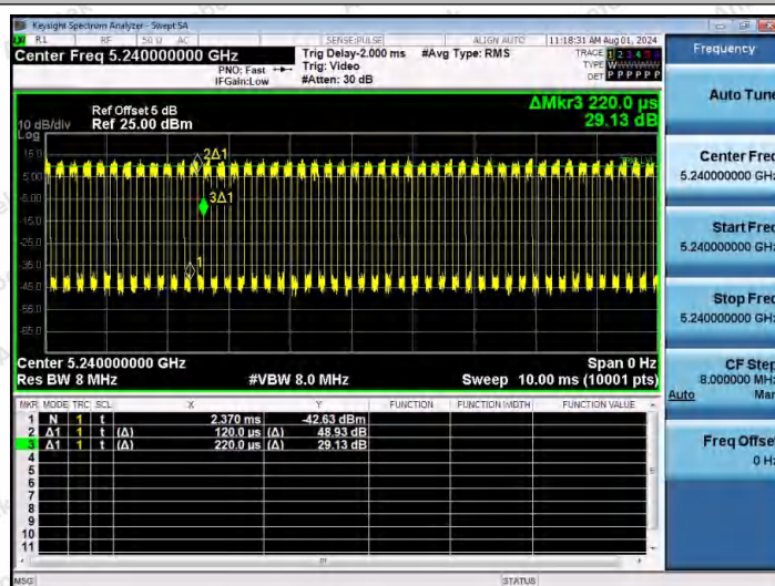
NTNV-11AX20MIMO-Ant2-5240
