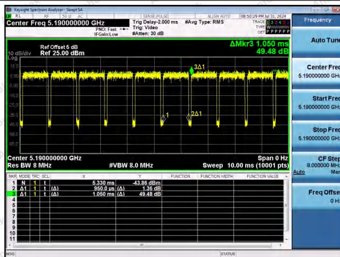
NTNV-11N40MIMO-Ant2-5190
