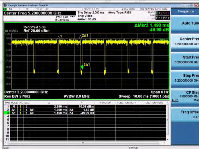
NTNV-11A-Ant2-5200
