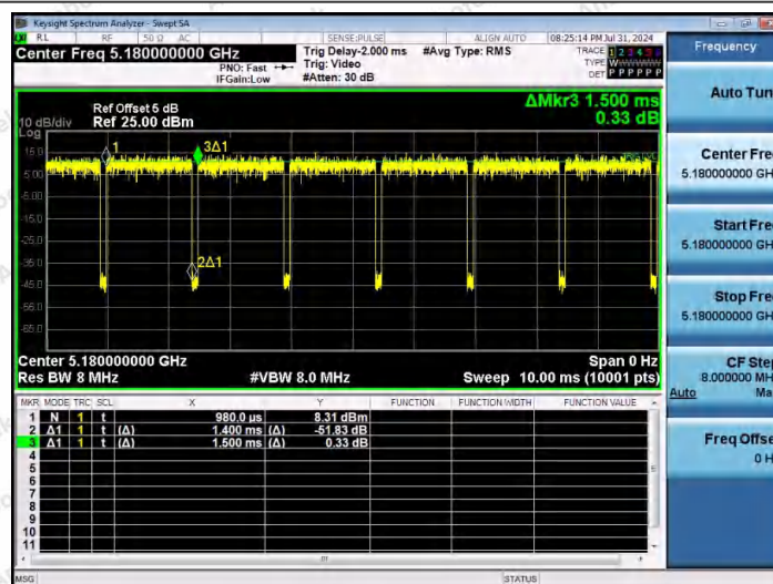
NTNV-11A-Ant2-5180
