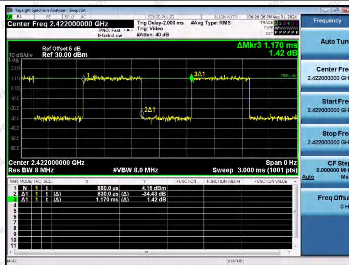
NTNV-11AX40MIMO-Ant2-2422
