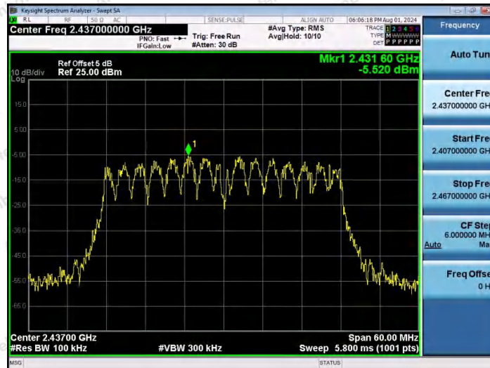
11N40MIMO-Ant1-2437-0~Reference-PASS
