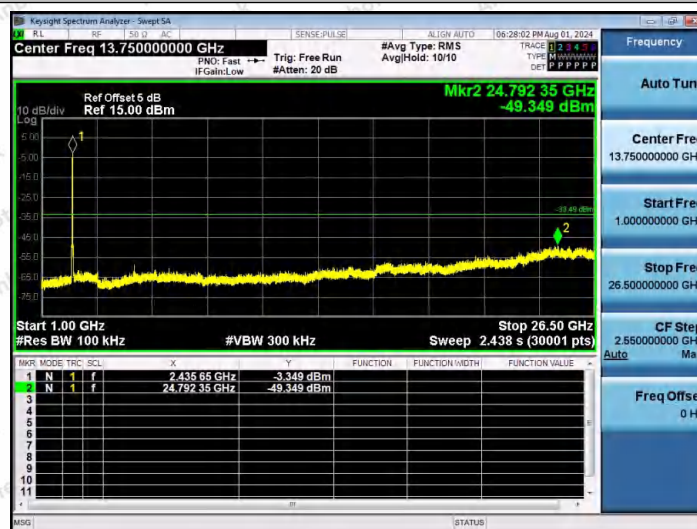
11AX40MIMO-Ant2-2422-1000~26500-PASS
