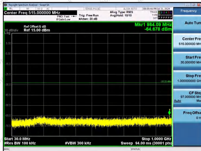
11N20MIMO-Ant1-2437-30~1000-PASS
