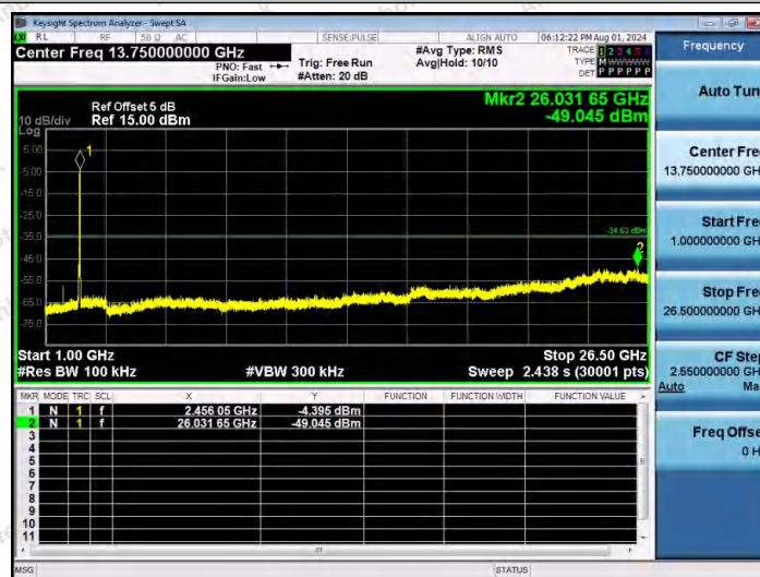
11N40MIMO-Ant2-2452-1000~26500-PASS
