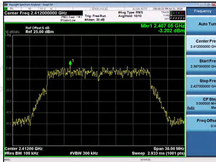
11N20MIMO-Ant1-2412-0~Reference-PASS
