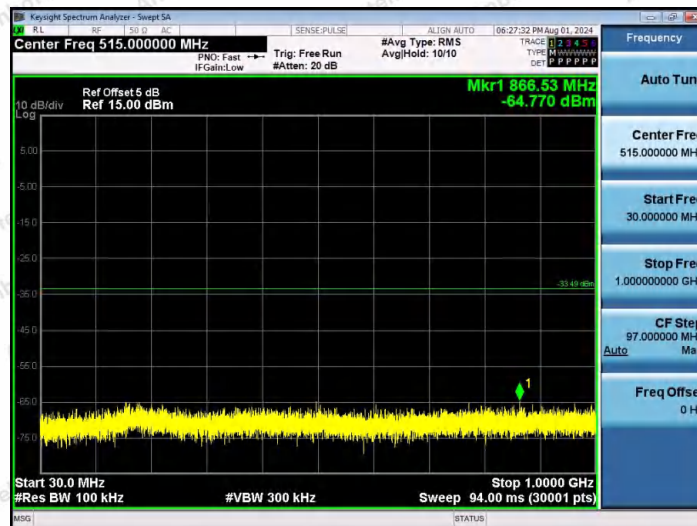
11AX40MIMO-Ant2-2422-30~1000-PASS
