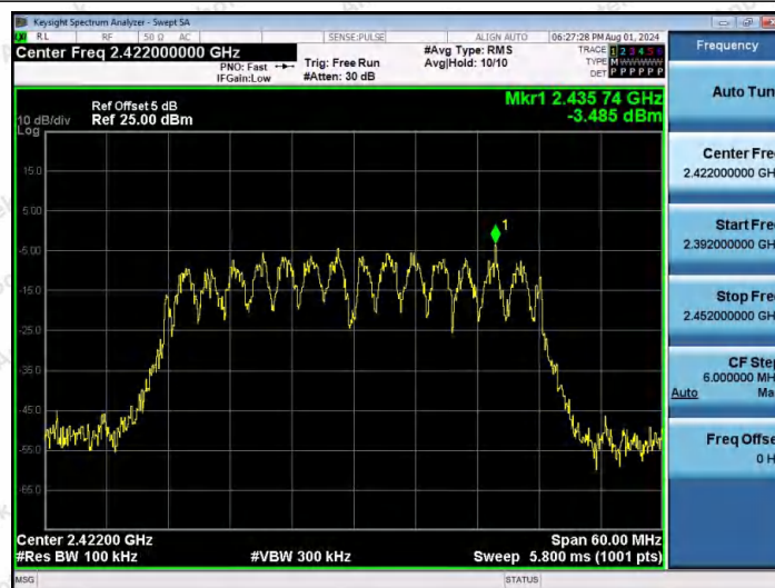
11AX40MIMO-Ant2-2422-0~Reference-PASS
