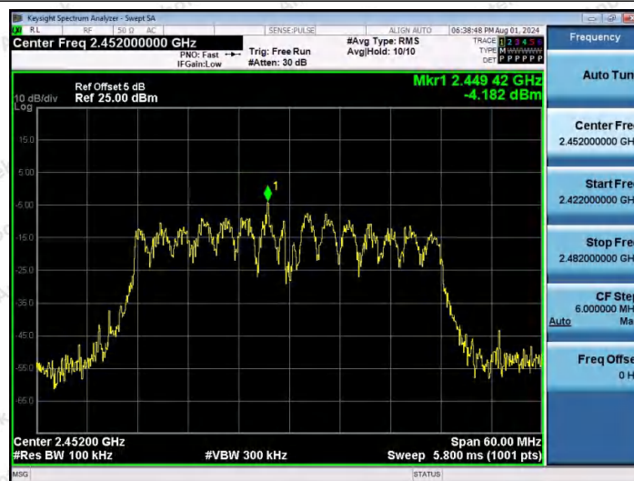
11AX40MIMO-Ant2-2452-0~Reference-PASS
