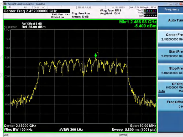
11N40MIMO-Ant1-2452-0~Reference-PASS
