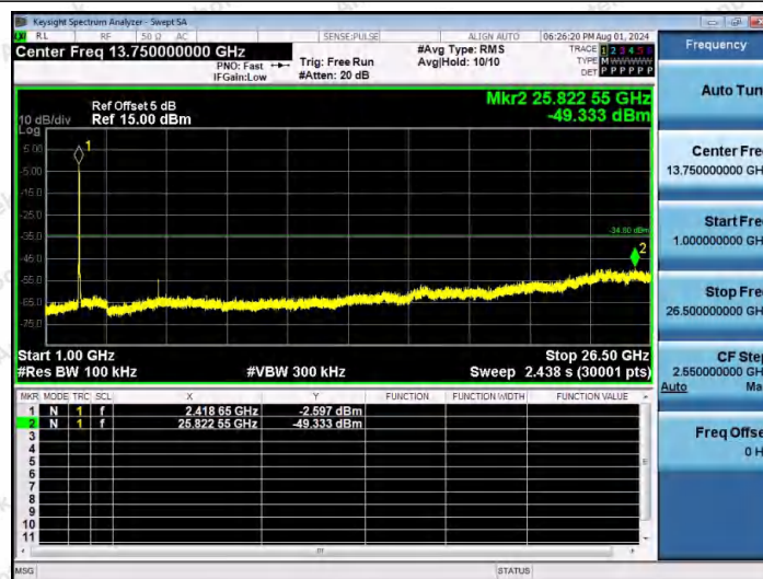
11AX40MIMO-Ant1-2422-1000~26500-PASS
