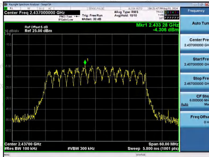
11AX40MIMO-Ant1-2437-0~Reference-PASS
