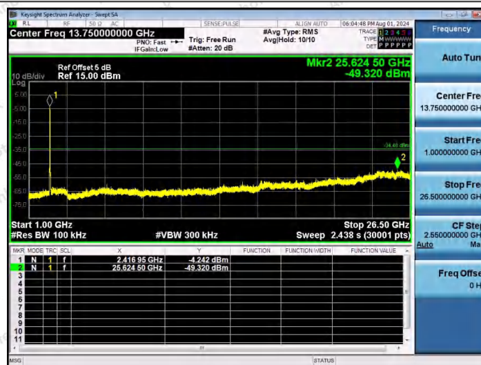
11N40MIMO-Ant2-2422-1000~26500-PASS
