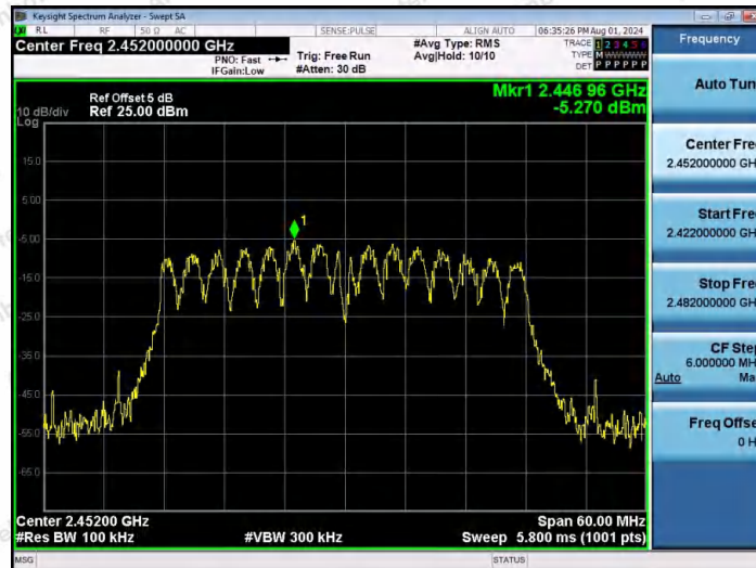
11AX40MIMO-Ant1-2452-0~Reference-PASS
