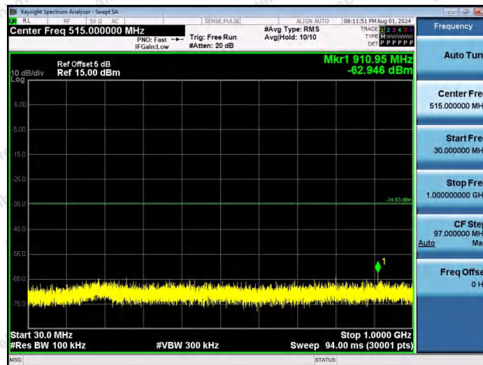
11N40MIMO-Ant2-2452-30~1000-PASS
