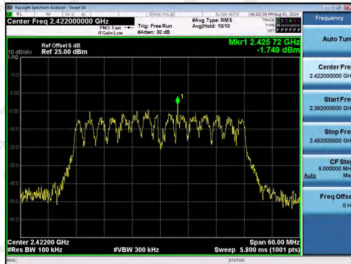
11N40MIMO-Ant1-2422-0~Reference-PASS
