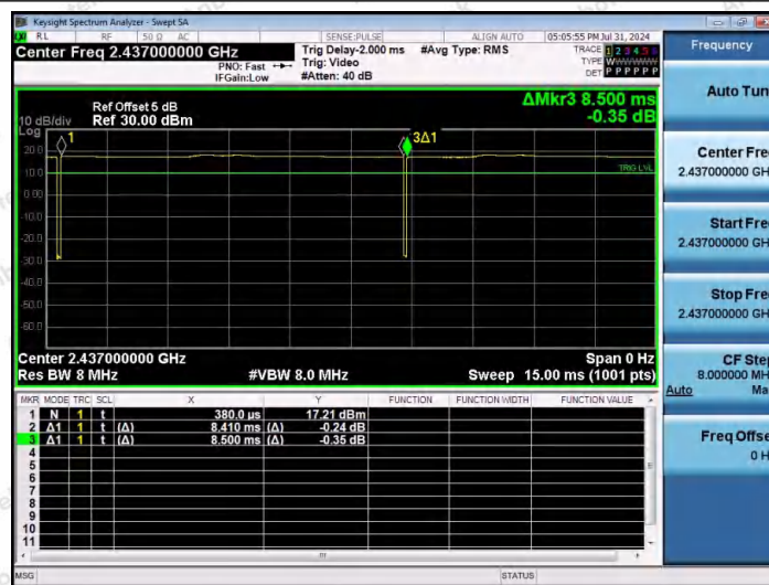
NTNV-11B-Ant2-2437
