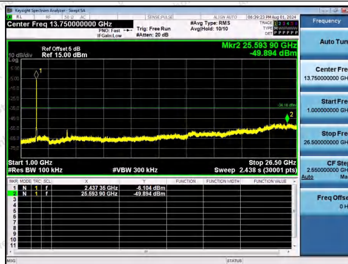
11AX40MIMO-Ant2-2452-1000~26500-PASS
