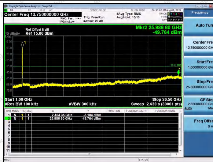
11AX40MIMO-Ant1-2452-1000~26500-PASS
