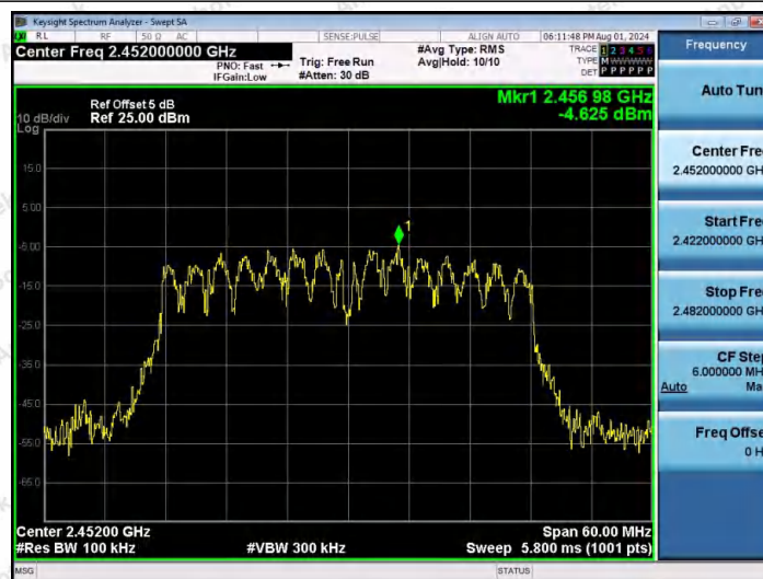
11N40MIMO-Ant2-2452-0~Reference-PASS
