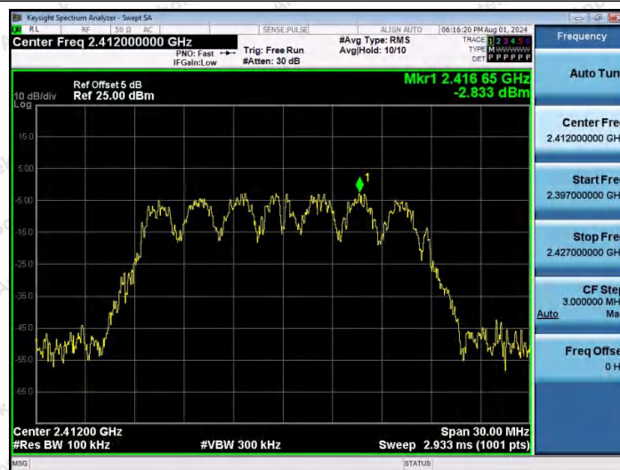
11AX20MIMO-Ant2-2412-0~Reference-PASS
