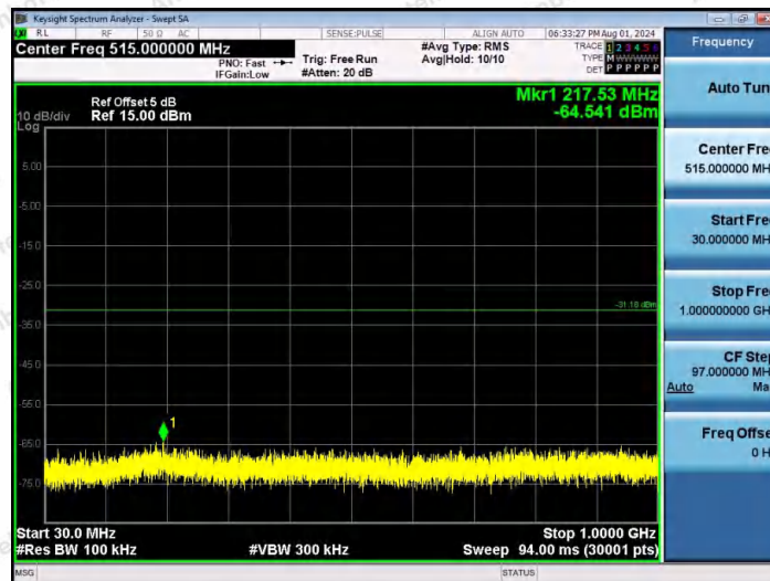
11AX40MIMO-Ant2-2437-30~1000-PASS
