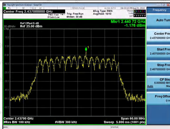
11AX40MIMO-Ant2-2437-0~Reference-PASS
