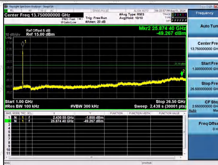
11AX40MIMO-Ant2-2437-1000~26500-PASS
