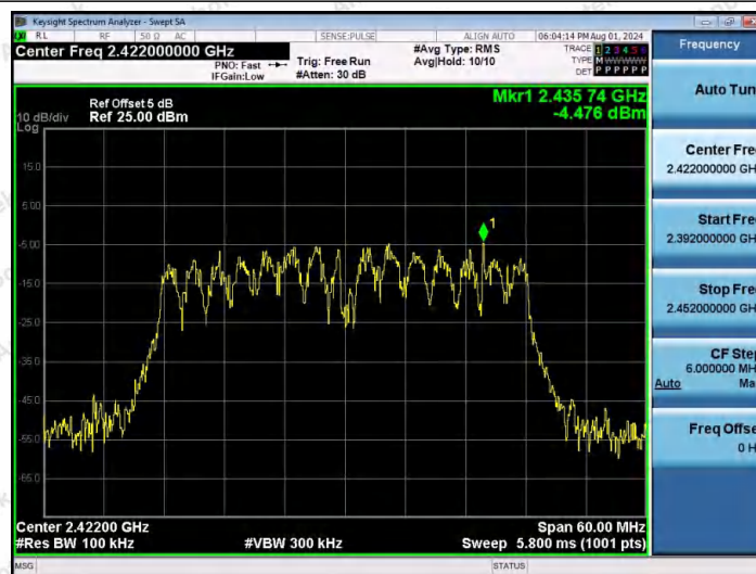
11N40MIMO-Ant2-2422-0~Reference-PASS
