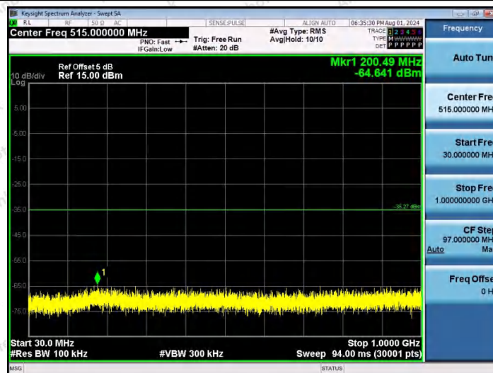
11AX40MIMO-Ant1-2452-30~1000-PASS
