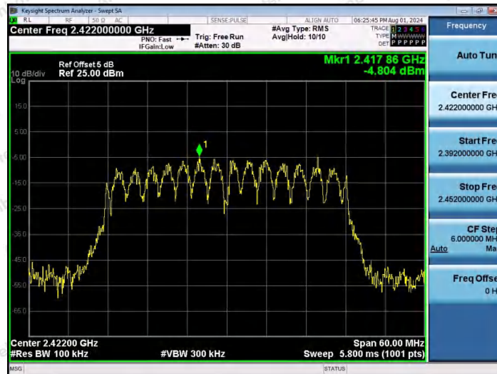
11AX40MIMO-Ant1-2422-0~Reference-PASS
