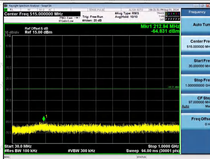
11AX40MIMO-Ant1-2437-30~1000-PASS
