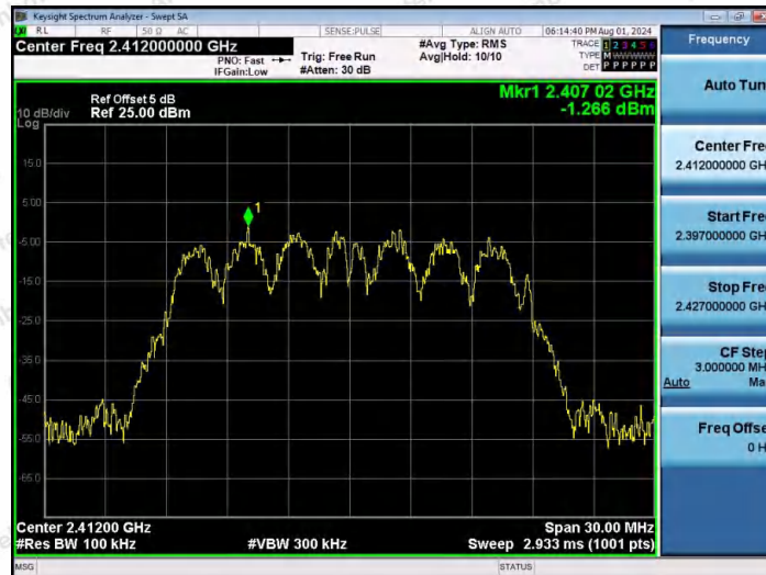
11AX20MIMO-Ant1-2412-0~Reference-PASS
