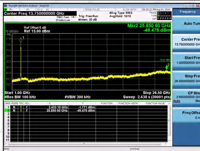
11AX40MIMO-Ant1-2437-1000~26500-PASS
