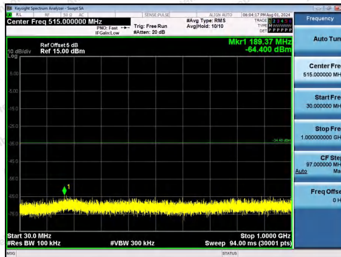
11N40MIMO-Ant2-2422-30~1000-PASS
