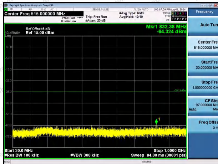
11N40MIMO-Ant2-2437-30~1000-PASS
