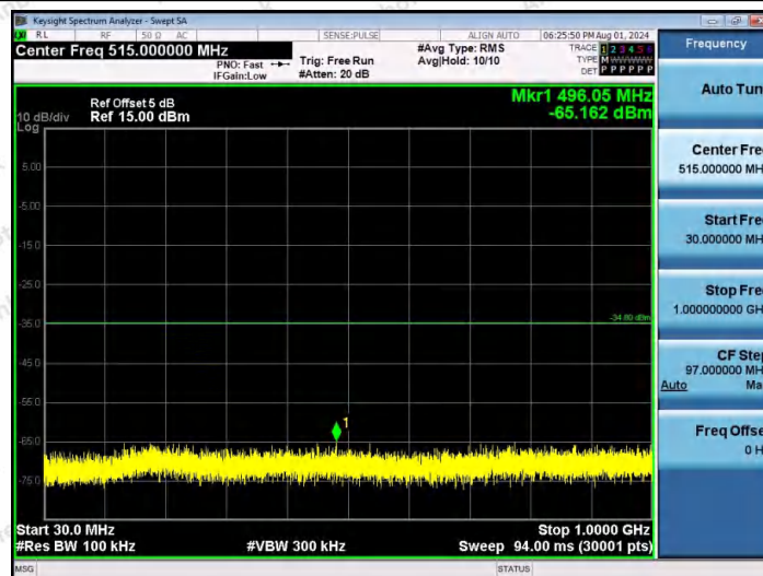
11AX40MIMO-Ant1-2422-30~1000-PASS
