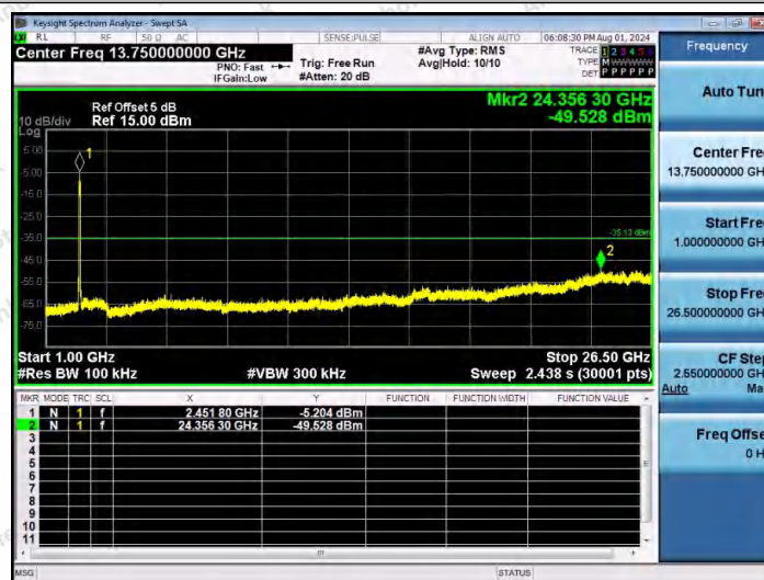
11N40MIMO-Ant2-2437-1000~26500-PASS
