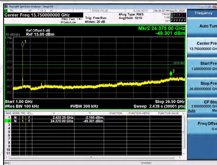
11AX20MIMO-Ant2-2437-1000~26500-PASS
