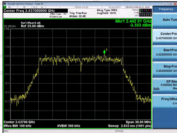
11N20MIMO-Ant1-2437-0~Reference-PASS
