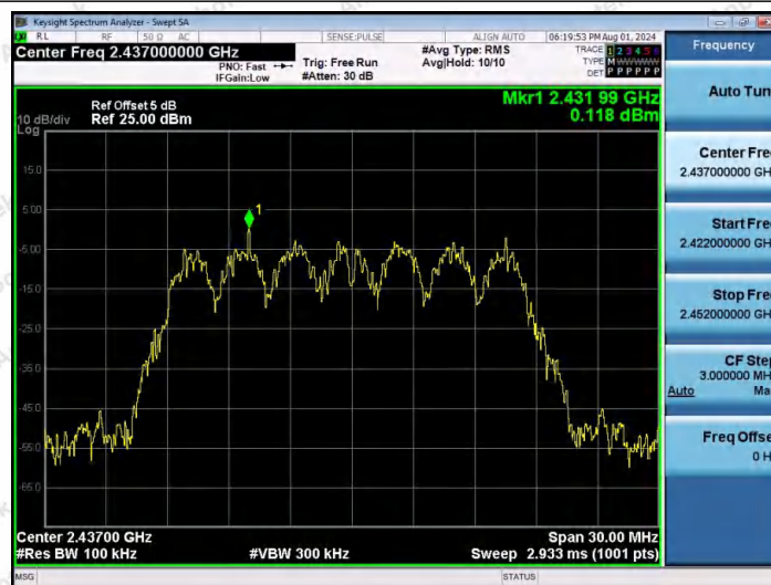
11AX20MIMO-Ant2-2437-0~Reference-PASS
