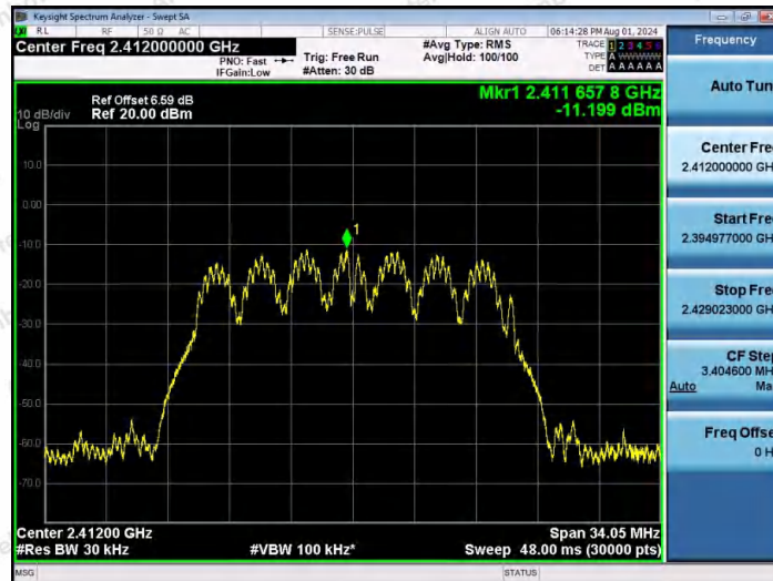
11AX20MIMO-Ant1-2412-PASS
