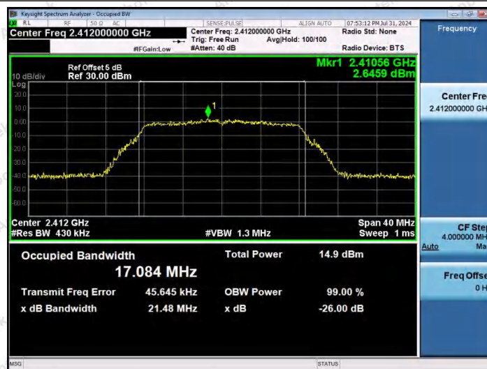
11G-Ant2-2412
