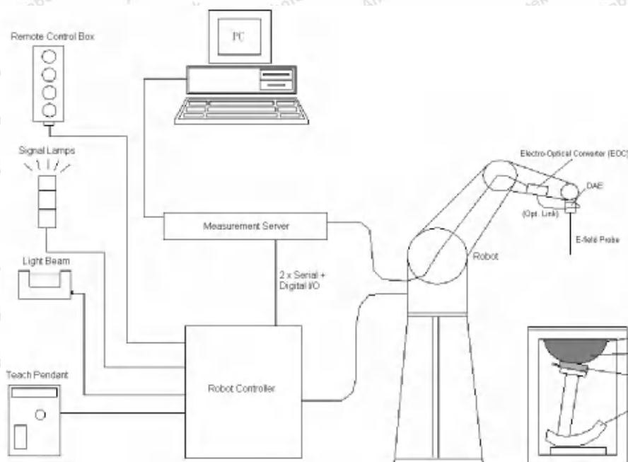
DASY System Configurations
