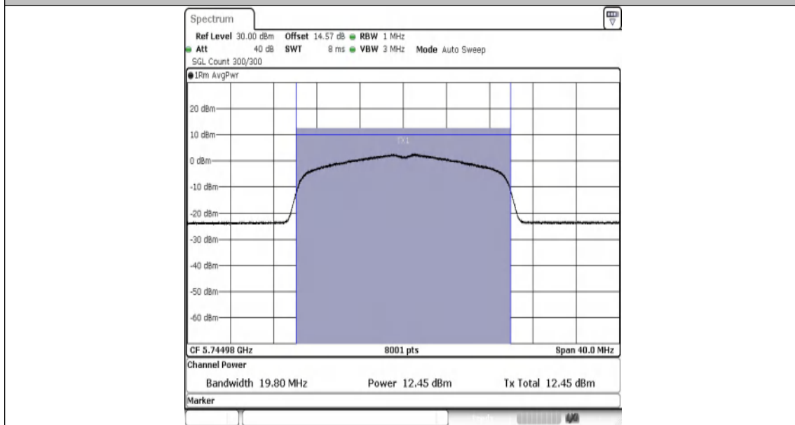
11AX20MIMO-Ant2-5745-PASS
