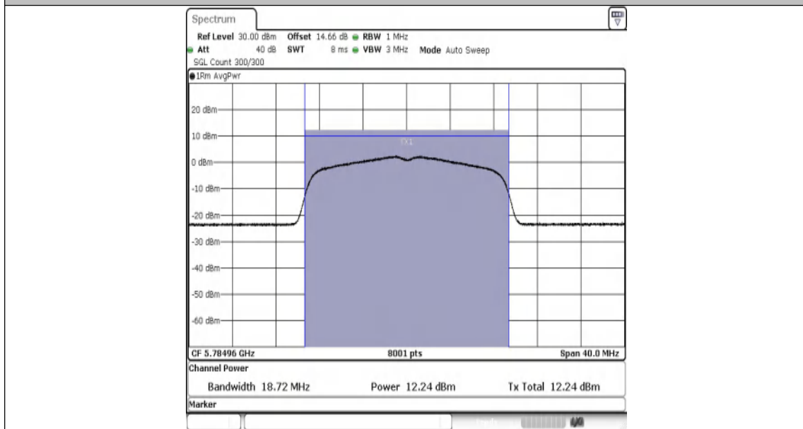
11N20MIMO-Ant1-5785-PASS
