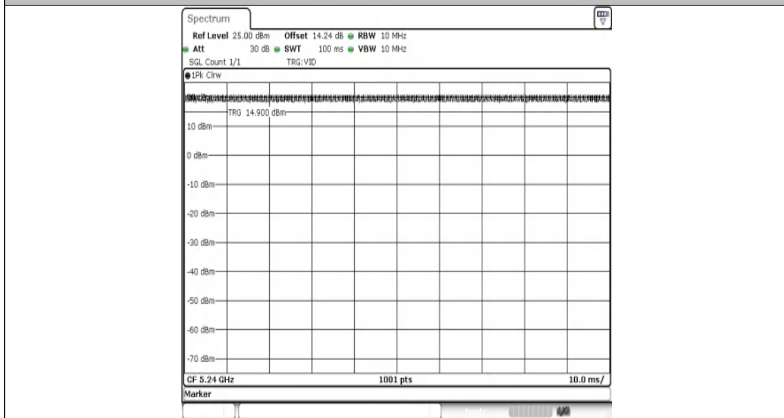
NTNV-11AC20MIMO-Ant1-5240
