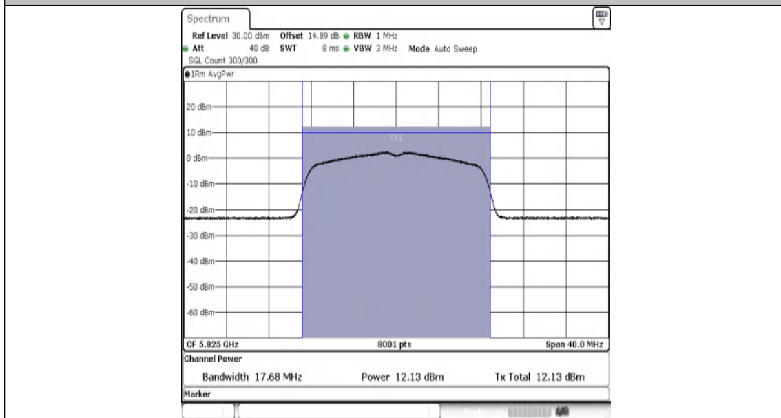
11A-Ant2-5825-PASS
