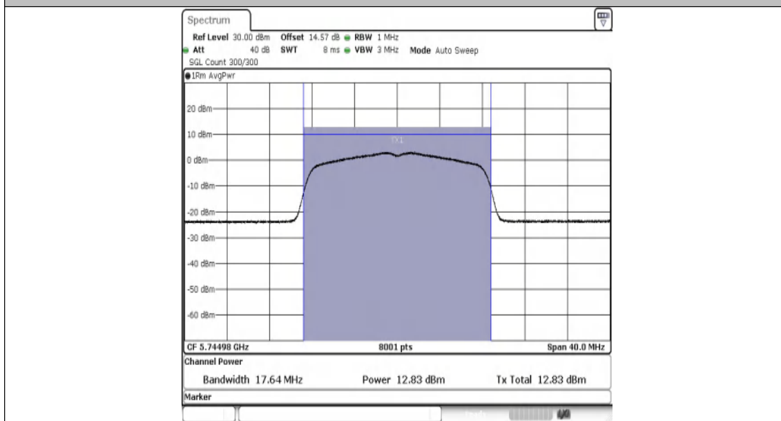
11A-Ant1-5745-PASS
