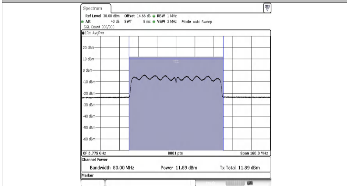
11AC80MIMO-Ant2-5775-PASS
