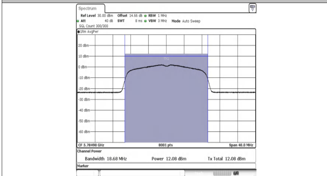
11AC20MIMO-Ant2-5785-PASS
