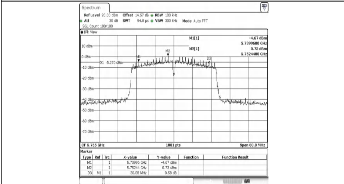
11N40MIMO-Ant2-5755-PASS
