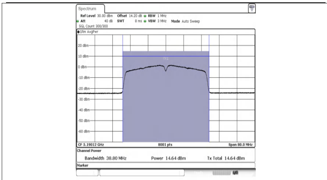
11N40MIMO-Ant1-5190-PASS
