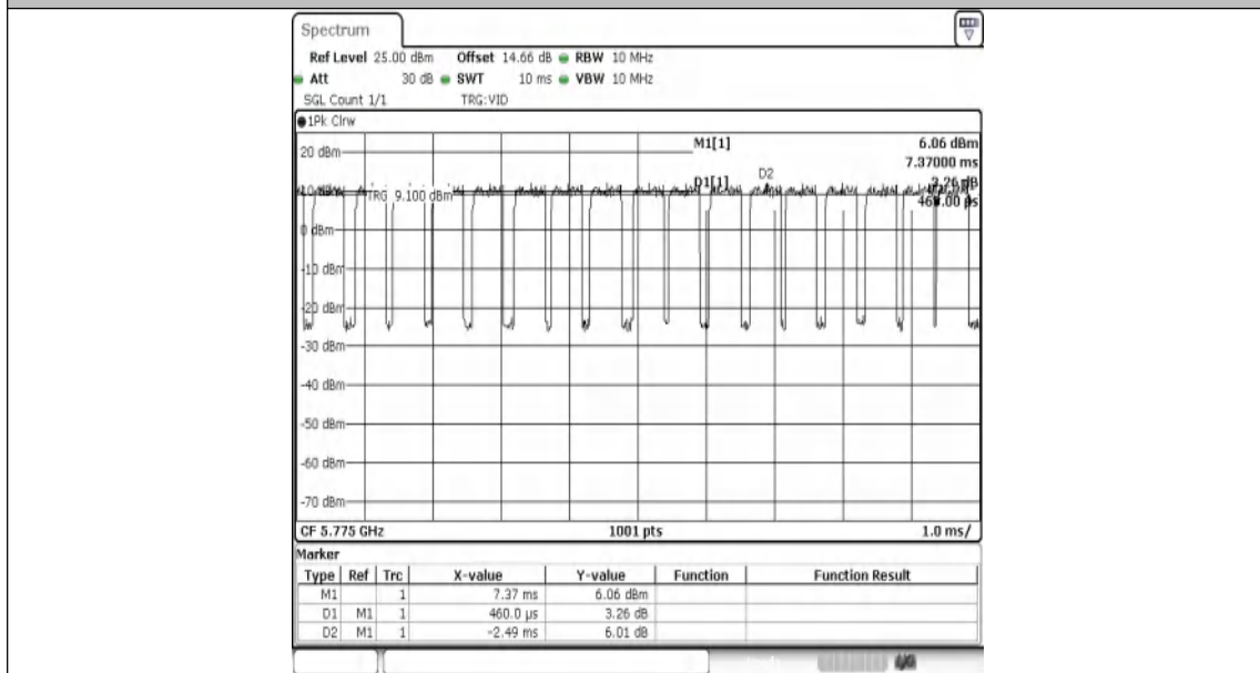
NTNV-11AC80MIMO-Ant1-5775
