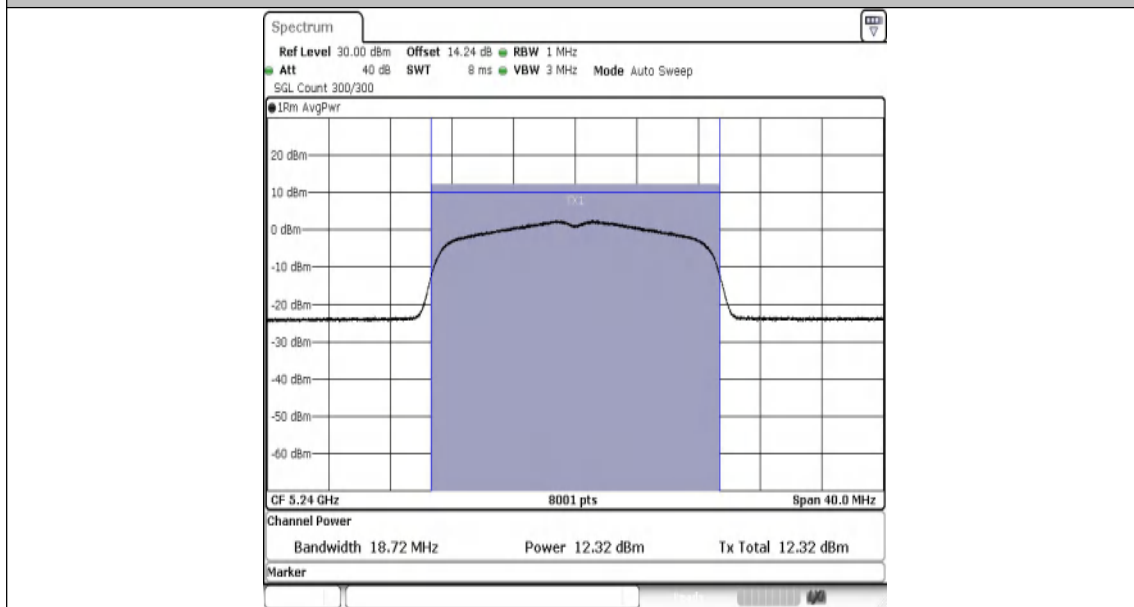
11AC20MIMO-Ant2-5240-PASS
