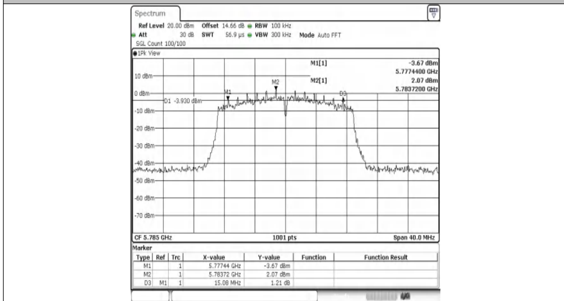
11AC20MIMO-Ant1-5785-PASS
