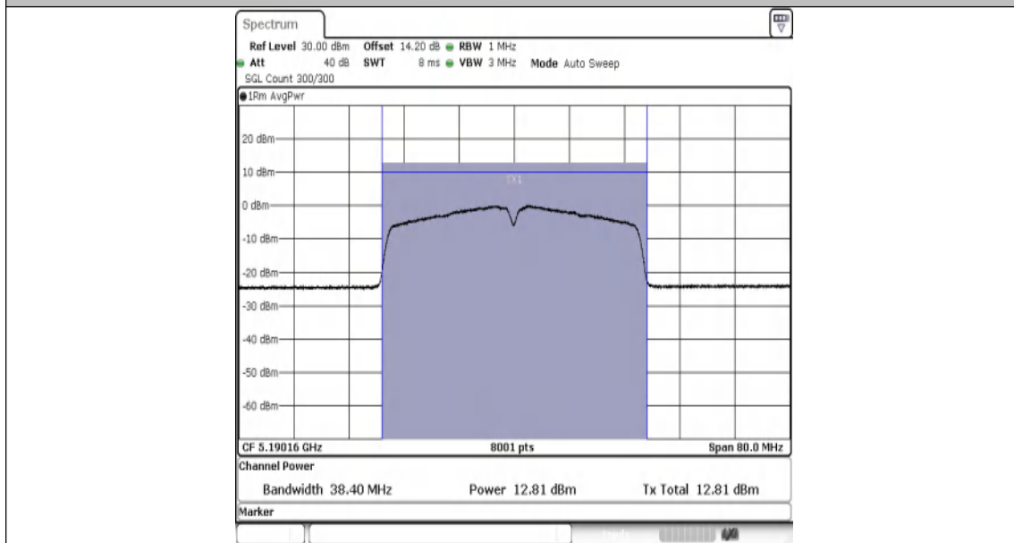
11N40MIMO-Ant2-5190-PASS
