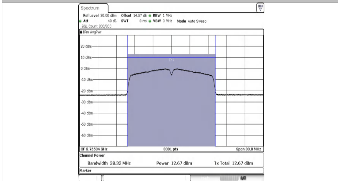
11AC40MIMO-Ant2-5755-PASS
