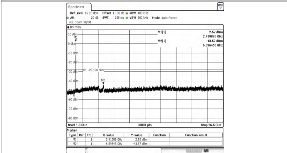
11N40MIMO-Ant1-2422-1000~26500-PASS
