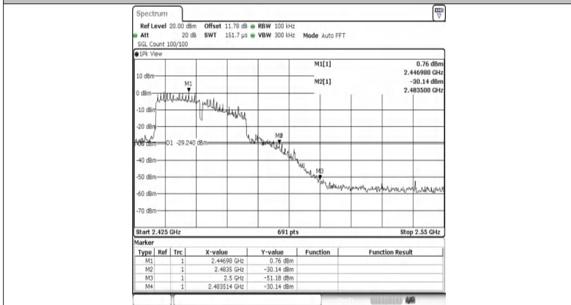
11N40MIMO-Ant1-2452-PASS
