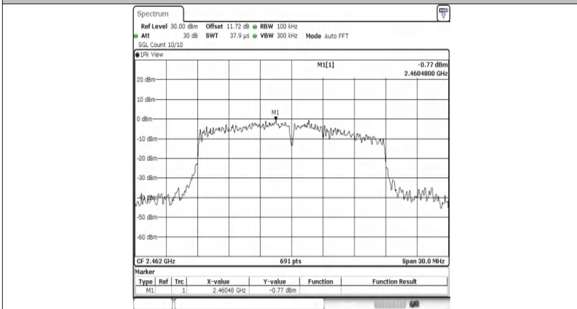
11N20MIMO-Ant1-2462-0~Reference-PASS
