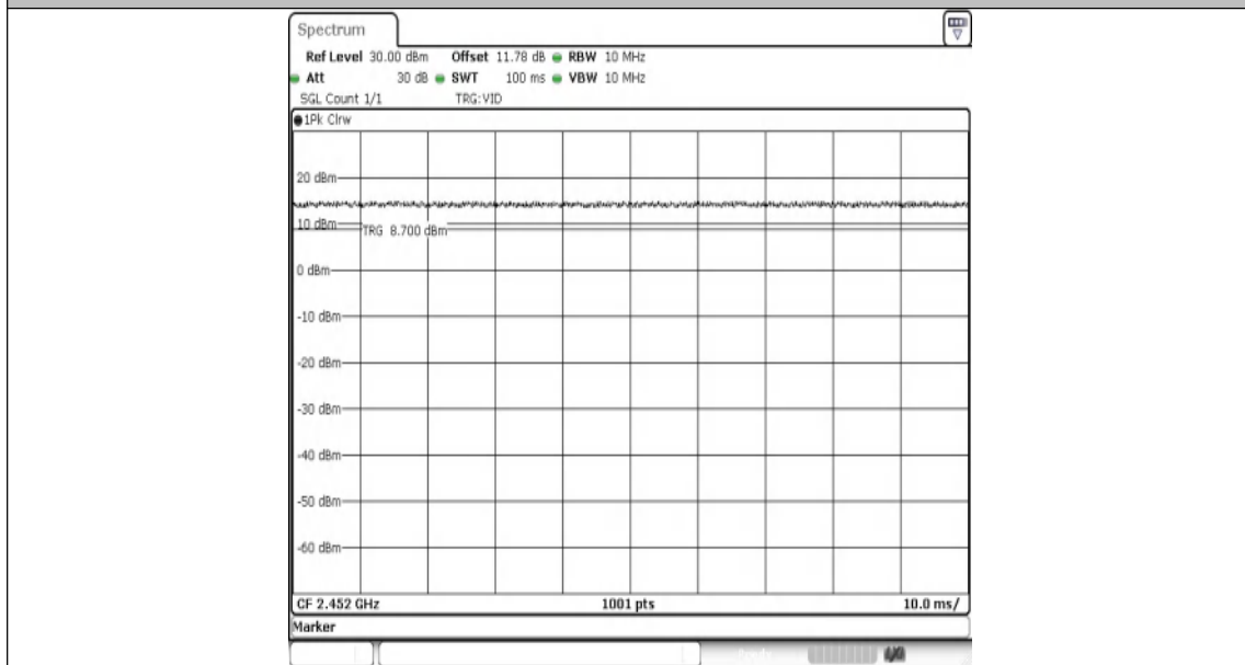
NTNV-11N40MIMO-Ant1-2452
