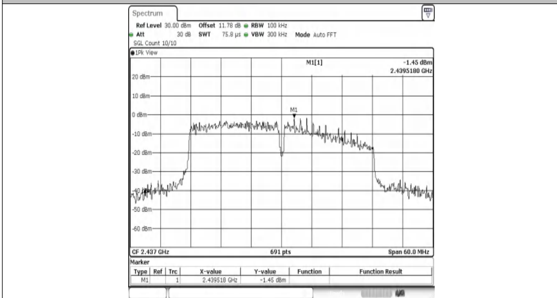
11N40MIMO-Ant1-2437-0~Reference-PASS
