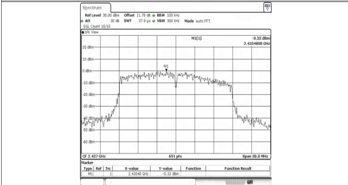
11N20MIMO-Ant2-2437-0~Reference-PASS
