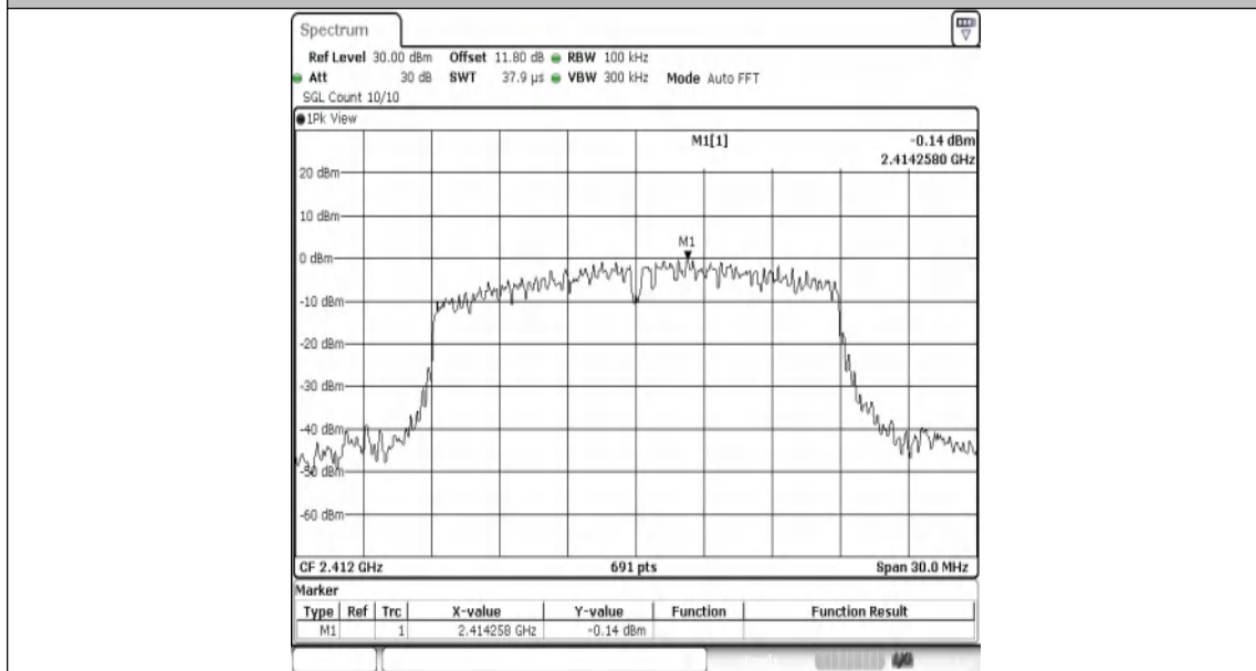
11N20MIMO-Ant1-2412-0~Reference-PASS
