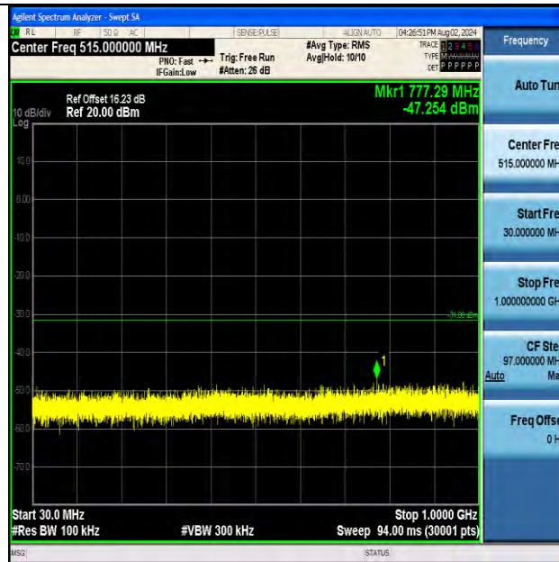
11AX20MIMO-Ant2-2437 -30~1000-PASS
