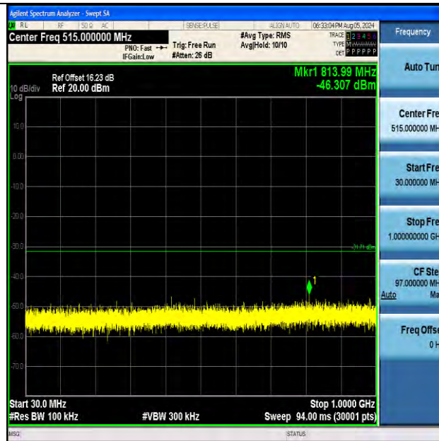
11AX40MIMO-Ant2-2422 -30~1000-PASS
