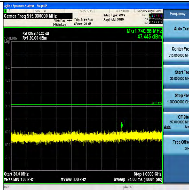
11AX20MIMO-Ant2-2412 -30~1000-PASS
