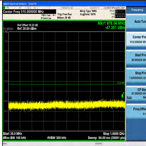
11AX40MIMO-Ant2-2452 -30~1000-PASS
