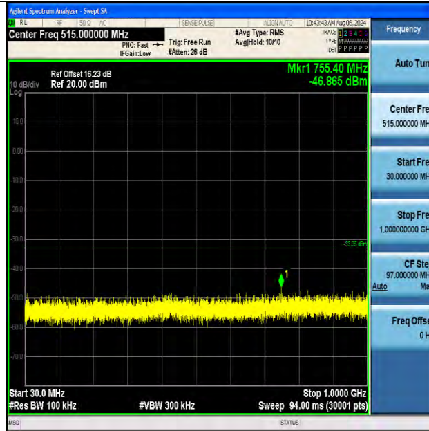
11AX40MIMO-Ant2-2437 -30~1000-PASS
