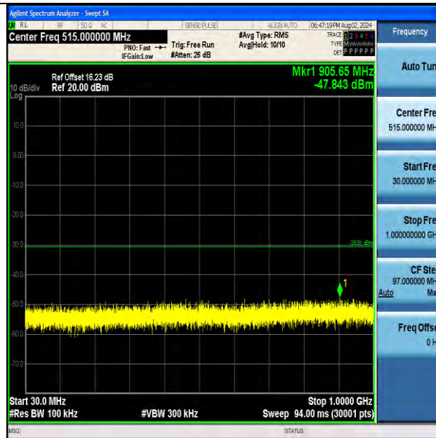
11AX20MIMO-Ant2-2462 -30~1000-PASS
