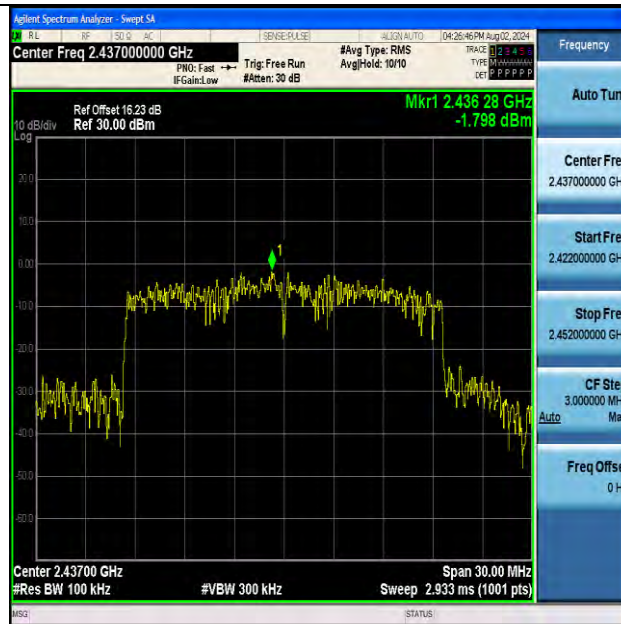
11AX20MIMO-Ant2-2437 -0~Reference-PASS
