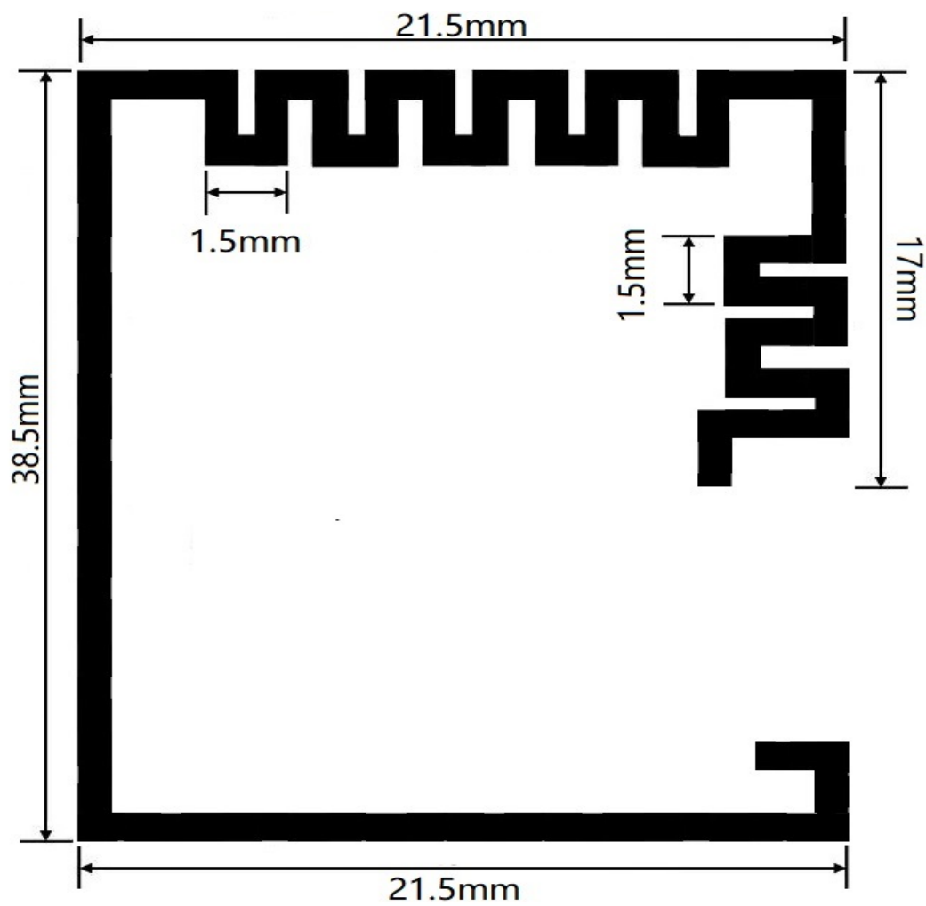
AntennaPhoto&Length(mm)
