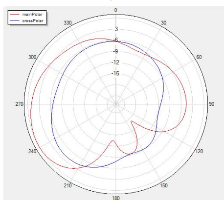
Phi=0 freq=2410MHz
