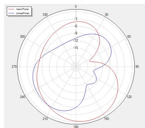
Theta=90 freq=2410MHz
