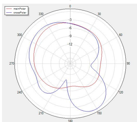
Phi=90 freq=2410MHz
