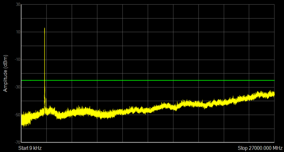
Band41 QPSK BW=20MHz Channel=39750 RB Size=100 Position=#0
