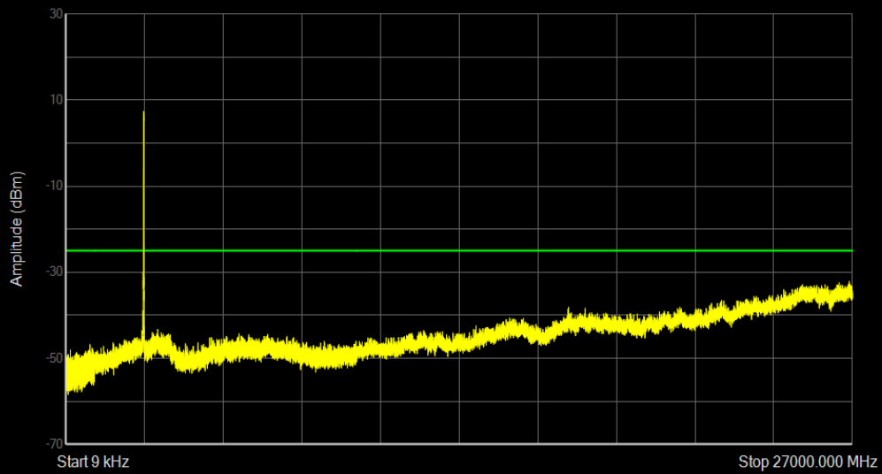
Band41 QPSK BW=10MHz Channel=41540 RB Size=50 Position=#0
