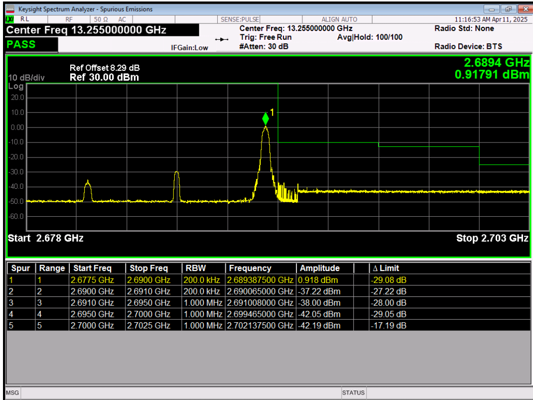
Band41 16QAM BW=10MHz Channel=41540 RB Size=50 Position=#0
