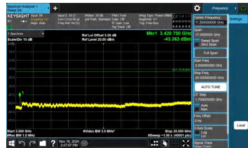
Band66-5MHz-QPSK-131997-1RB#0-3000~20000-PASS
