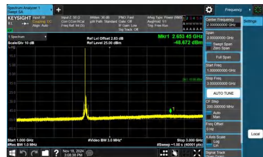
Band66-20MHz-QPSK-132322-1RB#0-1000~3000-PASS
