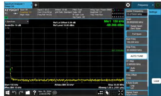
Band66-5MHz-QPSK-132322-1RB#24-0.15~30-PASS
