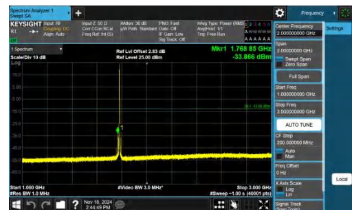
Band66-3MHz-QPSK-132657-1RB#14-1000~3000-PASS
