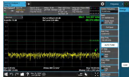
Band66-5MHz-QPSK-131997-1RB#0-0.009~0.15-PASS
