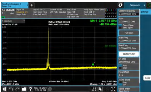
Band66-20MHz-QPSK-132322-1RB#99-1000~3000-PASS
