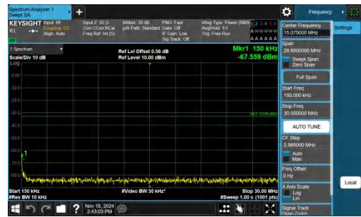
Band66-3MHz-QPSK-132322-1RB#14-0.15~30-PASS
