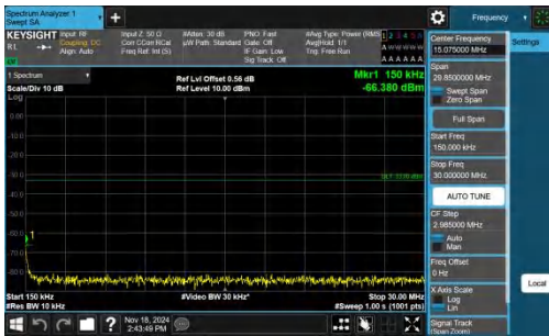
Band66-3MHz-QPSK-132657-1RB#0-0.15~30-PASS
