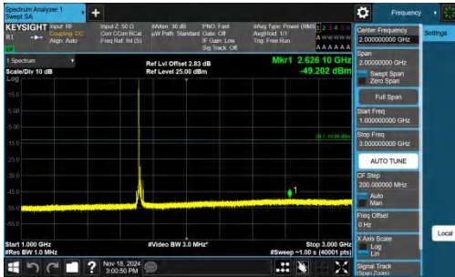
Band66-15MHz-QPSK-132047-1RB#0-1000~3000-PASS
