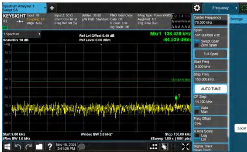
Band66-3MHz-QPSK-131987-1RB#14-0.009~0.15-PASS
