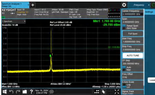
Band66-5MHz-QPSK-132647-1RB#0-1000~3000-PASS
