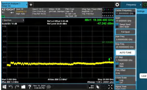
Band66-20MHz-QPSK-132322-1RB#0-3000~20000-PASS
