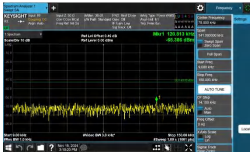
Band66-20MHz-QPSK-132572-1RB#99-0.009~0.15-PASS
