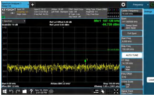
Band66-5MHz-QPSK-132647-1RB#24-0.009~0.15-PASS
