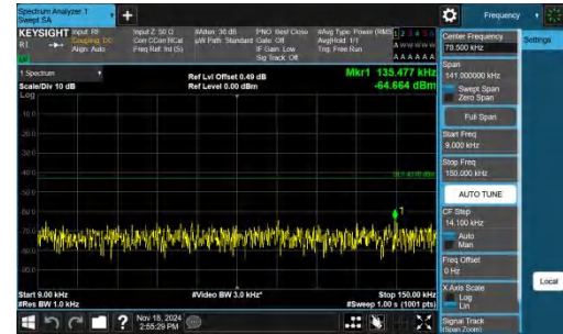
Band66-10MHz-QPSK-132322-1RB#0-0.009~0.15-PASS
