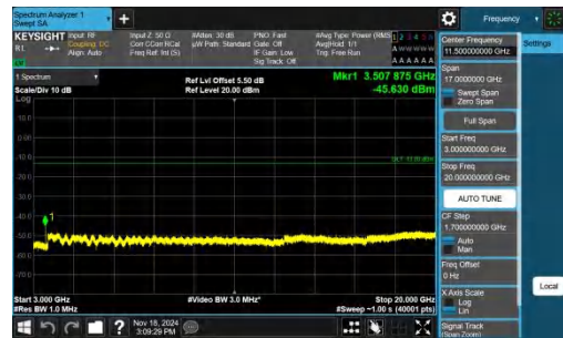
Band66-20MHz-QPSK-132322-1RB#99-3000~20000-PASS
