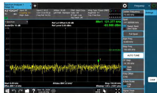
Band66-15MHz-QPSK-132047-1RB#0-0.009~0.15-PASS
