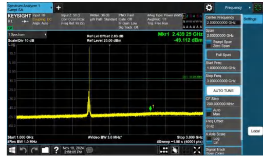
Band66-10MHz-QPSK-132622-1RB#49-1000~3000-PASS
