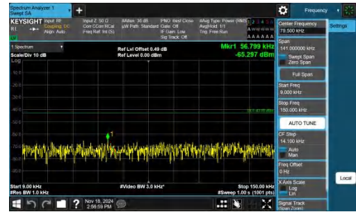
Band66-10MHz-QPSK-132622-1RB#0-0.009~0.15-PASS
