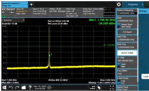
Band66-3MHz-QPSK-132657-1RB#0-1000~3000-PASS
