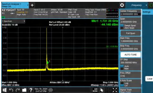
Band66-5MHz-QPSK-131997-1RB#0-1000~3000-PASS
