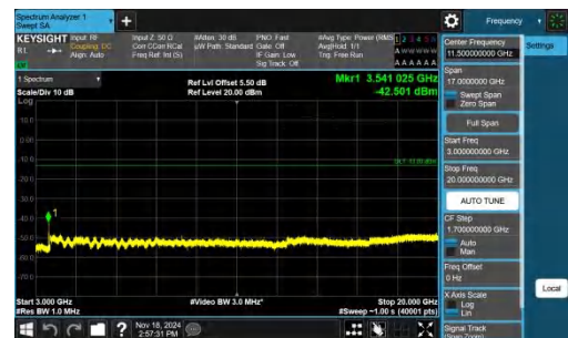
Band66-10MHz-QPSK-132622-1RB#0-3000~20000-PASS
