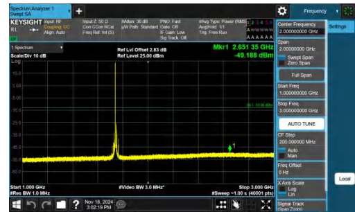
Band66-15MHz-QPSK-132322-1RB#0-1000~3000-PASS
