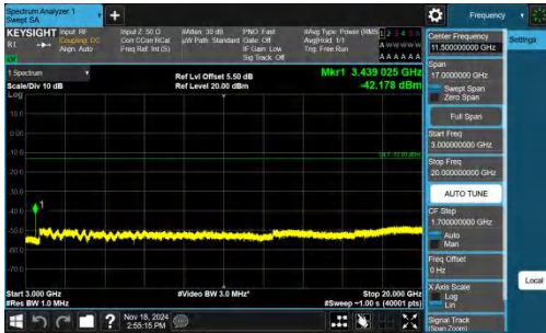
Band66-10MHz-QPSK-132022-1RB#49-3000~20000-PASS
