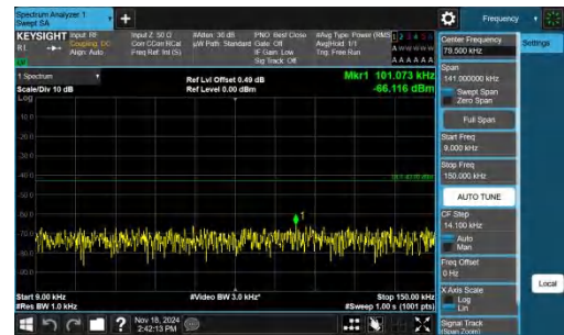
Band66-3MHz-QPSK-132322-1RB#0-0.009~0.15-PASS
