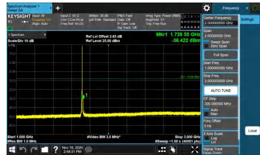
Band66-5MHz-QPSK-131997-1RB#24-1000~3000-PASS
