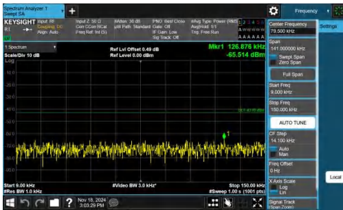
Band66-15MHz-QPSK-132597-1RB#0-0.009~0.15-PASS
