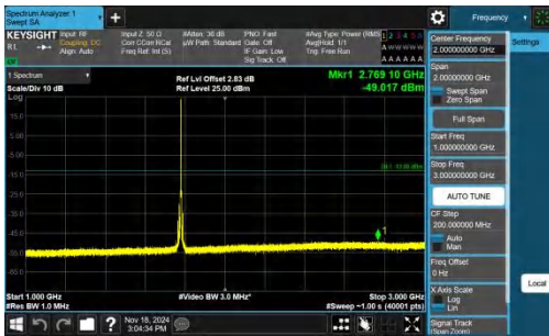
Band66-15MHz-QPSK-132597-1RB#74-1000~3000-PASS
