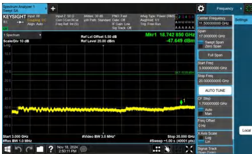
Band66-5MHz-QPSK-132322-1RB#24-3000~20000-PASS
