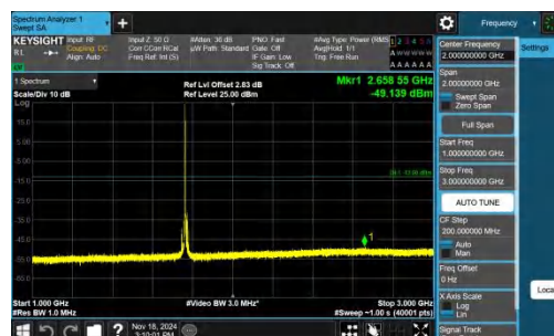
Band66-20MHz-QPSK-132572-1RB#0-1000~3000-PASS
