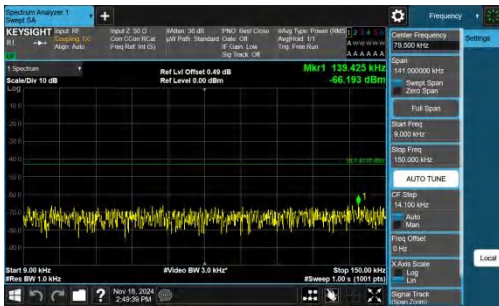
Band66-5MHz-QPSK-132322-1RB#24-0.009~0.15-PASS
