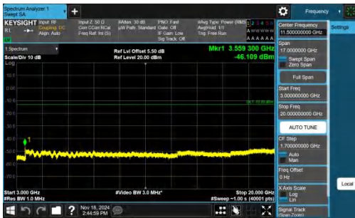
Band66-3MHz-QPSK-132657-1RB#14-3000~20000-PASS
