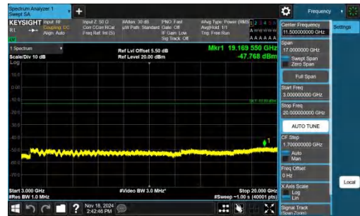
Band66-3MHz-QPSK-132322-1RB#0-3000~20000-PASS
