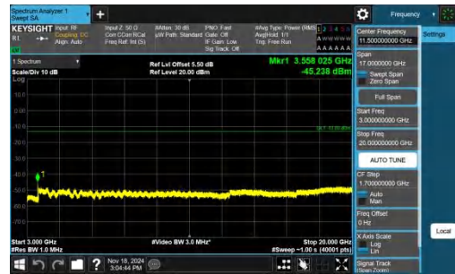
Band66-15MHz-QPSK-132597-1RB#74-3000~20000-PASS
