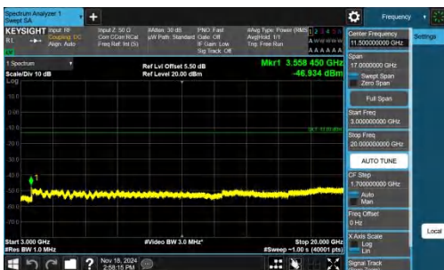
Band66-10MHz-QPSK-132622-1RB#49-3000~20000-PASS
