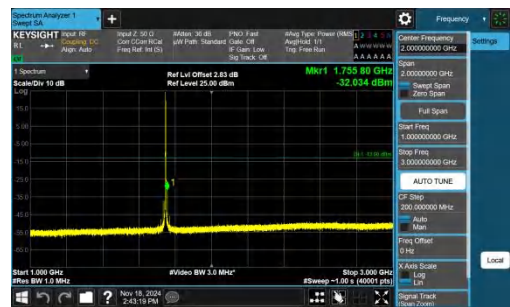
Band66-3MHz-QPSK-132322-1RB#14-1000~3000-PASS
