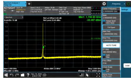
Band66-5MHz-QPSK-132322-1RB#24-1000~3000-PASS
