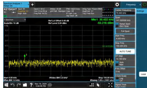
Band66-20MHz-QPSK-132322-1RB#99-0.009~0.15-PASS
