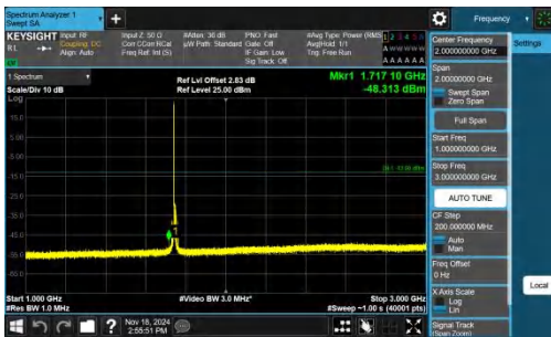
Band66-10MHz-QPSK-132322-1RB#0-1000~3000-PASS
