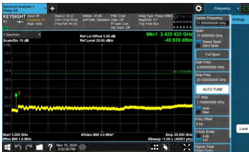
Band66-3MHz-QPSK-131987-1RB#14-3000~20000-PASS
