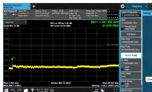
Band66-20MHz-QPSK-132572-1RB#0-3000~20000-PASS
