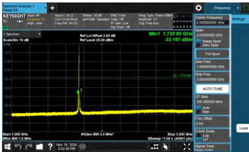
Band66-3MHz-QPSK-132322-1RB#0-1000~3000-PASS
