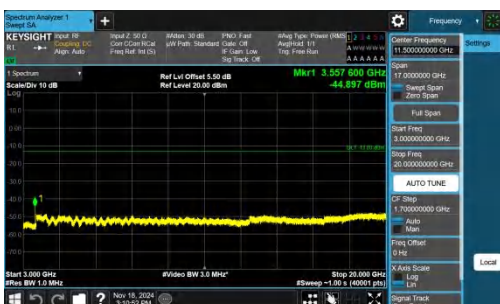
Band66-20MHz-QPSK-132572-1RB#99-3000~20000-PASS
