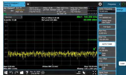
Band66-5MHz-QPSK-132647-1RB#0-0.009~0.15-PASS
