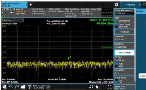
Band66-10MHz-QPSK-132622-1RB#49-0.009~0.15-PASS
