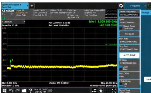
Band66-5MHz-QPSK-132647-1RB#24-3000~20000-PASS
