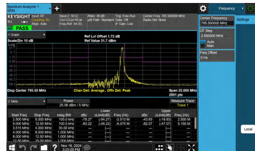
NTNV-Band14-5MHz-16QAM-23355-1RB#24--5.00--2.50-PASS
