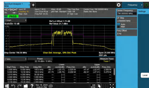
NTNV-Band14-5MHz-16QAM-23305-25RB#0--2.50-2.50-PASS
