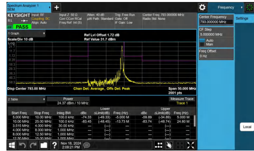
NTNV-Band14-10MHz-16QAM-23330-1RB#49-10.00-25.00-PASS
