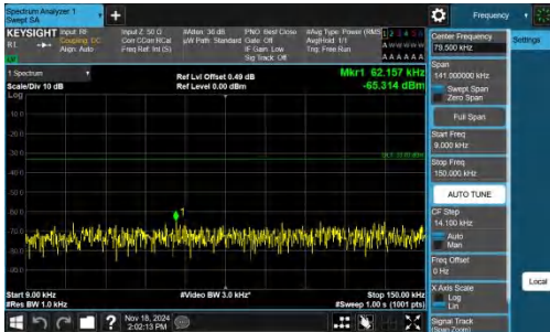
Band14-5MHz-QPSK-23305-1RB#0-0.009~0.15-PASS
