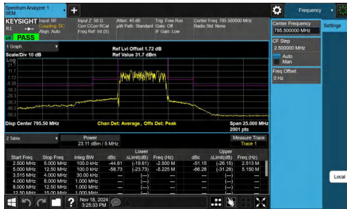
NTNV-Band14-5MHz-QPSK-23355-25RB#0-2.50-5.00-PASS
