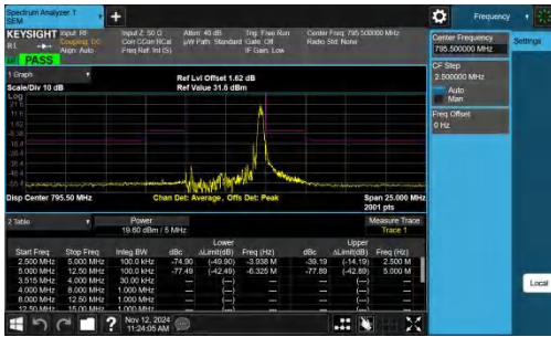
NTNV-Band14-5MHz-16QAM-23355-1RB#24-2.50-5.00-PASS
