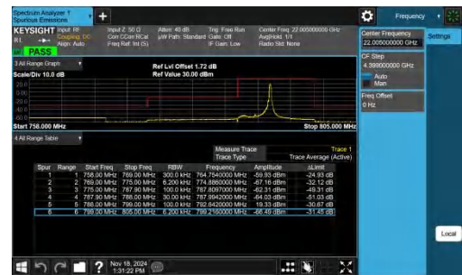
Band14-5MHz-QPSK-23305-1RB#24-PASS
