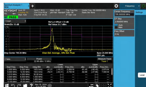
NTNV-Band14-5MHz-64QAM-23355-1RB#0--12.50--5.00-PASS
