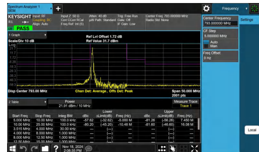
NTNV-Band14-10MHz-64QAM-23330-1RB#0-10.00-25.00-PASS
