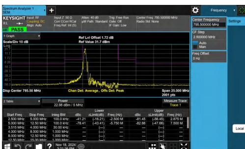
NTNV-Band14-5MHz-64QAM-23355-1RB#0-2.50-5.00-PASS
