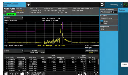
NTNV-Band14-5MHz-16QAM-23355-1RB#24--12.50--5.00-PASS
