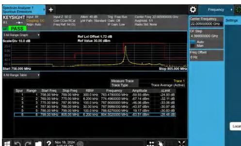
Band14-10MHz-QPSK-23330-1RB#0-PASS
