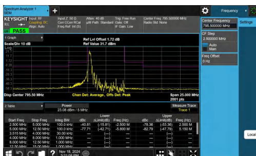
NTNV-Band14-5MHz-QPSK-23355-1RB#0--12.50--5.00-PASS
