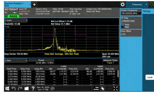
NTNV-Band14-5MHz-16QAM-23355-1RB#0--12.50--5.00-PASS
