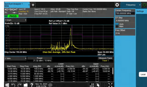
NTNV-Band14-10MHz-QPSK-23330-1RB#49--5.00-5.00-PASS
