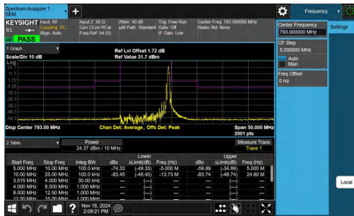
NTNV-Band14-10MHz-16QAM-23330-1RB#49--10.00--5.00-PASS
