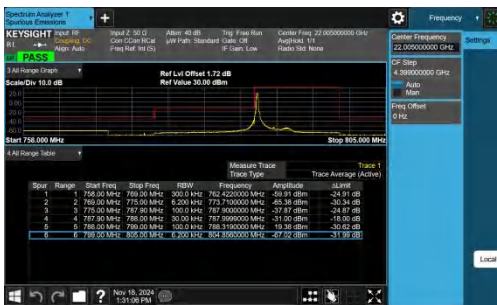
Band14-5MHz-QPSK-23305-1RB#0-PASS
