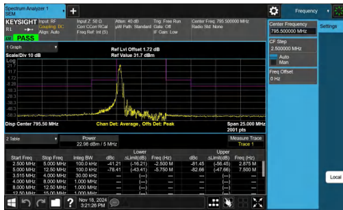
NTNV-Band14-5MHz-64QAM-23355-1RB#0-5.00-12.50-PASS
