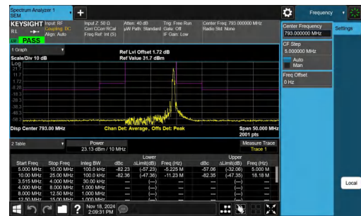
NTNV-Band14-10MHz-64QAM-23330-1RB#49--5.00-5.00-PASS
