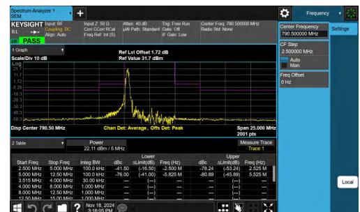
NTNV-Band14-5MHz-16QAM-23305-1RB#0-2.50-5.00-PASS
