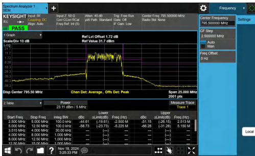
NTNV-Band14-5MHz-QPSK-23355-25RB#0-5.00-12.50-PASS
