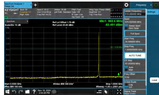
Band14-5MHz-QPSK-23330-1RB#24-30~1000-PASS
