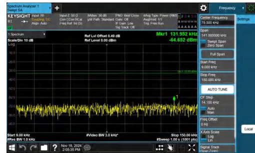
Band14-5MHz-QPSK-23355-1RB#24-0.009~0.15-PASS
