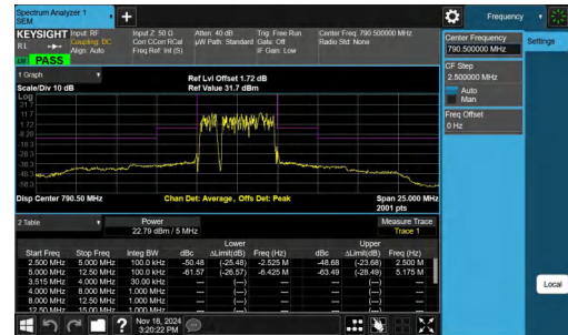
NTNV-Band14-5MHz-QPSK-23305-25RB#0-5.00-12.50-PASS
