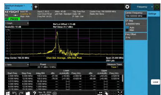
NTNV-Band14-5MHz-16QAM-23305-1RB#0-5.00-12.50-PASS
