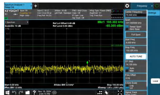
Band14-5MHz-QPSK-23330-1RB#24-0.009~0.15-PASS
