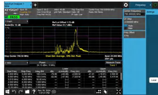
NTNV-Band14-5MHz-QPSK-23305-1RB#24--2.50-2.50-PASS
