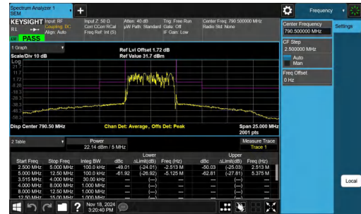
NTNV-Band14-5MHz-64QAM-23305-25RB#0-2.50-5.00-PASS
