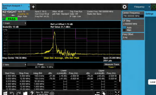
NTNV-Band14-5MHz-16QAM-23305-1RB#0--12.50--5.00-PASS
