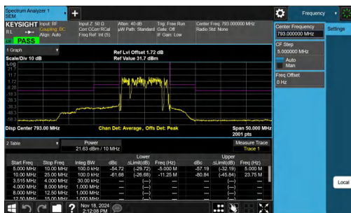
NTNV-Band14-10MHz-QPSK-23330-50RB#0--5.00-5.00-PASS
