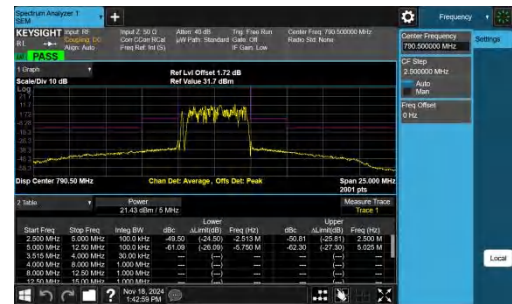
NTNV-Band14-5MHz-64QAM-23305-25RB#0--2.50-2.50-PASS
