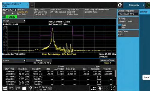
NTNV-Band14-5MHz-QPSK-23305-1RB#0-5.00-12.50-PASS
