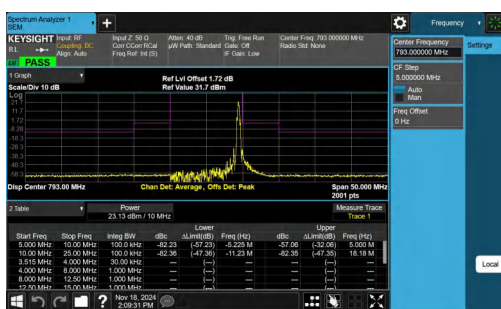
NTNV-Band14-10MHz-64QAM-23330-1RB#49--25.00--10.00-PASS S
