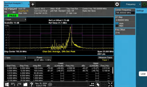
NTNV-Band14-5MHz-QPSK-23355-1RB#24--12.50--5.00-PASS
