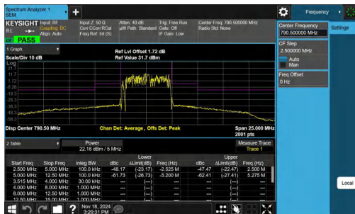
NTNV-Band14-5MHz-16QAM-23305-25RB#0--5.00--2.50-PASS
