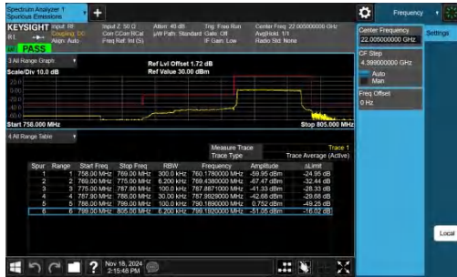
Band14-10MHz-QPSK-23330-50RB#0-PASS
