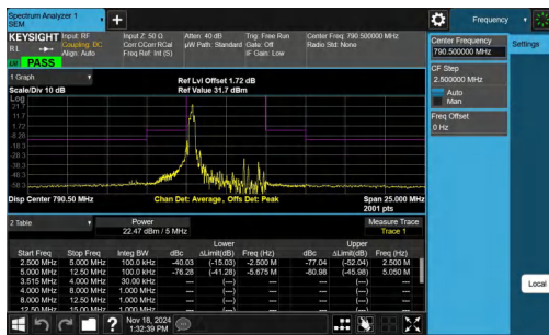
NTNV-Band14-5MHz-QPSK-23305-1RB#0--2.50-2.50-PASS
