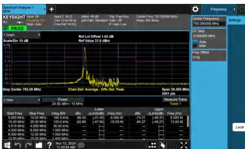
NTNV-Band14-10MHz-QPSK-23330-1RB#0--5.00-5.00-PASS
