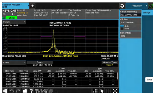
NTNV-Band14-10MHz-16QAM-23330-1RB#0--10.00--5.00-PASS
