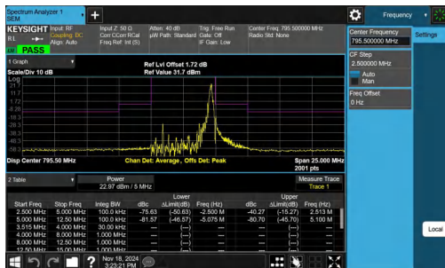
NTNV-Band14-5MHz-QPSK-23355-1RB#24-5.00-12.50-PASS
