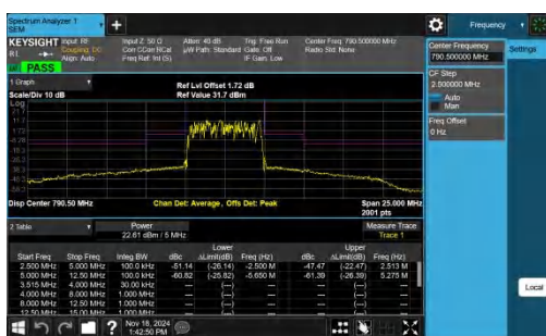
NTNV-Band14-5MHz-16QAM-23305-25RB#0-2.50-5.00-PASS
