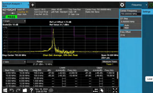
NTNV-Band14-10MHz-64QAM-23330-1RB#0--10.00--5.00-PASS
