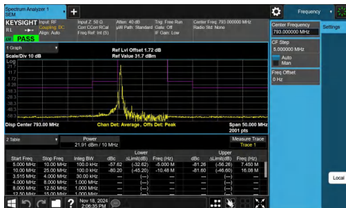
NTNV-Band14-10MHz-64QAM-23330-1RB#0--25.00--10.00-PASS
