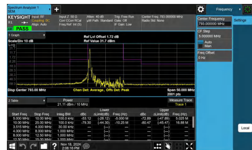
NTNV-Band14-10MHz-QPSK-23330-1RB#0--10.00--5.00-PASS
