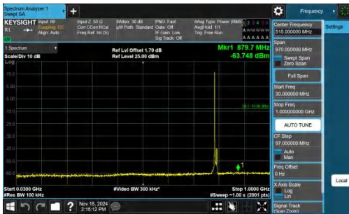
Band14-10MHz-QPSK-23330-1RB#0-30~1000-PASS
