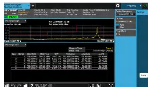
Band14-10MHz-QPSK-23330-1RB#49-PASS
