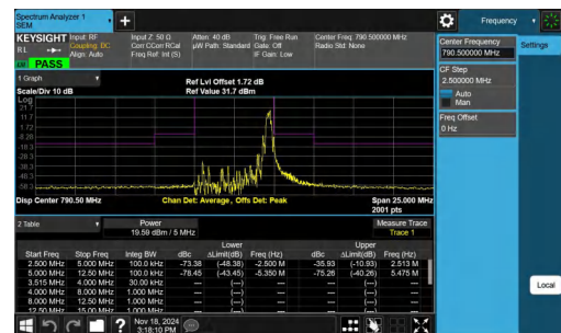
NTNV-Band14-5MHz-QPSK-23305-1RB#24--5.00--2.50-PASS
