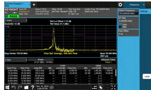
NTNV-Band14-10MHz-64QAM-23330-1RB#0-5.00-10.00-PASS
