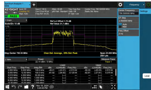
NTNV-Band14-5MHz-64QAM-23305-25RB#0--12.50--5.00-PASS
