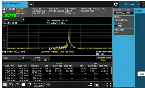
NTNV-Band14-10MHz-16QAM-23330-1RB#49--25.00--10.00-PASS S
