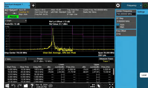
NTNV-Band14-10MHz-16QAM-23330-1RB#0-10.00-25.00-PASS
