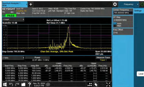
NTNV-Band14-5MHz-QPSK-23355-1RB#24--5.00--2.50-PASS
