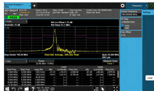
NTNV-Band14-5MHz-64QAM-23355-1RB#0--5.00--2.50-PASS
