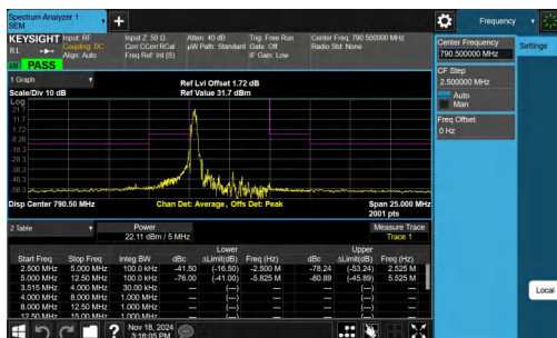
NTNV-Band14-5MHz-16QAM-23305-1RB#0--5.00--2.50-PASS
