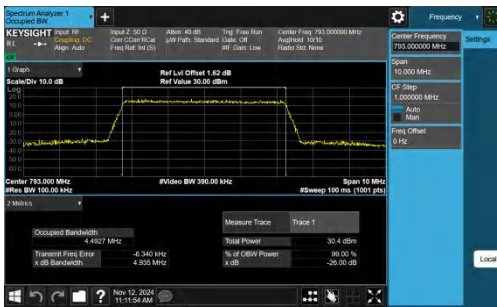
Band14-5MHz-QPSK-23330-25RB#0-PASS
