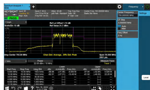
NTNV-Band14-10MHz-16QAM-23330-50RB#0-10.00-25.00-PASS
