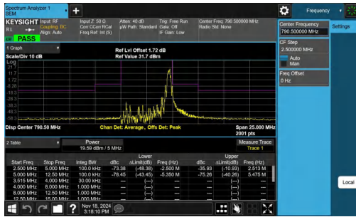
NTNV-Band14-5MHz-QPSK-23305-1RB#24-5.00-12.50-PASS
