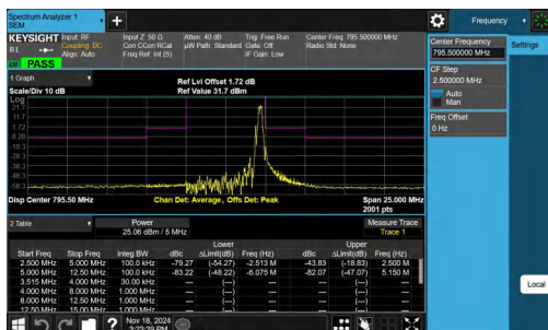
NTNV-Band14-5MHz-16QAM-23355-1RB#24--2.50-2.50-PASS
