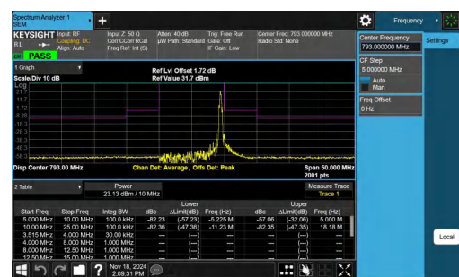
NTNV-Band14-10MHz-64QAM-23330-1RB#49-10.00-25.00-PASS
