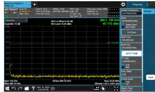
Band14-5MHz-QPSK-23330-1RB#0-0.15~30-PASS
