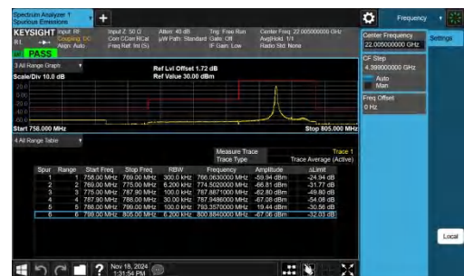
Band14-5MHz-QPSK-23355-1RB#0-PASS
