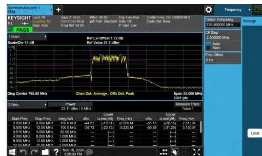
NTNV-Band14-5MHz-QPSK-23355-25RB#0--12.50--5.00-PASS
