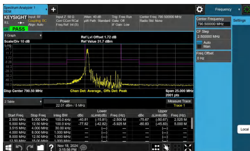
NTNV-Band14-5MHz-QPSK-23305-1RB#0--12.50--5.00-PASS
