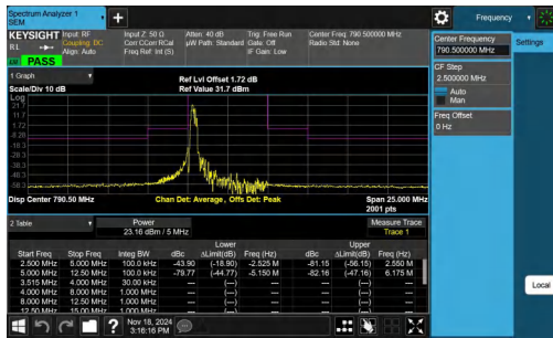
NTNV-Band14-5MHz-64QAM-23305-1RB#0--5.00--2.50-PASS
