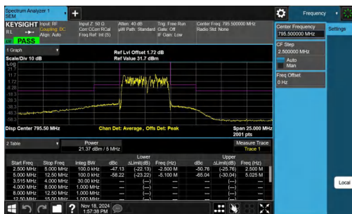
NTNV-Band14-5MHz-64QAM-23355-25RB#0--2.50-2.50-PASS
