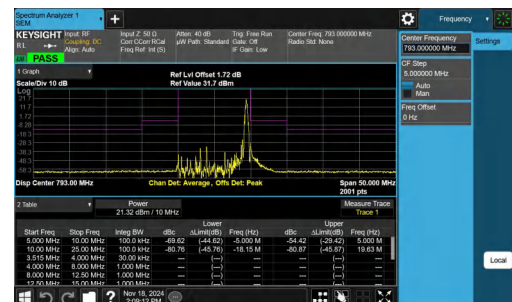
NTNV-Band14-10MHz-QPSK-23330-1RB#49-10.00-25.00-PASS
