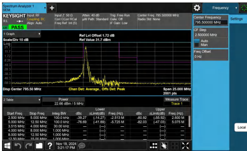
NTNV-Band14-5MHz-16QAM-23355-1RB#0--5.00--2.50-PASS
