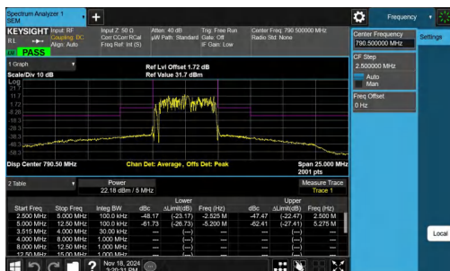
NTNV-Band14-5MHz-16QAM-23305-25RB#0--12.50--5.00-PASS
