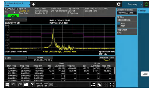
NTNV-Band14-10MHz-QPSK-23330-1RB#0-10.00-25.00-PASS
