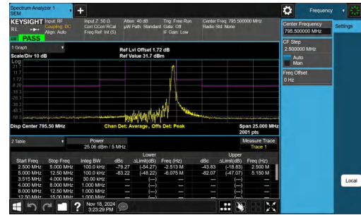
NTNV-Band14-5MHz-16QAM-23355-1RB#24-5.00-12.50-PASS
