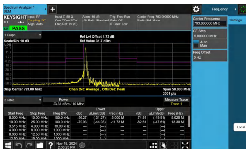
NTNV-Band14-10MHz-16QAM-23330-1RB#0--25.00--10.00-PASS
