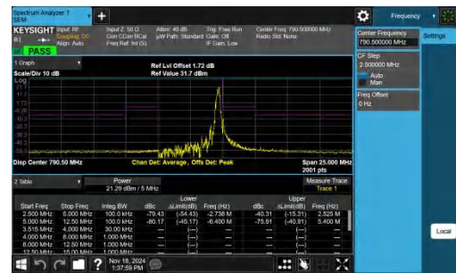
NTNV-Band14-5MHz-64QAM-23305-1RB#24-2.50-5.00-PASS
