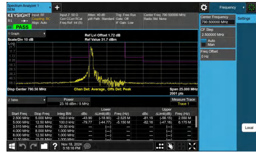
NTNV-Band14-5MHz-64QAM-23305-1RB#0--12.50--5.00-PASS
