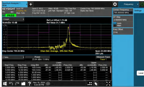
NTNV-Band14-5MHz-64QAM-23355-1RB#24--12.50--5.00-PASS
