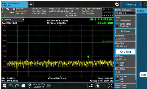
Band14-5MHz-QPSK-23330-1RB#0-0.009~0.15-PASS
