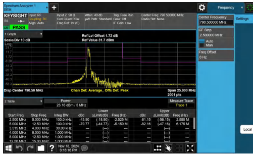
NTNV-Band14-5MHz-64QAM-23305-1RB#0-2.50-5.00-PASS
