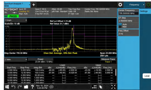
NTNV-Band14-5MHz-64QAM-23355-1RB#24--2.50-2.50-PASS
