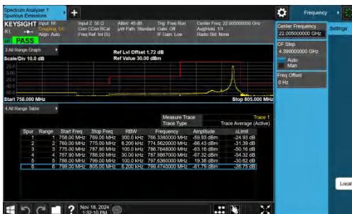
Band14-5MHz-QPSK-23355-1RB#24-PASS
