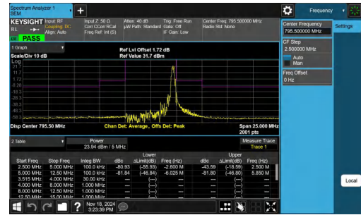
NTNV-Band14-5MHz-64QAM-23355-1RB#24-5.00-12.50-PASS
