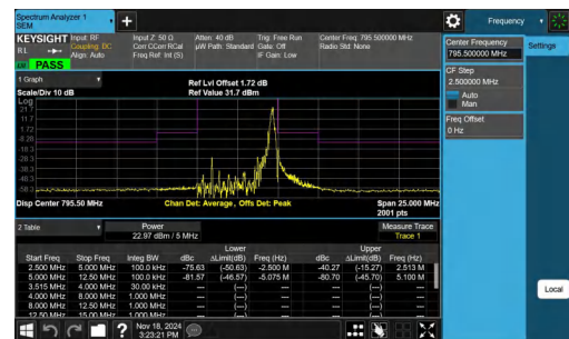
NTNV-Band14-5MHz-QPSK-23355-1RB#24-2.50-5.00-PASS
