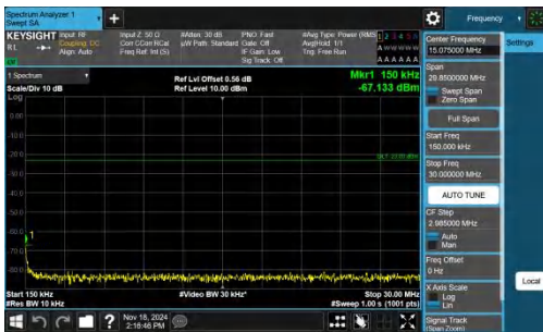
Band14-10MHz-QPSK-23330-1RB#49-0.15~30-PASS
