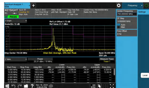
NTNV-Band14-10MHz-16QAM-23330-1RB#0-5.00-10.00-PASS
