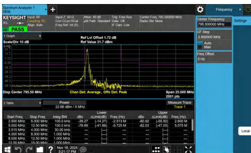
NTNV-Band14-5MHz-16QAM-23355-1RB#0-5.00-12.50-PASS
