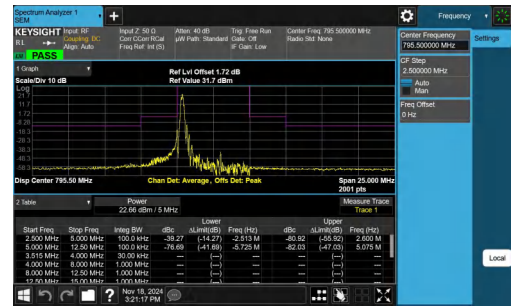
NTNV-Band14-5MHz-16QAM-23355-1RB#0-2.50-5.00-PASS
