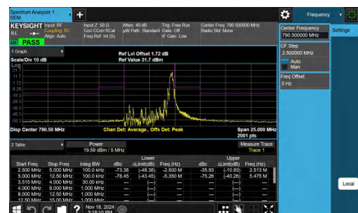
NTNV-Band14-5MHz-QPSK-23305-1RB#24--12.50--5.00-PASS
