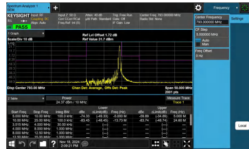
NTNV-Band14-10MHz-16QAM-23330-1RB#49--5.00-5.00-PASS
