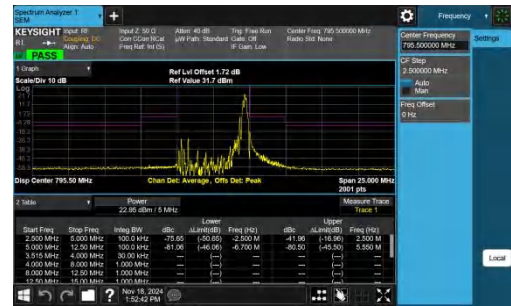
NTNV-Band14-5MHz-QPSK-23355-1RB#24--2.50-2.50-PASS
