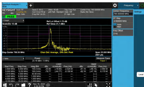
NTNV-Band14-5MHz-64QAM-23305-1RB#0-5.00-12.50-PASS
