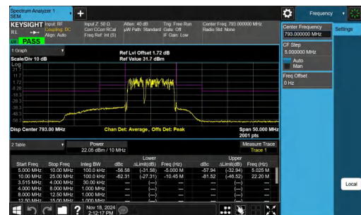
NTNV-Band14-10MHz-16QAM-23330-50RB#0--10.00--5.00-PASS
