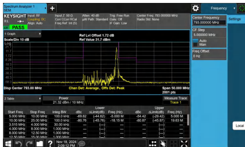
NTNV-Band14-10MHz-QPSK-23330-1RB#49--10.00--5.00-PASS
