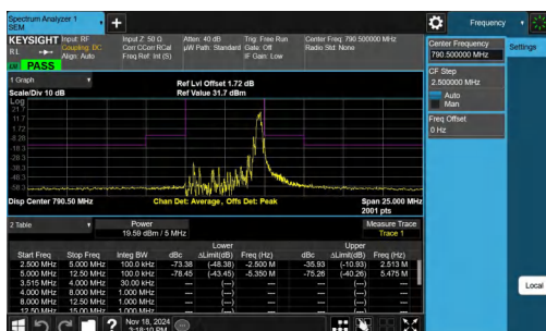
NTNV-Band14-5MHz-QPSK-23305-1RB#24-2.50-5.00-PASS
