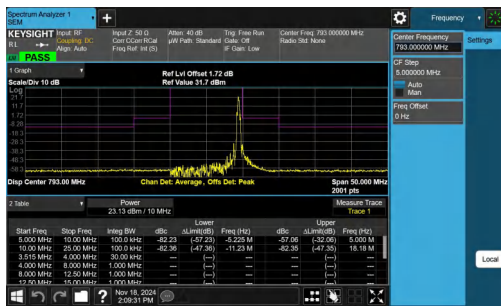
NTNV-Band14-10MHz-64QAM-23330-1RB#49--10.00--5.00-PASS
