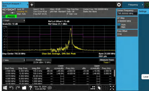
NTNV-Band14-5MHz-64QAM-23355-1RB#24--5.00--2.50-PASS
