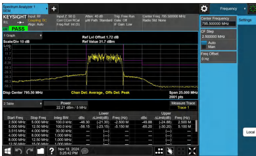
NTNV-Band14-5MHz-16QAM-23355-25RB#0-5.00-12.50-PASS
