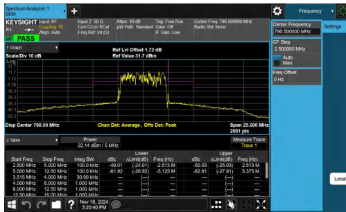
NTNV-Band14-5MHz-64QAM-23305-25RB#0--5.00--2.50-PASS
