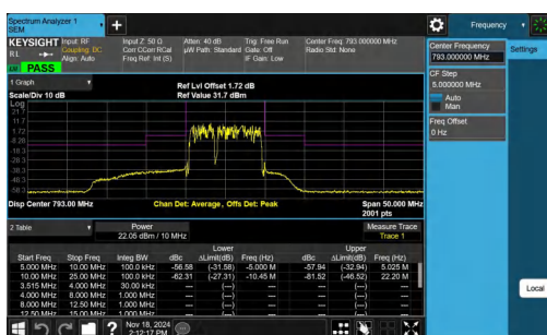
NTNV-Band14-10MHz-16QAM-23330-50RB#0--25.00--10.00-PASS
