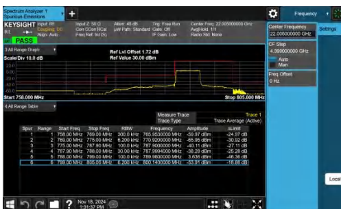
Band14-5MHz-QPSK-23305-25RB#0-PASS
