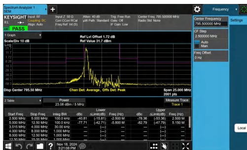
NTNV-Band14-5MHz-QPSK-23355-1RB#0--2.50-2.50-PASS
