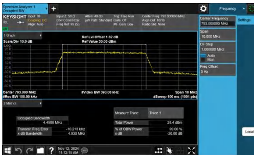
Band14-5MHz-64QAM-23330-25RB#0-PASS
