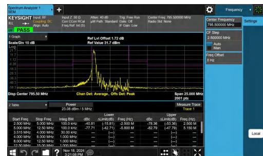
NTNV-Band14-5MHz-QPSK-23355-1RB#0--5.00--2.50-PASS
