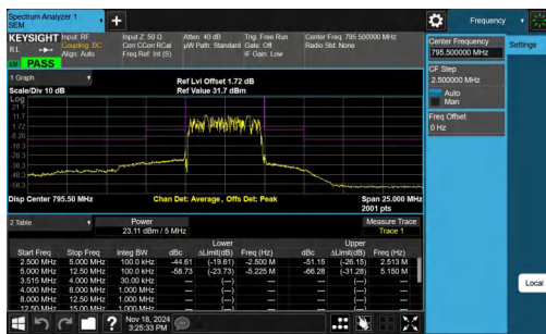
NTNV-Band14-5MHz-QPSK-23355-25RB#0--5.00--2.50-PASS
