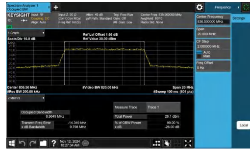
Band5-10MHz-64QAM-20525-50RB#0-PASS
