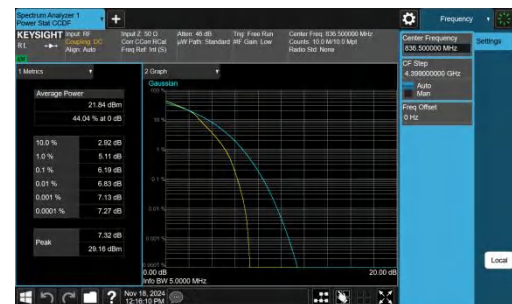
Band5-5MHz-16QAM-20525-25RB#0-PASS
