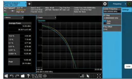
Band5-5MHz-64QAM-20525-25RB#0-PASS
