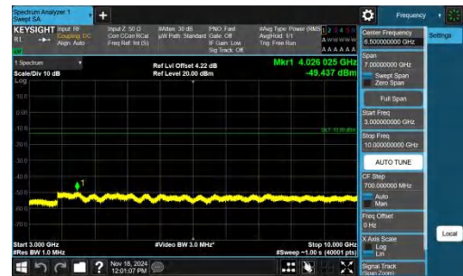
Band5-1.4MHz-QPSK-20643-1RB#5-3000~10000-PASS
