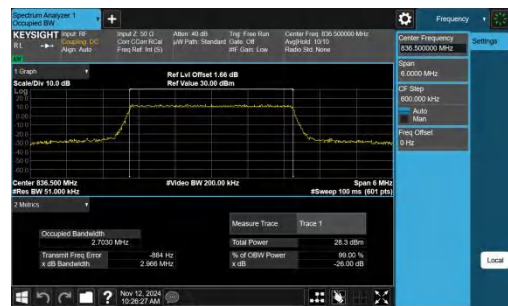
Band5-3MHz-64QAM-20525-15RB#0-PASS
