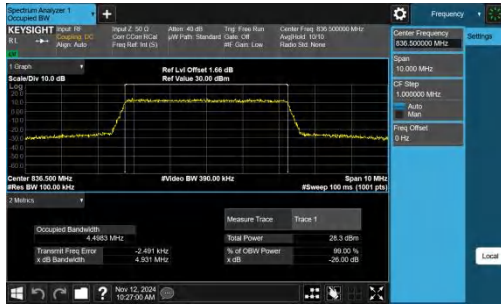
Band5-5MHz-64QAM-20525-25RB#0-PASS
