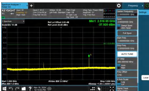
Band5-5MHz-QPSK-20525-1RB#24-1000~3000-PASS
