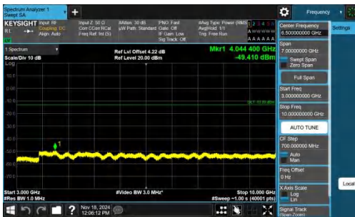
Band5-3MHz-QPSK-20525-1RB#0-3000~10000-PASS
