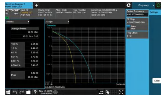
Band5-3MHz-QPSK-20525-15RB#0-PASS
