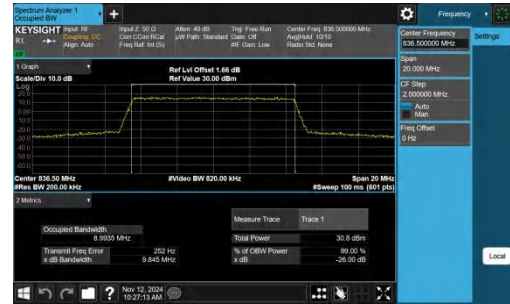
Band5-10MHz-QPSK-20525-50RB#0-PASS
