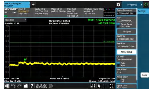
Band5-3MHz-QPSK-20525-1RB#14-3000~10000-PASS
