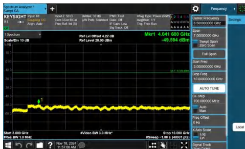
Band5-1.4MHz-QPSK-20407-1RB#0-3000~10000-PASS
