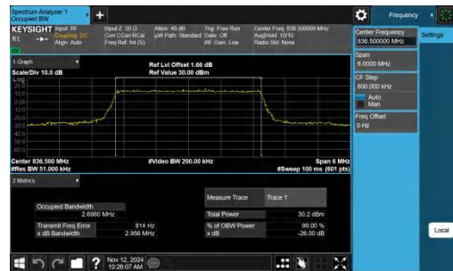
Band5-3MHz-QPSK-20525-15RB#0-PASS
