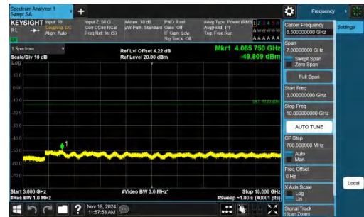
Band5-1.4MHz-QPSK-20407-1RB#5-3000~10000-PASS
