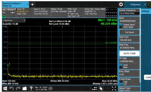
Band5-5MHz-QPSK-20425-1RB#24-0.15~30-PASS
