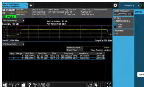
Band5-10MHz-QPSK-20450-50RB#0-PASS
