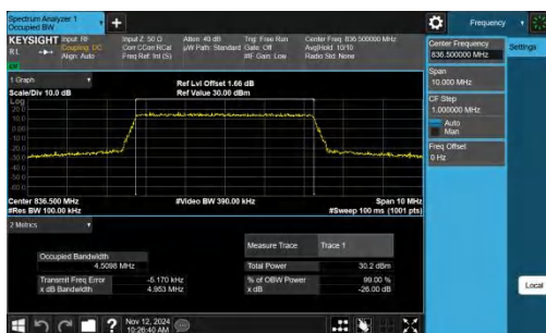
Band5-5MHz-QPSK-20525-25RB#0-PASS
