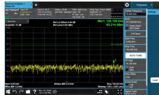
Band5-5MHz-QPSK-20425-1RB#24-0.009~0.15-PASS
