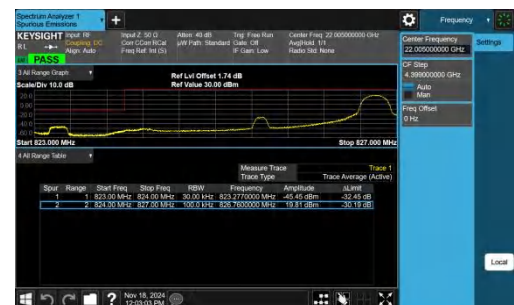
Band5-3MHz-QPSK-20415-1RB#14-PASS
