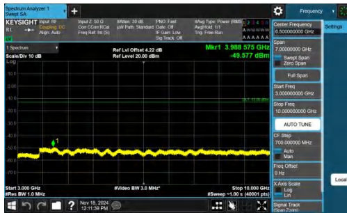
Band5-5MHz-QPSK-20425-1RB#0-3000~10000-PASS
