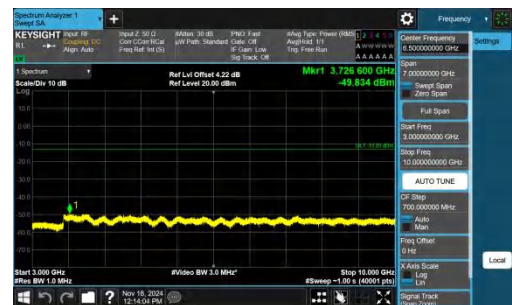
Band5-5MHz-QPSK-20525-1RB#24-3000~10000-PASS
