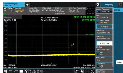
Band5-5MHz-QPSK-20425-1RB#0-1000~3000-PASS
