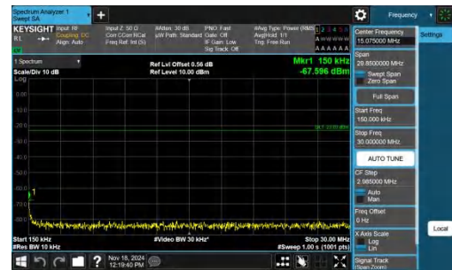
Band5-10MHz-QPSK-20525-1RB#0-0.15~30-PASS
