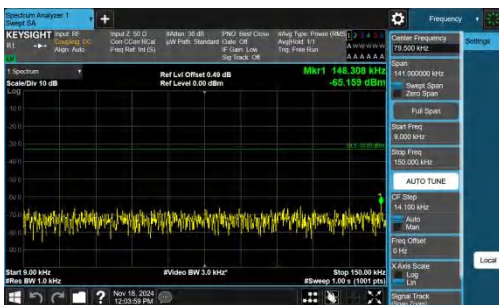
Band5-3MHz-QPSK-20415-1RB#0-0.009~0.15-PASS
