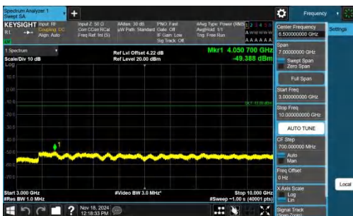
Band5-10MHz-QPSK-20450-1RB#0-3000~10000-PASS
