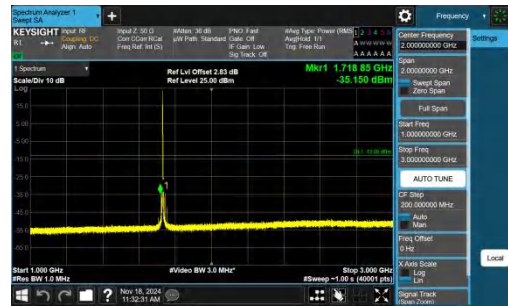
Band4-5MHz-QPSK-20175-1RB#0-1000~3000-PASS
