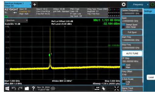
Band4-3MHz-QPSK-20175-1RB#0-1000~3000-PASS
