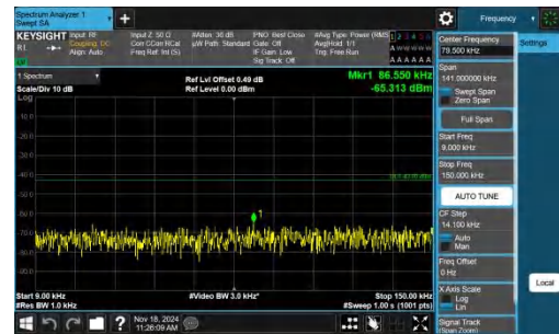
Band4-3MHz-QPSK-20175-1RB#14-0.009~0.15-PASS
