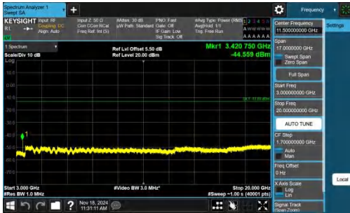
Band4-5MHz-QPSK-19975-1RB#0-3000~20000-PASS
