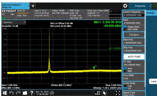
Band4-10MHz-QPSK-20175-1RB#49-1000~3000-PASS
