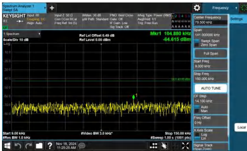
Band4-3MHz-QPSK-20175-1RB#0-0.009~0.15-PASS
