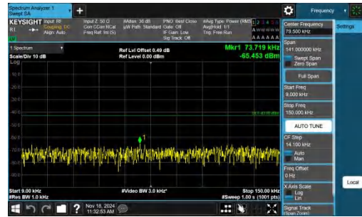
Band4-5MHz-QPSK-20175-1RB#24-0.009~0.15-PASS
