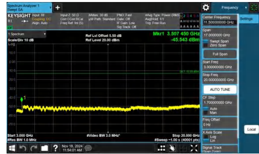
Band4-20MHz-QPSK-20300-1RB#99-3000~20000-PASS
