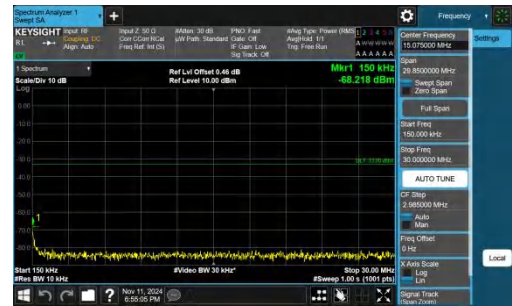
Band2-3MHz-QPSK-18900-1RB#0-0.15~30-PASS
