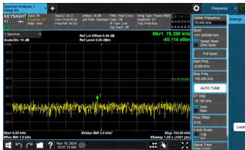
Band2-10MHz-QPSK-18900-1RB#0-0.009~0.15-PASS
