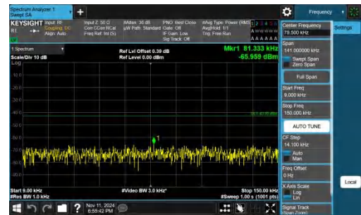
Band2-3MHz-QPSK-18900-1RB#14-0.009~0.15-PASS
