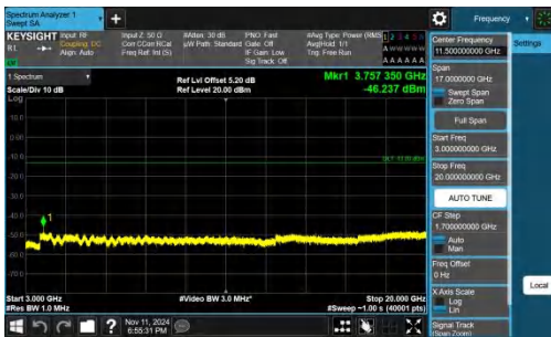
Band2-3MHz-QPSK-18900-1RB#0-3000~20000-PASS
