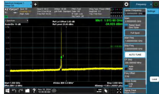
Band2-1.4MHz-QPSK-19193-1RB#5-1000~3000-PASS
