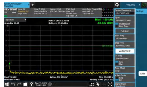
Band2-5MHz-QPSK-18625-1RB#0-0.15~30-PASS
