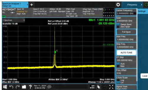
Band2-3MHz-QPSK-18900-1RB#14-1000~3000-PASS
