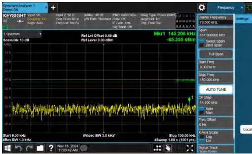
Band2-15MHz-QPSK-18900-1RB#0-0.009~0.15-PASS
