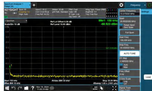
Band2-15MHz-QPSK-19125-1RB#0-0.15~30-PASS
