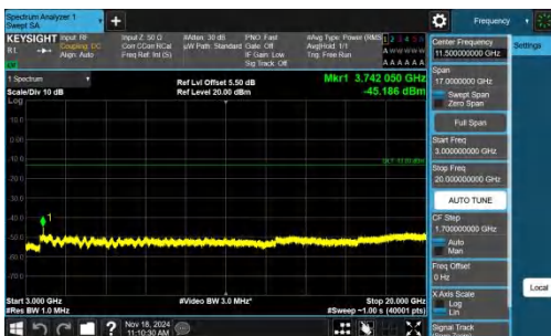
Band2-20MHz-QPSK-18900-1RB#0-3000~20000-PASS
