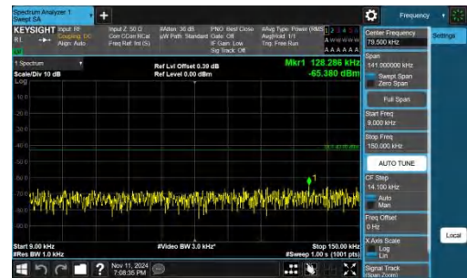
Band2-5MHz-QPSK-19175-1RB#24-0.009~0.15-PASS
