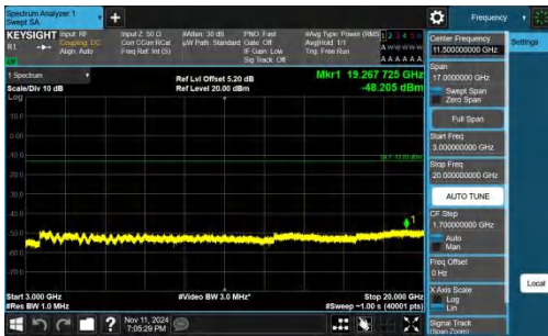
Band2-5MHz-QPSK-18625-1RB#0-3000~20000-PASS
