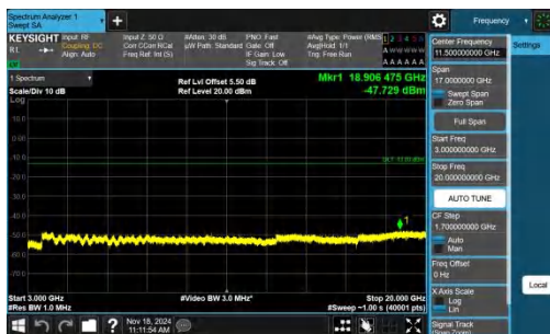
Band2-20MHz-QPSK-19100-1RB#0-3000~20000-PASS
