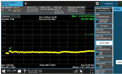
Band2-1.4MHz-QPSK-19193-1RB#5-3000~20000-PASS
