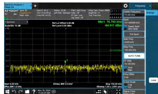
Band2-15MHz-QPSK-18900-1RB#74-0.009~0.15-PASS
