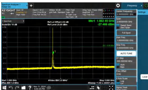
Band2-3MHz-QPSK-18615-1RB#14-1000~3000-PASS
