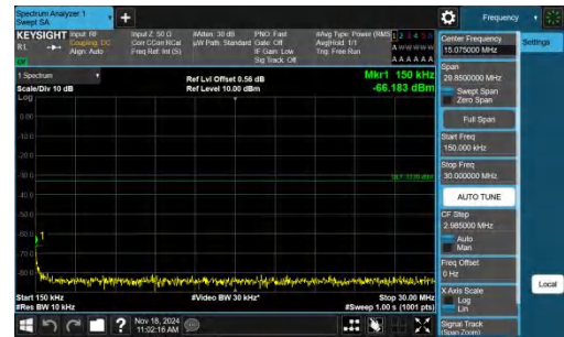
Band2-15MHz-QPSK-18675-1RB#0-0.15~30-PASS
