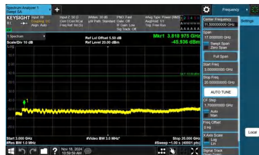
Band2-10MHz-QPSK-19150-1RB#49-3000~20000-PASS
