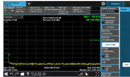
Band2-15MHz-QPSK-18900-1RB#0-0.15~30-PASS
