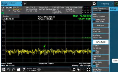
Band2-5MHz-QPSK-19175-1RB#0-0.009~0.15-PASS
