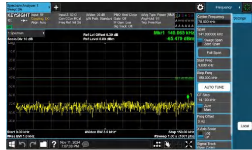
Band2-5MHz-QPSK-18900-1RB#24-0.009~0.15-PASS
