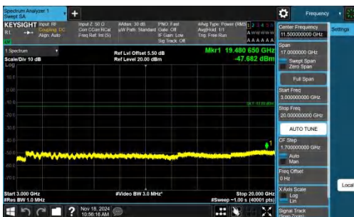
Band2-10MHz-QPSK-18650-1RB#0-3000~20000-PASS
