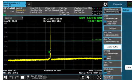
Band2-10MHz-QPSK-19150-1RB#0-1000~3000-PASS
