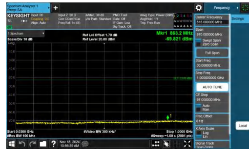
Band2-10MHz-QPSK-18650-1RB#49-30~1000-PASS
