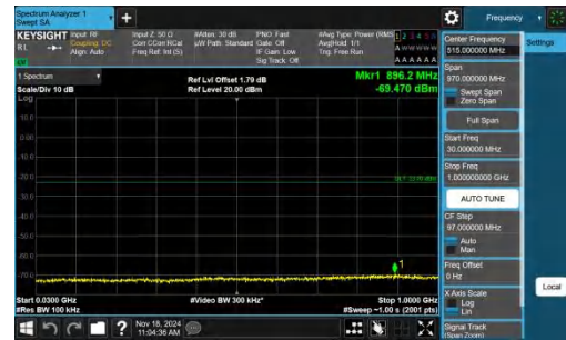
Band2-15MHz-QPSK-18900-1RB#74-30~1000-PASS
