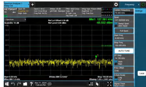
Band2-5MHz-QPSK-18625-1RB#24-0.009~0.15-PASS
