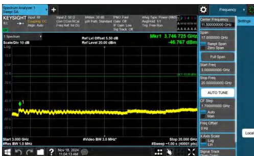
Band2-15MHz-QPSK-18900-1RB#0-3000~20000-PASS
