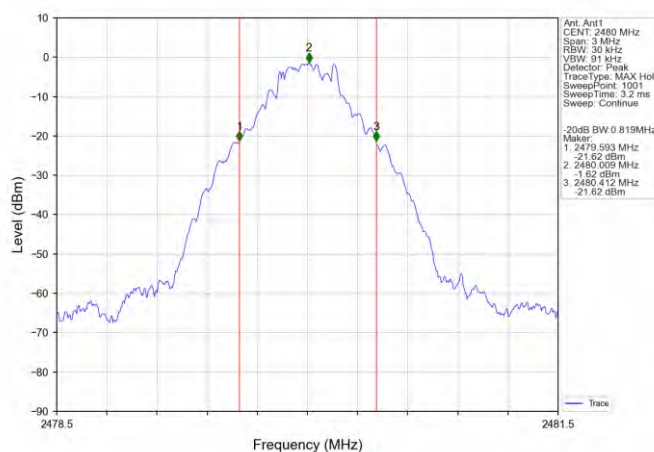
GFSK_DH5_HCH_2480MHz_Ant1_NTNV
