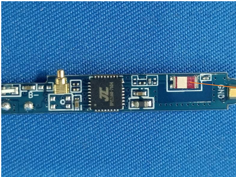
Ceramic antenna
