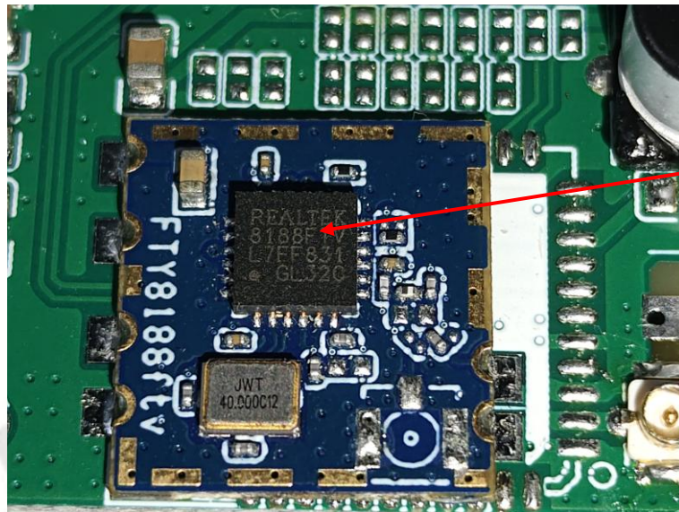
WiFi Chip
