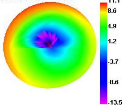
Bluetooth 0 TRP
