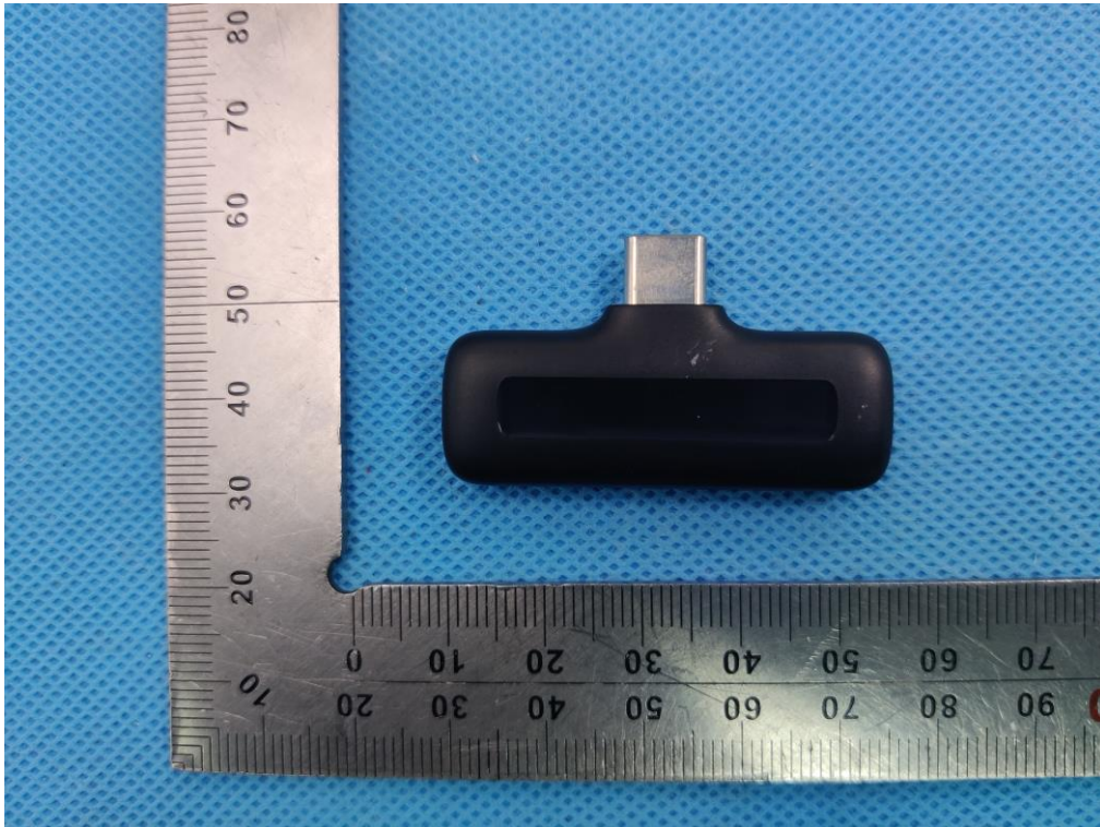
TOP VIEW OF EUT (Receiver)
