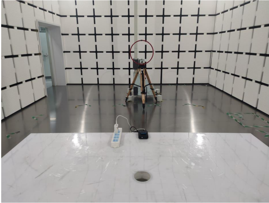
Radiation (9KHz-30MHz)
