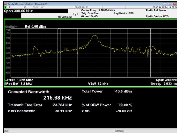
Test Plots of Occupied Bandwidth
