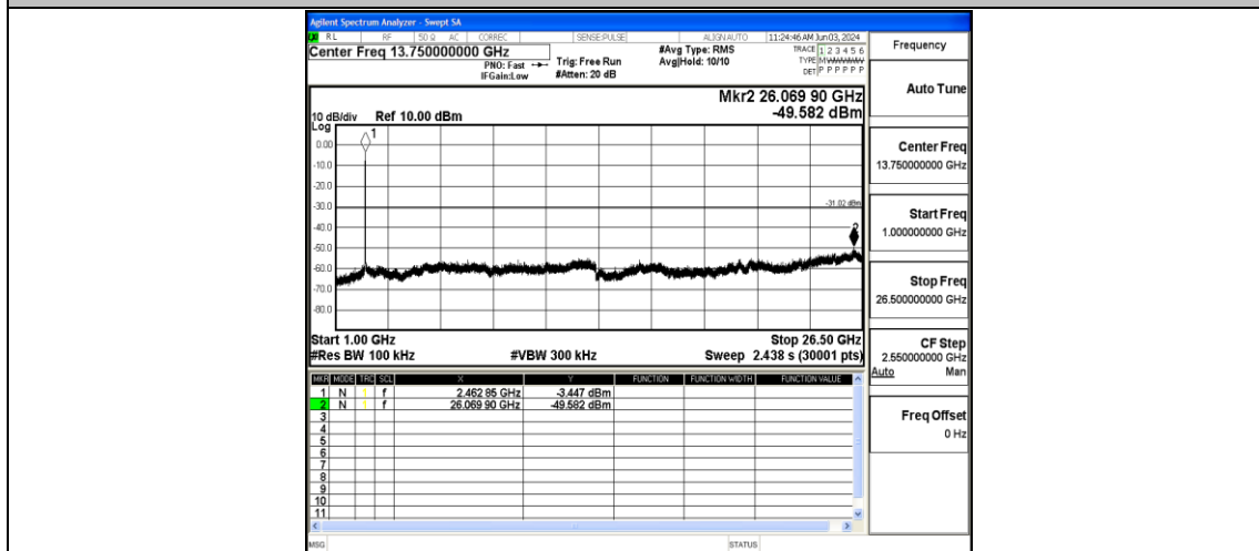
11N20SISO-Ant1-2462-1000~26500-PASS
