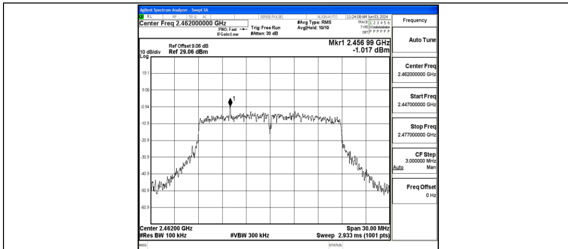
11N20SISO-Ant1-2462-0~Reference-PASS
