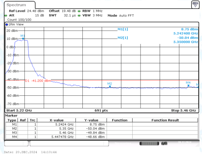
11A-Ant1-5240-PASS
