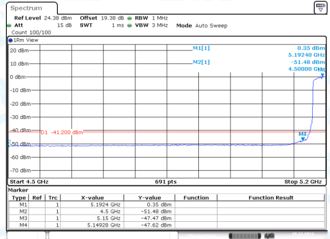
11AX40SISO-Ant1-5190-PASS
