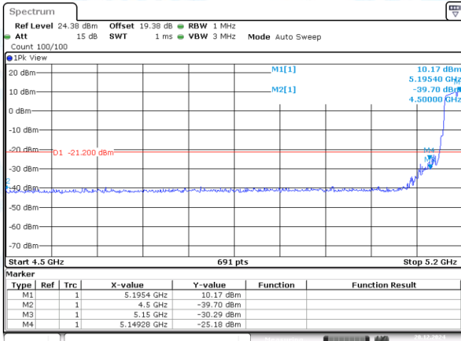
11N40SISO-Ant1-5190-PASS
