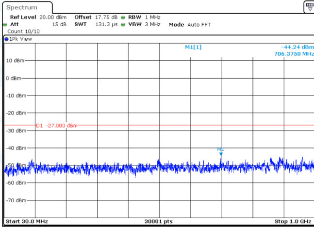
11AC20SISO-Ant1-5240-30~1000-PASS
