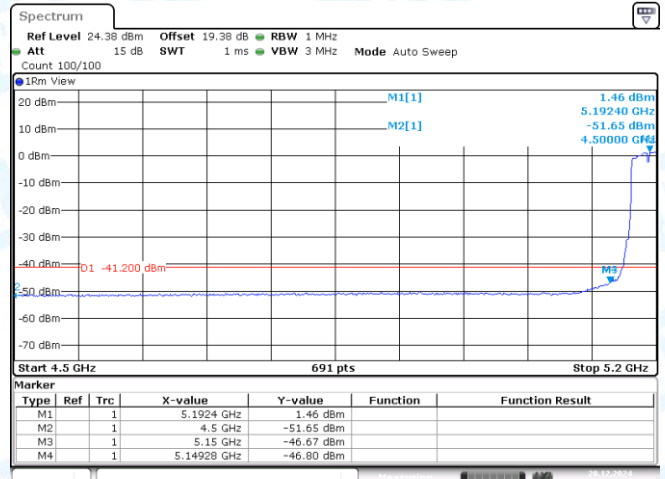
11N40SISO-Ant1-5190-PASS
