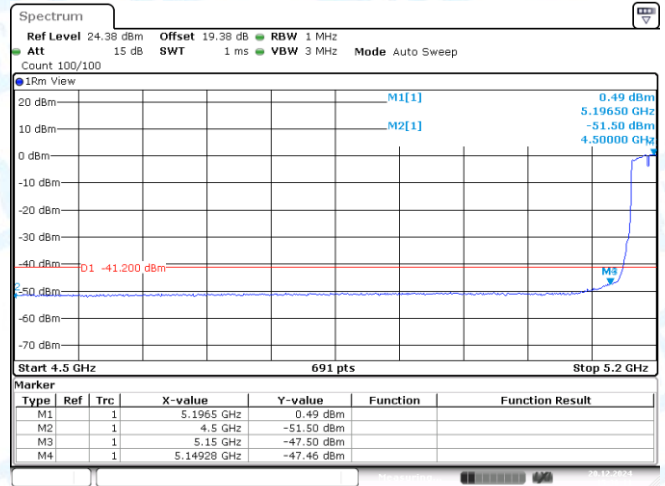
11AC40SISO-Ant1-5190-PASS
