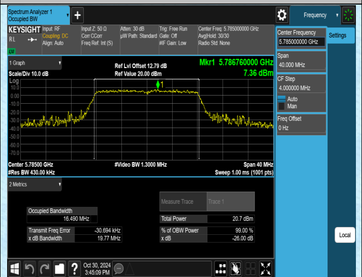
11A-Ant2-5785
