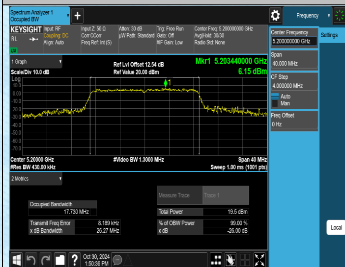
11N20SISO-Ant1-5200
