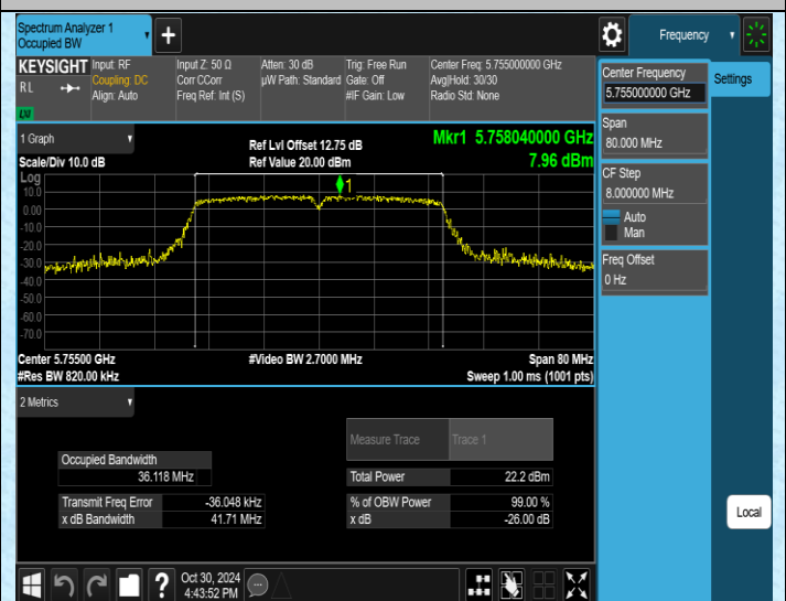
11N40SISO-Ant2-5755
