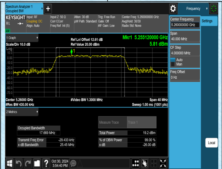
11N20SISO-Ant2-5260
