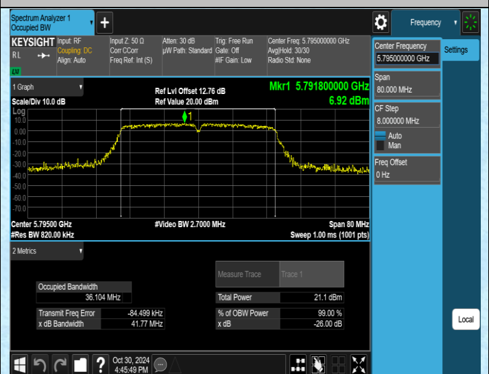
11N40SISO-Ant2-5795
