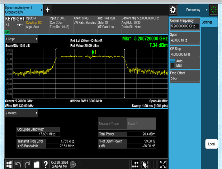
11N20SISO-Ant2-5200
