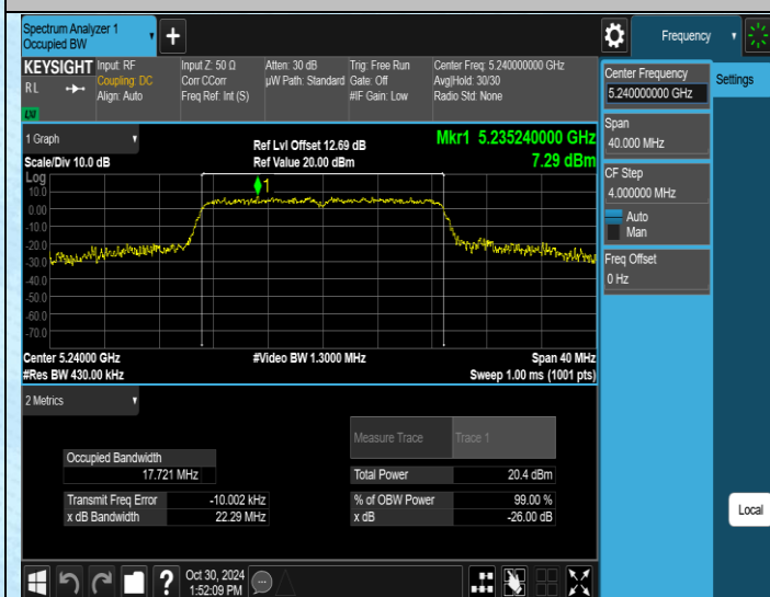
11N20SISO-Ant1-5240
