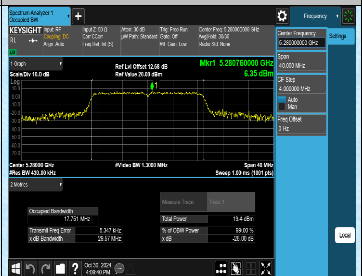
11N20SISO-Ant2-5280
