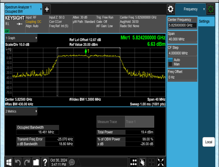
11A-Ant2-5825
