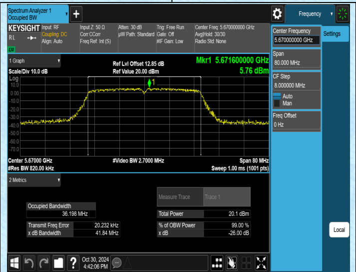
11N40SISO-Ant2-5670
