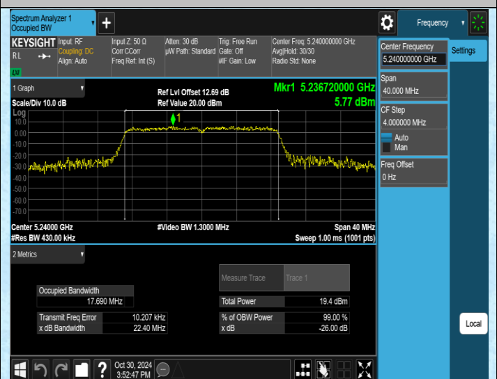
11N20SISO-Ant2-5240
