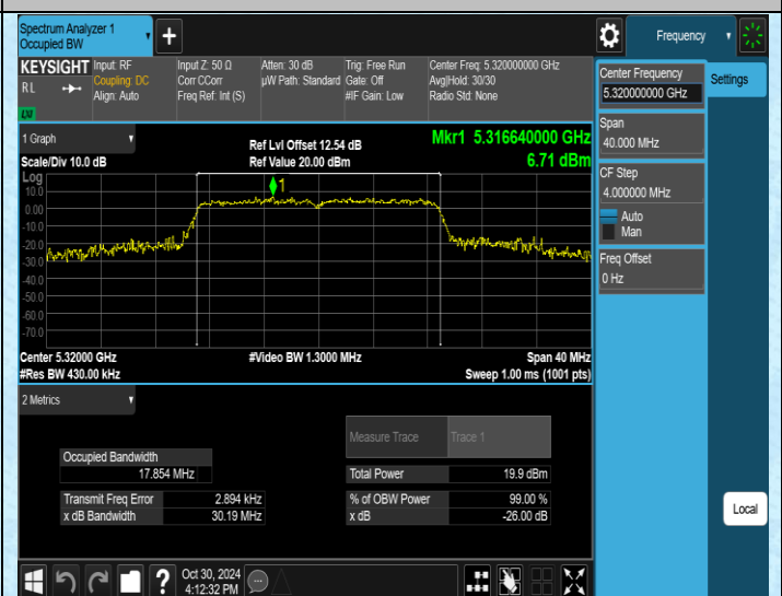
11N20SISO-Ant2-5320
