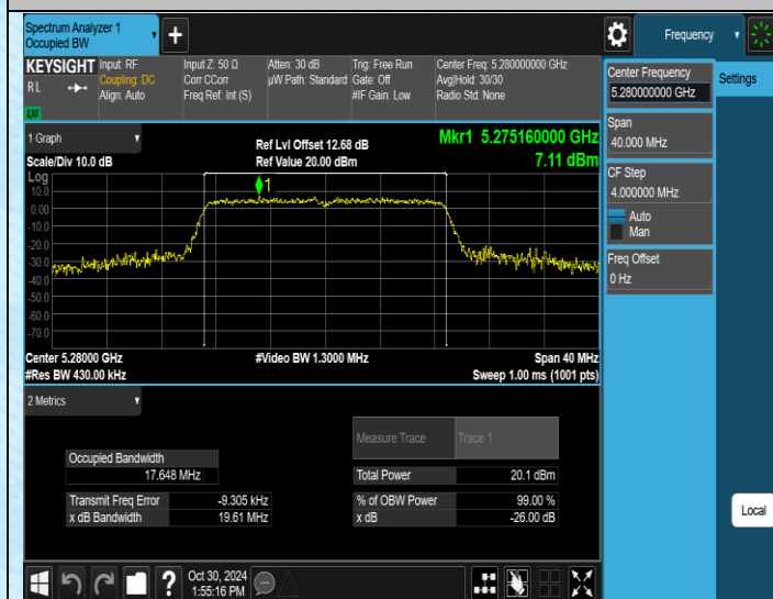
11N20SISO-Ant1-5280
