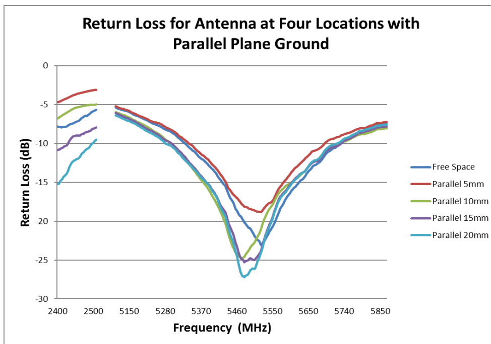
FIGURE 7.1.2 RETURN LOSS OF ANTENNA AT 2.4/5GHZ AT FOUR LOCATIONS WITH PARALLEL PLANE GROUND ON A REFERENCE PCB FOR CONFIGURE 2
