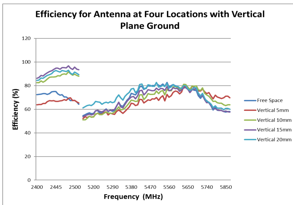
FIGURE 7.2.4 EFFICIENCY OF ANTENNA AT 2.4/5GHZ AT FOUR LOCATIONS WITH VERTICAL PLANE GROUND ON A REFERENCE PCB FOR CONFIGURE 2
