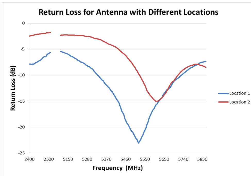
FIGURE 7.3.2 RETURN LOSS OF ANTENNA AT 2.4/5GHZ AT TWO DIFFERENT LOCATIONS FOR CONFIGURE 2
