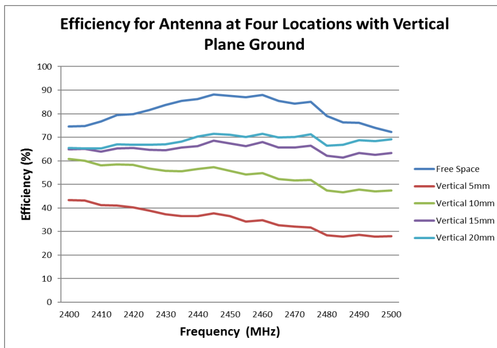
FIGURE 7.2.3 EFFICIENCY OF ANTENNA AT 2.4GHZ AT FOUR LOCATIONS WITH VERTICAL PLANE GROUND ON A REFERENCE PCB FOR CONFIGURE 1
