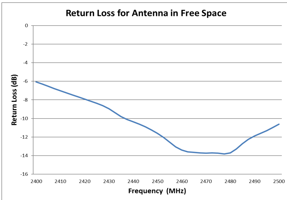
FIGURE 4.3.1 RETURN LOSS OF ANTENNA AT 2.4GHZ IN FREE SPACE FOR CONFIGURE 1
