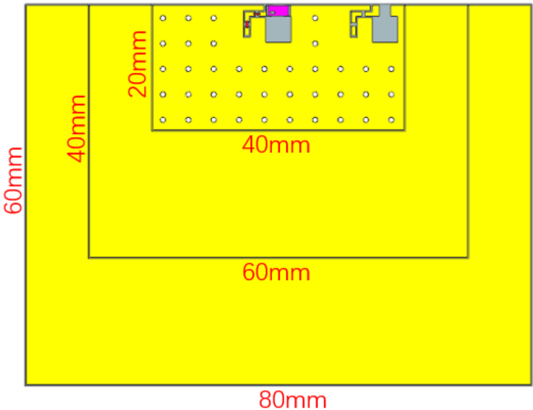
FIGURE 7.4 ANTENNA WITH DIFFERENT PLANE GROUNDS (USING CONFIG1 FOR ILLUSTRATION)
