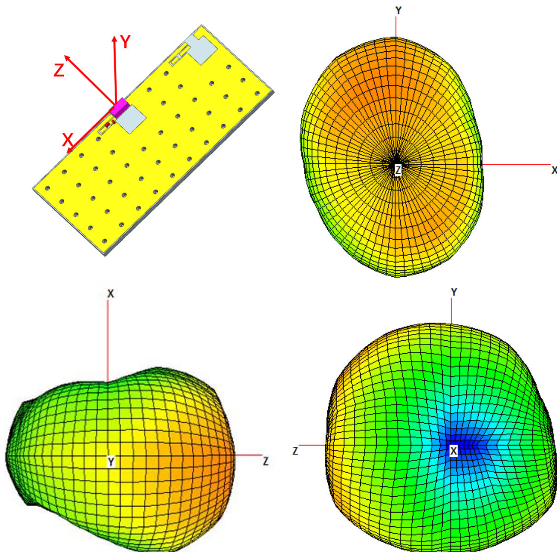
FIGURE 4.6.1 3D RADIATION PATTERN OF ANTENNA AT 2450GHZ IN FREE SPACE FOR CONFIGURE 1
