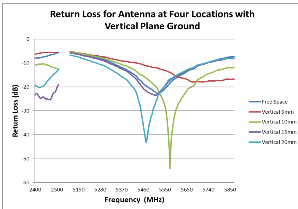
FIGURE 7.2.2 RETURN LOSS OF ANTENNA AT 2.4/5GHZ AT FOUR LOCATIONS WITH VERTICAL PLANE GROUND ON A REFERENCE PCB FOR CONFIGURE 2
