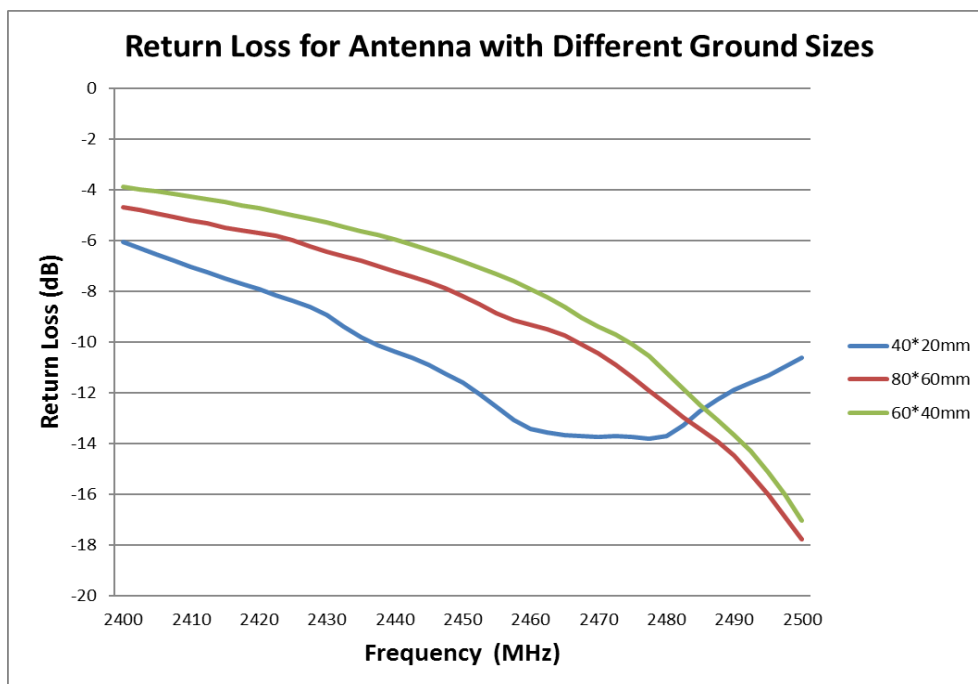
FIGURE 7.4.1 RETURN LOSS OF ANTENNA AT 2.4GHZ WITH DIFFERENT GROUND SIZES FOR CONFIGURE 1
