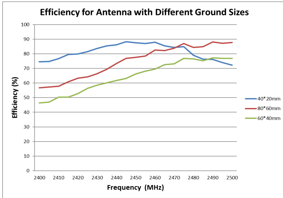
FIGURE 7.4.3 EFFICIENCY OF ANTENNA AT 2.4GHZ WITH DIFFERENT GROUND SIZES FOR CONFIGURE 1
