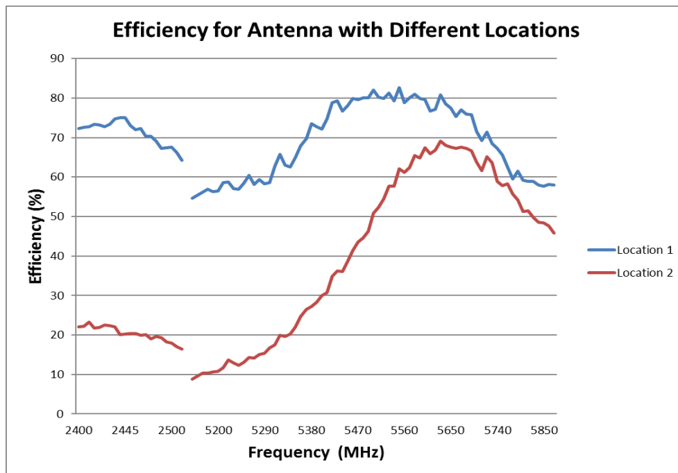
FIGURE 7.3.5 EFFICIENCY OF ANTENNA AT 2.4/5GHZ AT TWO DIFFERENT LOCCATIONS FOR CONFIGURE 2
