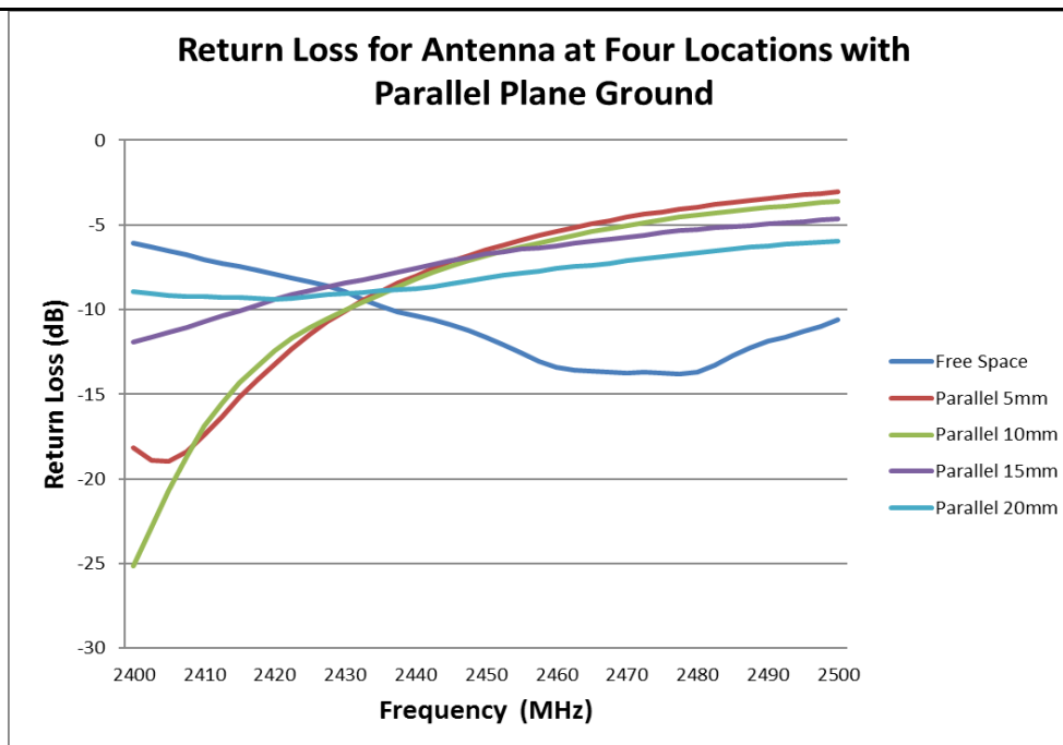
FIGURE 7.1.1 RETURN LOSS OF ANTENNA AT 2.4GHZ AT FOUR LOCATIONS WITH PARALLEL PLANE GROUND ON A REFERENCE PCB FOR CONFIGURE 1
