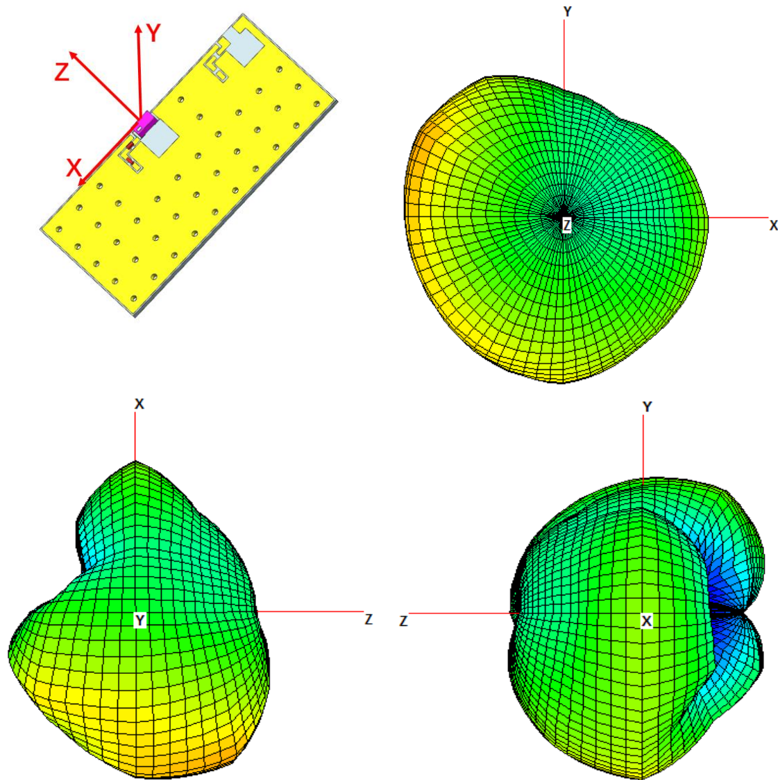
FIGURE 4.6.3 3D RADIATION PATTERN OF ANTENNA AT 5500MHZ IN FREE SPACE FOR CONFIGURE 2
