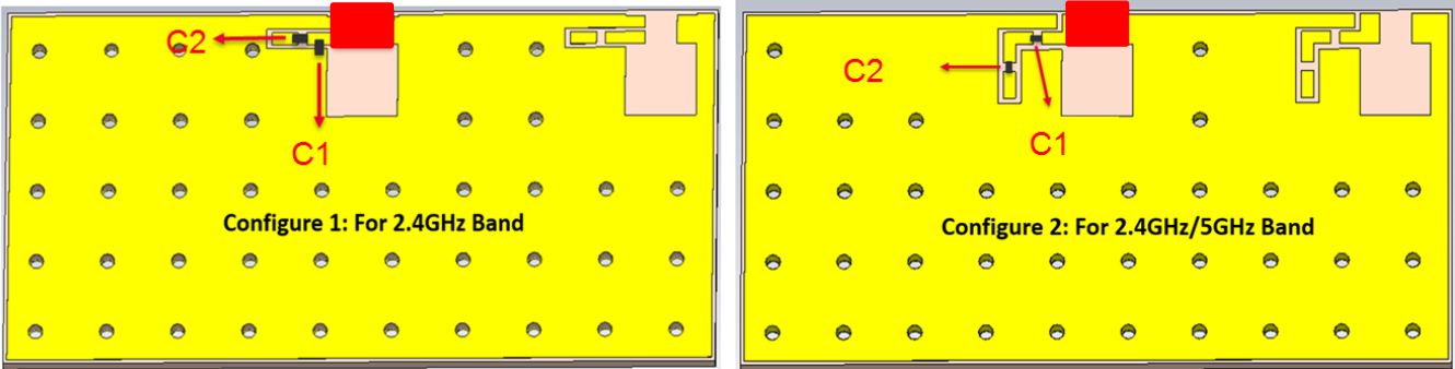
FIGURE 5.1 RECOMMENDED MATCHING CIRCUIT SCHEMATIC FOR CONFIGOURE 1 AND CONFIGURE 2
