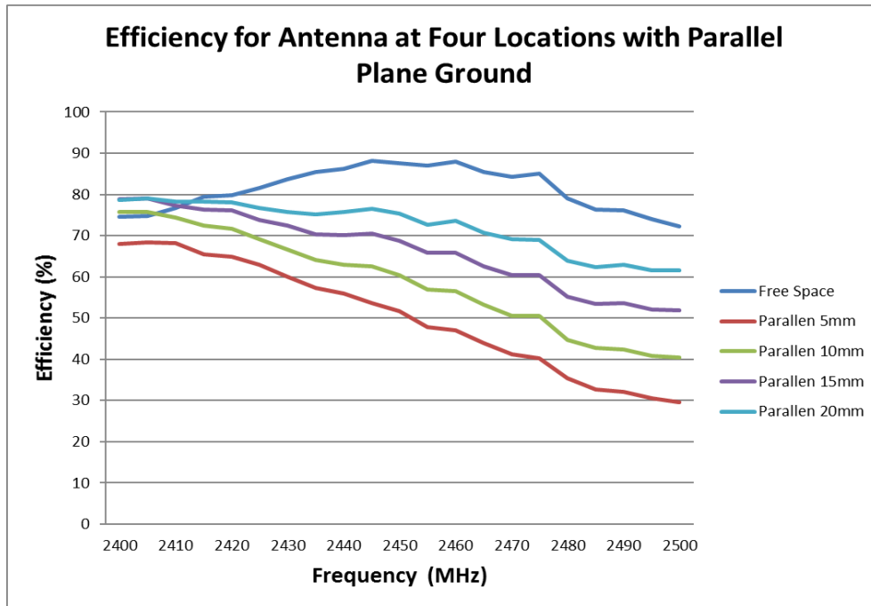
FIGURE 7.1.3 EFFICIENCY OF ANTENNA AT 2.4GHZ AT FOUR LOCATIONS WITH PARALLEL PLANE GROUND ON A REFERENCE PCB FOR CONFIGURE 1
