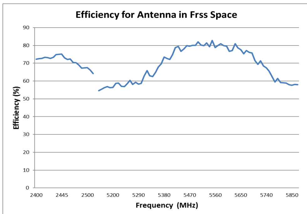
FIGURE 4.4.2 EFFICIENCY OF ANTENNA AT 2.4/5GHZ IN FREE SPACE FOR CONFIGURE 2
