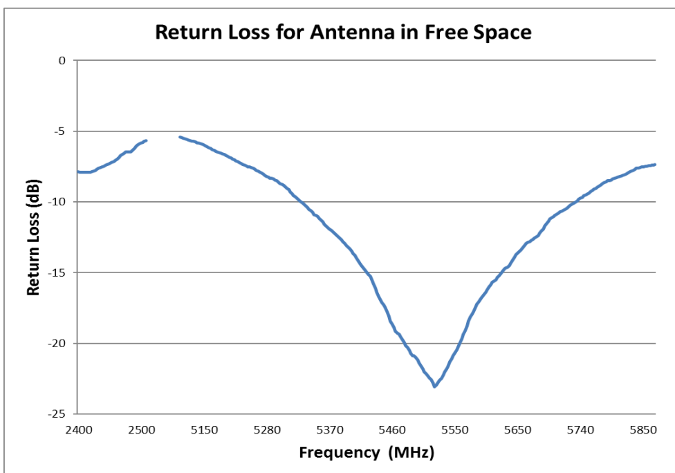
FIGURE 4.3.2 RETURN LOSS OF ANTENNA AT 2.4/5GHZ IN FREE SPACE FOR CONFIGURE 2
