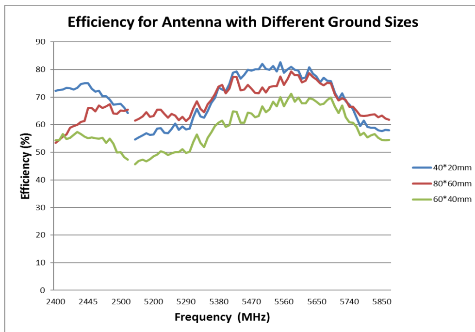
FIGURE 7.4.4 EFFICIENCY OF ANTENNA AT 2.4/5GHZ WITH DIFFERENT GROUND SIZES FOR CONFIGURE 2
