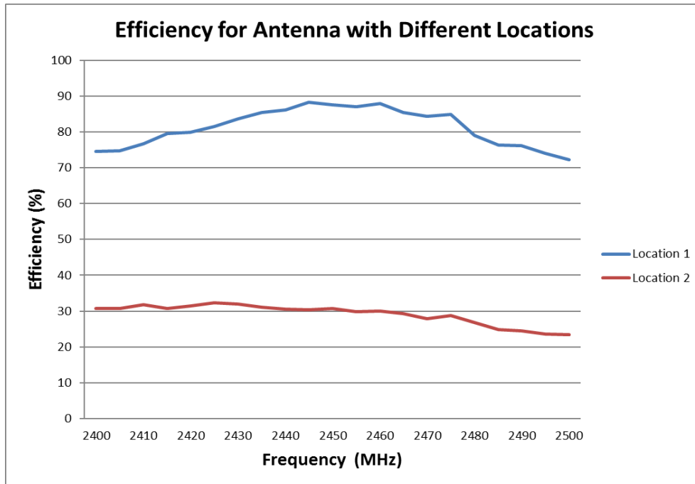
FIGURE 7.3.4 EFFICIENCY OF ANTENNA AT 2.4GHZ AT TWO DIFFERENT LOCATIONS FOR CONFIGURE 1
