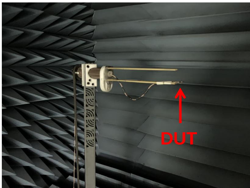
FIGURE4.1.2 ANTENNA LOADED WITH REFERENCE PCB TESTED IN OTA CHAMBER
