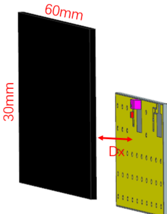
FIGURE 7.1 FOUR LOCATIONS WITH PARALLEL PLANE GROUND (USING CONFIG1 FOR ILLUSTRATION)
