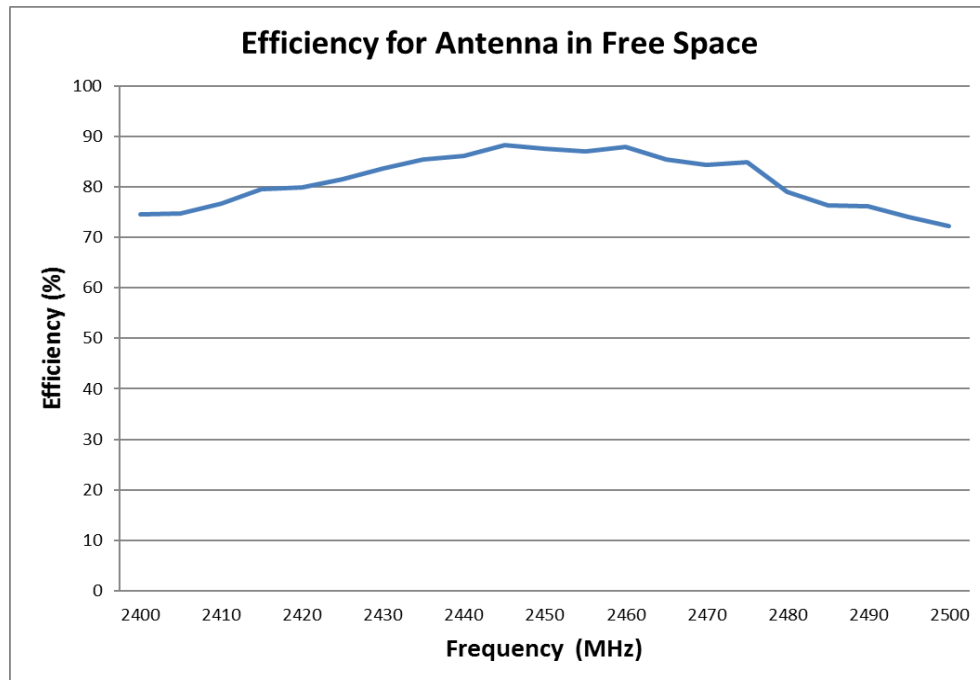
FIGURE 4.4.1 EFFICIENCY OF ANTENNA AT 2.4GHZ IN FREE SPACE FOR CONFIGURE 1
