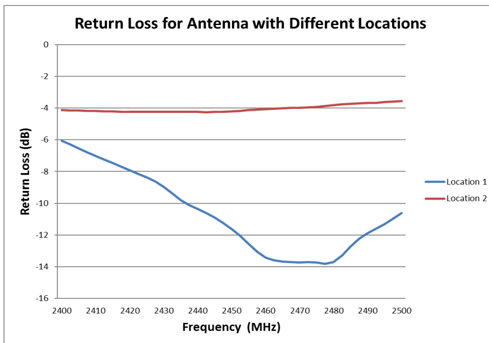
FIGURE 7.3.1 RETURN LOSS OF ANTENNA AT 2.4GHZ AT TWO DIFFERENT LOCATIONS FOR CONFIGURE 1
