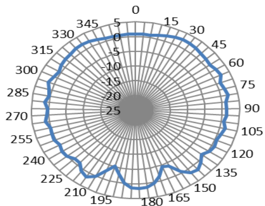
FIGURE 4.5.1 2D RADIATION PATTERN OF ANTENNA AT 2.4GHZ IN FREE SPACE FOR CONFIGURE 1
