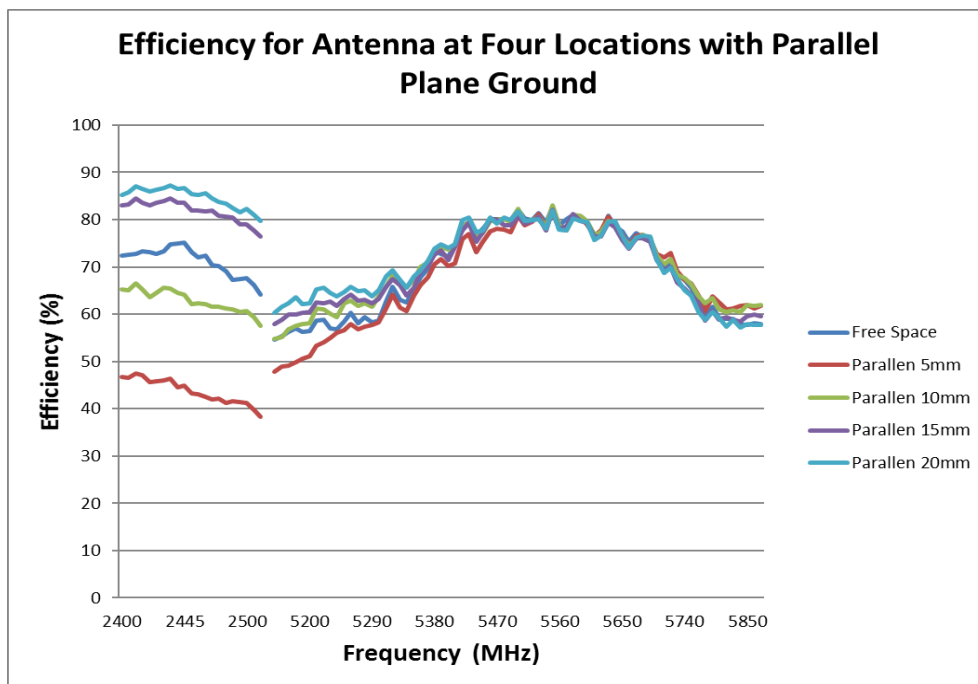
FIGURE 7.1.4 EFFICIENCY OF ANTENNA AT 2.4/5GHZ AT FOUR LOCATIONS WITH PARALLEL PLANE GROUND ON A REFERENCE PCB FOR CONFIGURE 2
