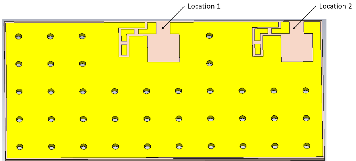
FIGURE 7.3 TWO LOCATIONS ON REFERENCE PCB FOR CONFIGURE 1 AND CONFIGURE 2(USING CONFIG1 FOR ILLUSTRATION)
