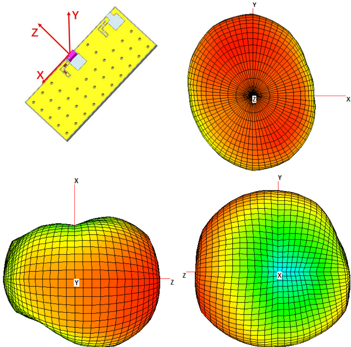
FIGURE 4.6.2 3D RADIATION PATTERN OF ANTENNA AT 2450MHZ IN FREE SPACE FOR CONFIGURE 2
