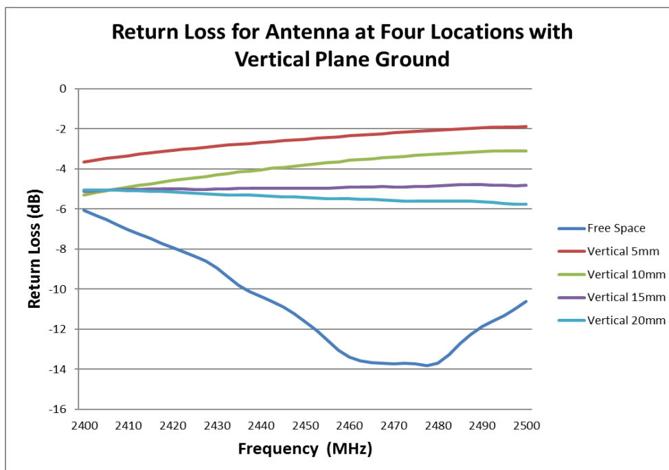
FIGURE 7.2.1 RETURN LOSS OF ANTENNA AT 2.4GHZ AT FOUR LOCATIONS WITH VERTICAL PLANE GROUND ON A REFERENCE PCB FOR CONFIGURE 1
