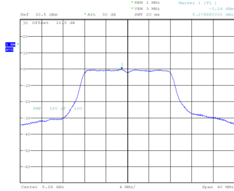
802.11a mode, 5280MHz
