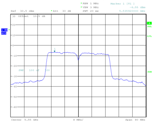
802.11n-HT40 mode, 5550MHz
