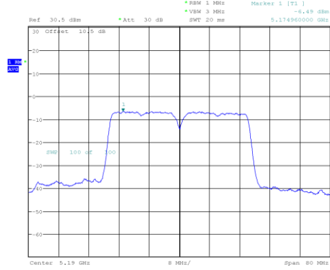
802.11n-HT40 mode, 5190MHz
