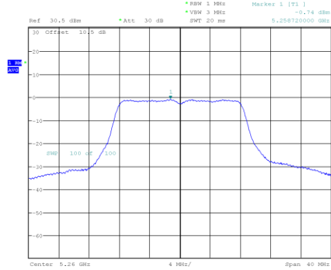
802.11a mode, 5260MHz
