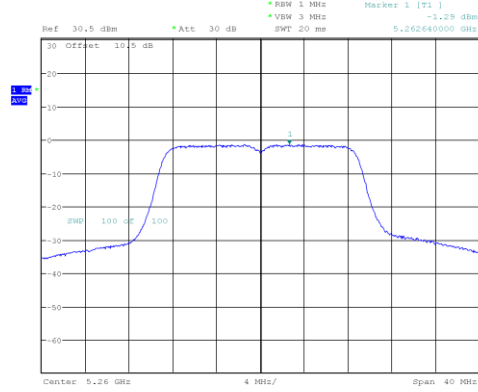
802.11n-HT20 mode, 5260MHz
