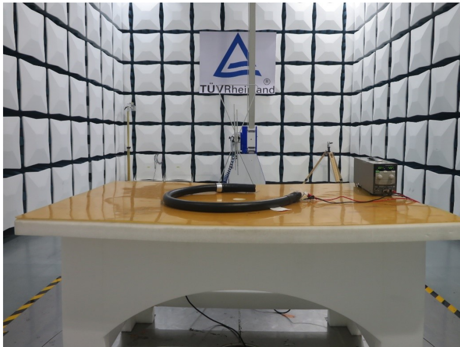
Photograph 2: Set-up for Radiated Spurious Emission, 1GHz - 3.2GHz
