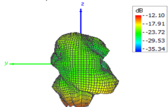
Theta = 90, Phi = 180
