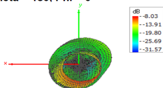
Theta = 180, Phi = 0
