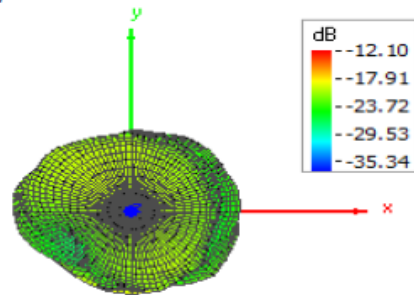
Theta = 0, Phi = 0
