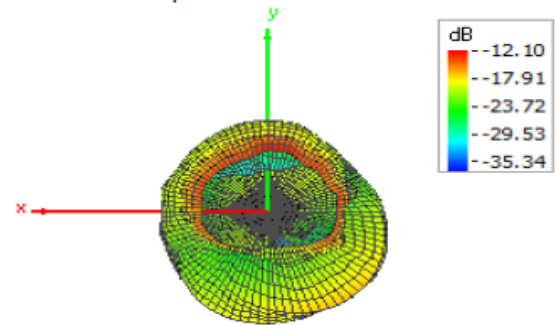
Theta = 180, Phi = 0
