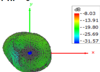
Theta = 0, Phi = 0
