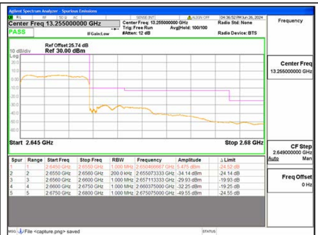
B41(2535-2655) / 10MHz / High CH / QPSK / FULL RB
