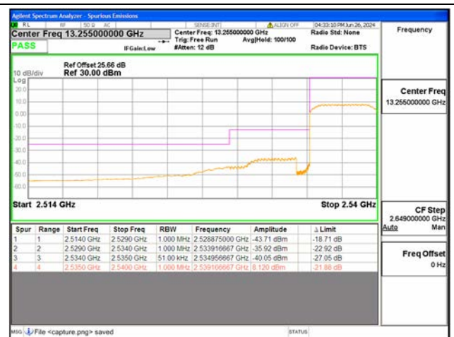
B41(2535-2655) / 5MHz / Low CH / QPSK / FULL RB
