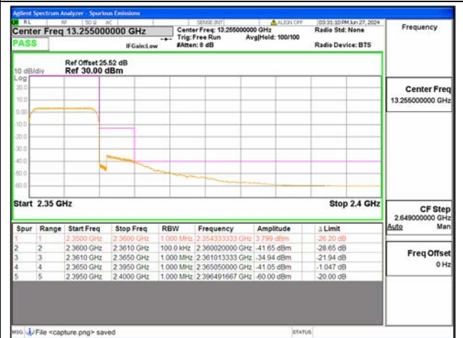
B40-2 / 10MHz / High CH / QPSK / FULL RB
