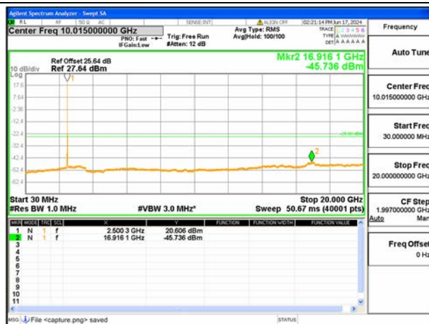
B7-30M-20G / 15MHz / Low CH / QPSK
