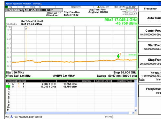
B40-1-30M-20G / 10MHz / Mid CH / QPSK
