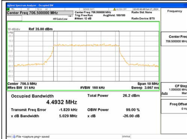
B17 / 5MHz / 64QAM/ Low CH
