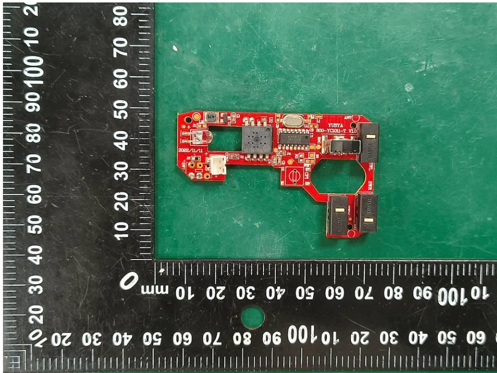
Top PCB view for model XSD-53
