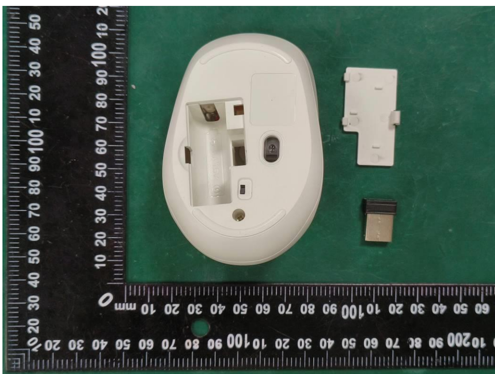
Internal view for model XSD-72
