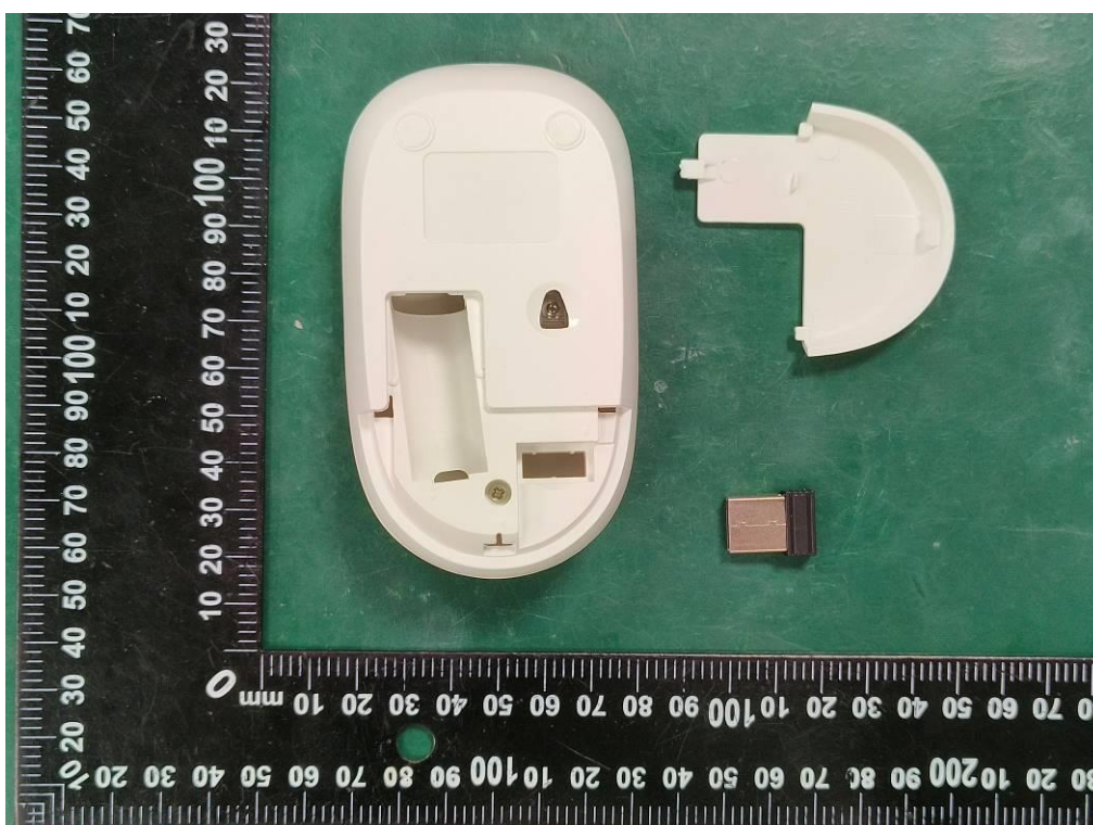
Internal view for model XSD-53
