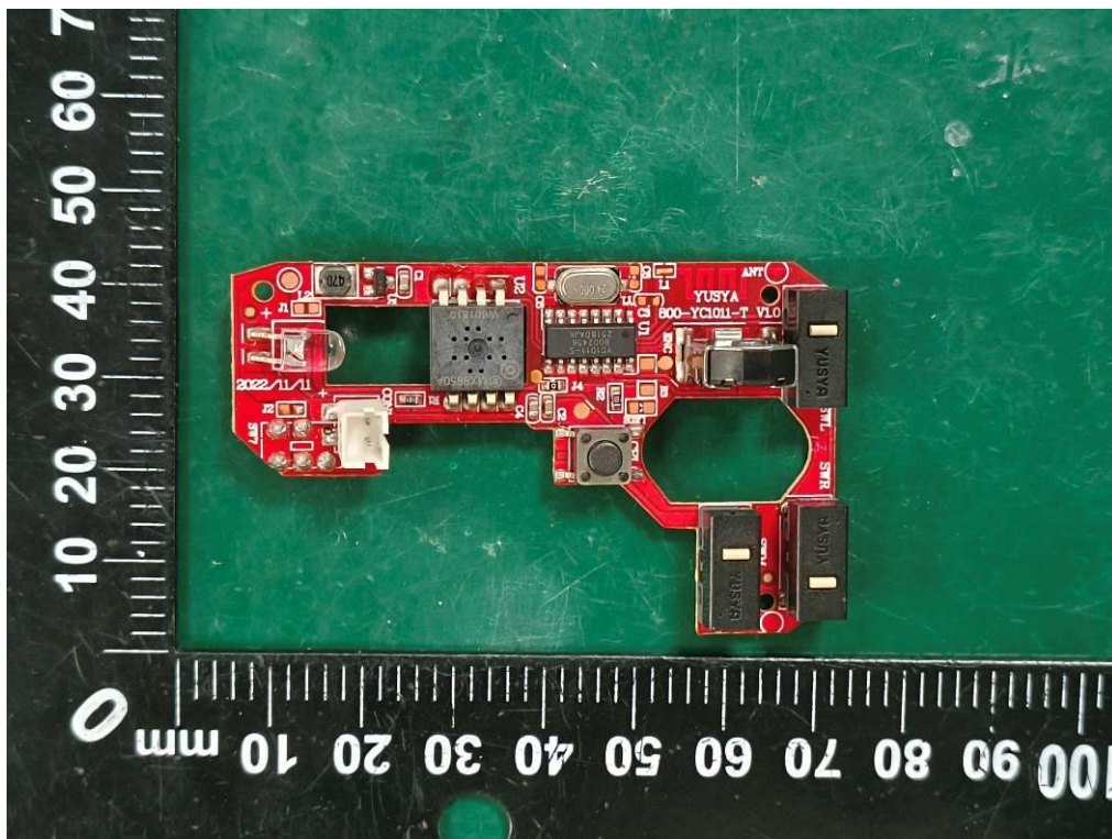
Top PCB view for model XSD-72
