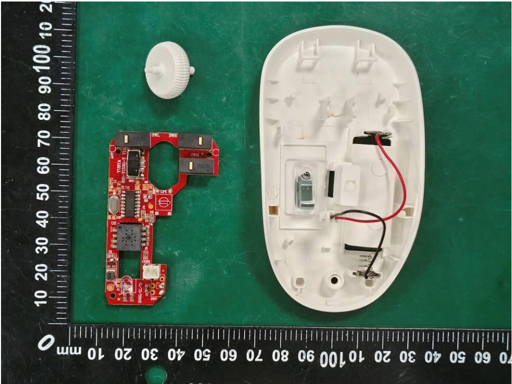
Internal view for model XSD-33
