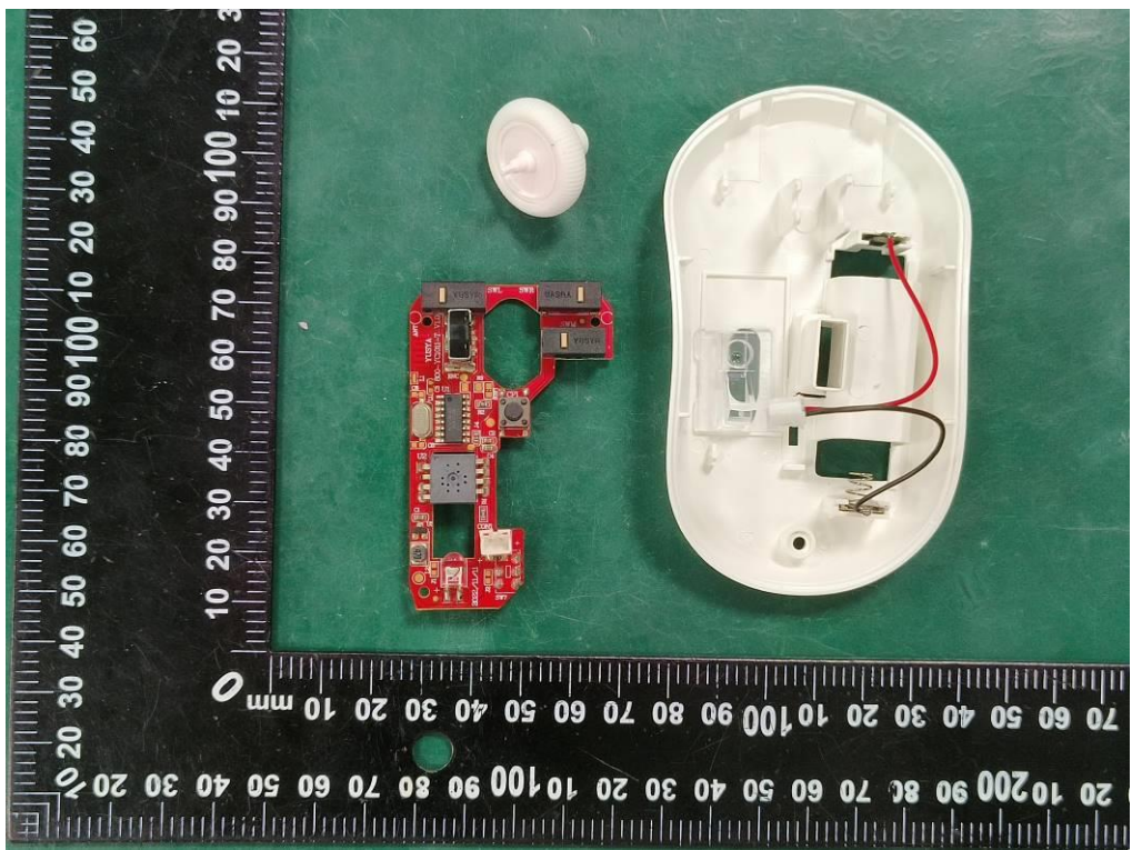
Internal view for model XSD-41
