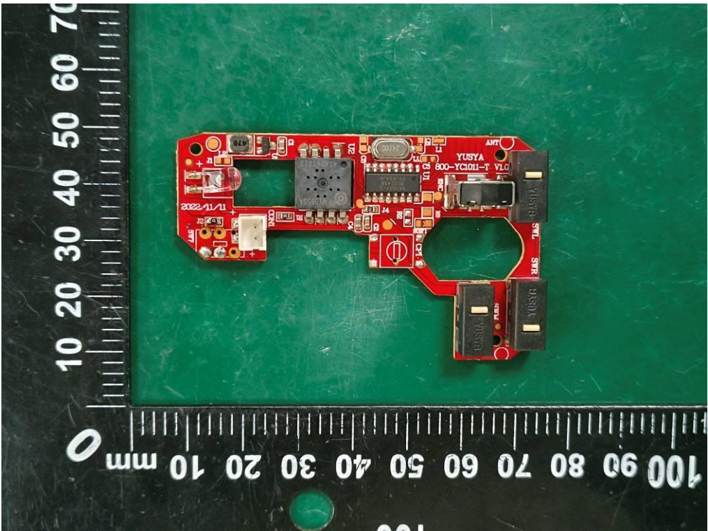
Top PCB view for model XSD-33
