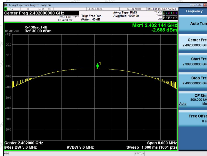
2.4G-Ant1-2402-PASS
