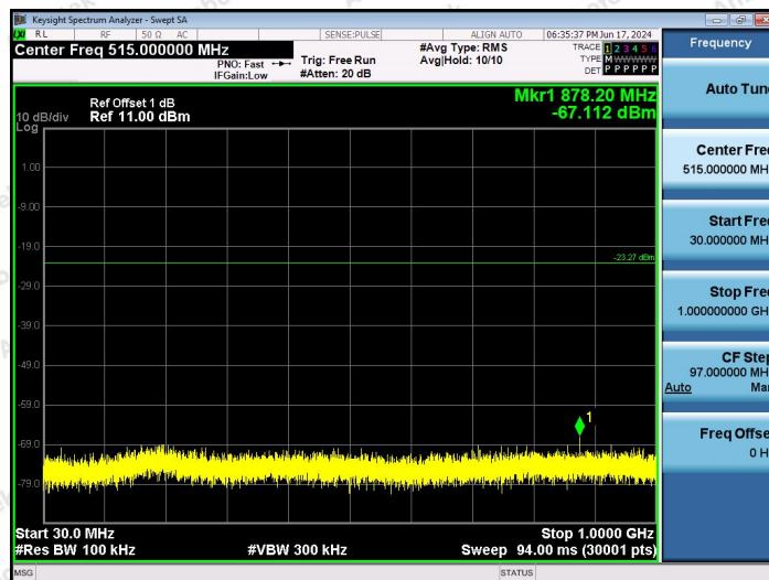
DH5-Ant1-2440-30~1000-PASS
