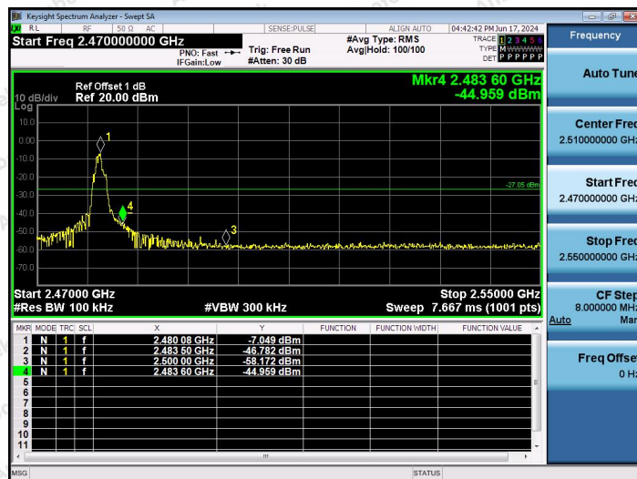
2.4G-Ant1-2480-PASS
