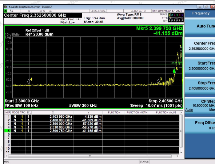
2.4G-Ant1-Hop_2402-PASS
