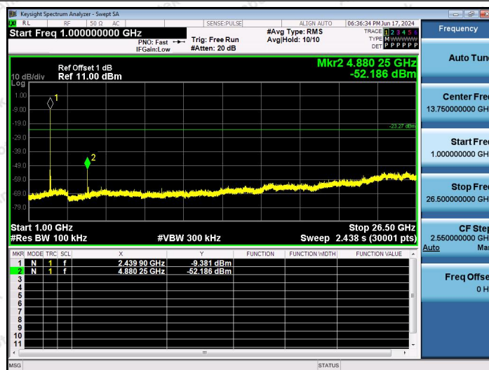
DH5-Ant1-2440-1000~26500-PASS
