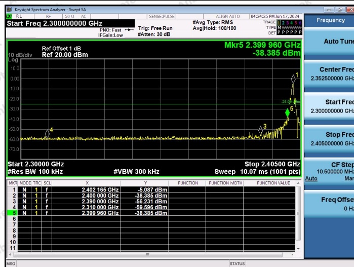
2.4G-Ant1-2402-PASS
