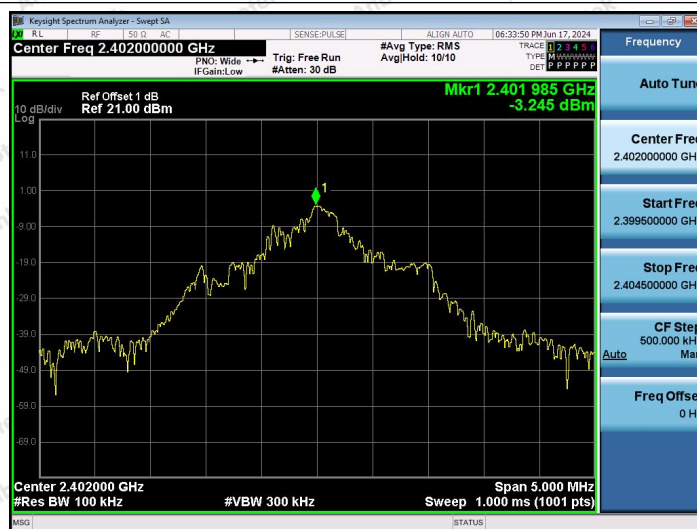
DH5-Ant1-2402-0~Reference-PASS
